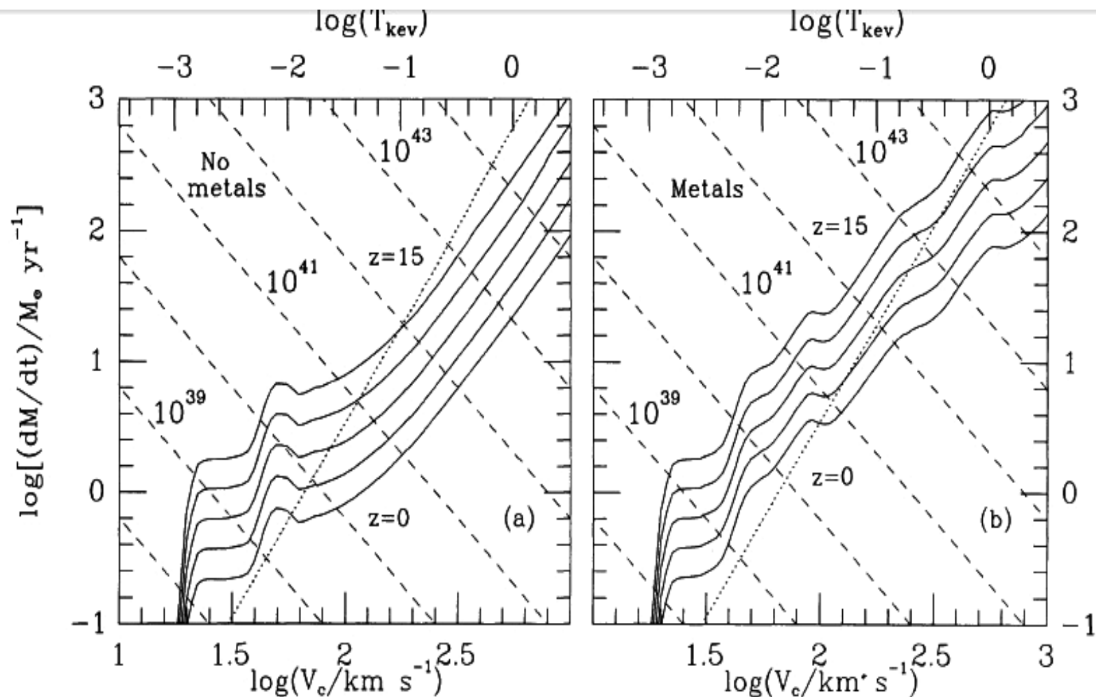
FIG. 2.—Gas infall rate and cooling rates in dark matter halos as a function of circular velocity and redshift. The infall rate ( dotted line ) is essentially independent of redshift; the cooling rates ( solid lines ) are given for redshifts z = 0, 1, 3, 7, and 15 ( from bottom to top ). Dashed lines give present-day X-ray luminosities in \text{ergs s}^{-1} produced by gas cooling at the given rate in each halo. The predicted temperature of this emission is given on the upper abscissa. (a) A cooling function for gas of zero metallicity is assumed. (b) A cooling function for gas enriched according to the models of § 4 is assumed. In both cases, \Omega_b = 0.1 and the biasing parameter b is 2.5.
