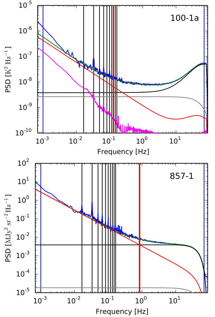
Figure 26. Two examples of the 4-component noise model fits to measured noise PSDs. The underlying noise estimation for these fits is described in Planck Collaboration XII (2015) . It measures the sample autocovariance of signal-subtracted and masked data to overcome effects of gaps and signal residuals. The blue curve is the measured PSD averaged over 30 pointing periods. The red curve is the 1/f component, deconvolved with the bolometer transfer function. The black curve is the electronic white noise component and the grey curve is the photonic white noise component. The magenta curve is the measured a/b correlated component. The green curve is the sum of all noise model components. Vertical blue lines indicate the region where the fit was made and the vertical black lines indicate the ten lowest spin harmonic frequencies.
