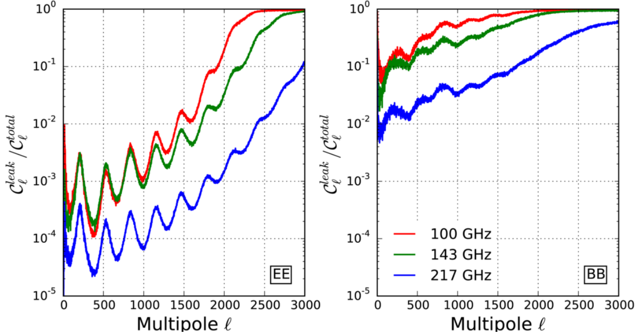
Figure 17. A simulation of the ratio of temperature-to-polarization leakage to EE and BB signal given the main beam mismatch.
