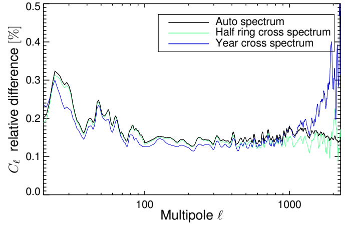
Figure 22. Relative differences of the C_\ell , computed on 60 % of the sky, using data processed with and without the nonlinearity correction of the bolometer response. The example shown here is for bolometer 217-1.
