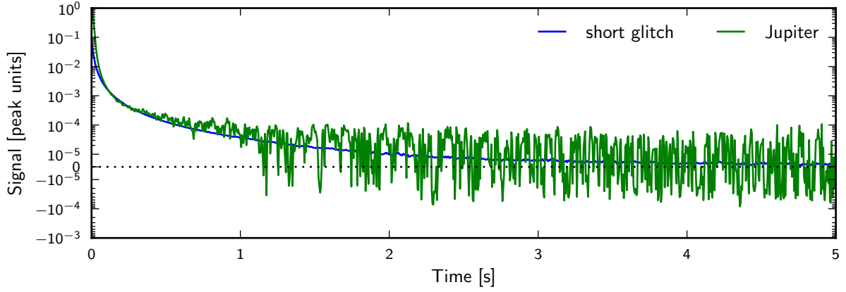
Figure 10. Impulse response of bolometer 143-6 to short glitches and to Jupiter. The plotted y-axis range is linear within the range \pm 10^{-5} and logarithmic elsewhere.
