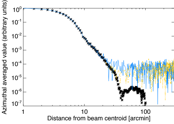
Figure B.4. Renormalization of the beam. The black stars show the beam azimuthal profile template used to renormalize the data. The pointing information of the scan is reflected through the values of the planet scan’s template since the two-dimensional scanning reference beam map is interpolated to the transit pointing before the azimuthal averaging. The renormalization convention is arbitrary, and is chosen so that the template resulting from uniform azimuthal coverage is set to the value 1 at 1’ from the beam centroid. The blue curve traces the positive data from the planet scan azimuthal average after the renormalization procedure; the yellow dashed curve shows the negative data redressed to positive values for plotting purposes. For Jupiter, only data below the conservative threshold are used in the renormalization procedure (see table B.1) to avoid biases from the finite planetary disc size and detector’s nonlinearity response effects.
