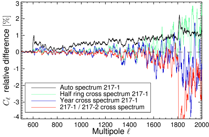
Figure 21. Relative differences of the C_\ell , computed on 60 % of the sky, using data analysed with and without removal of the 4 K line frequencies.
