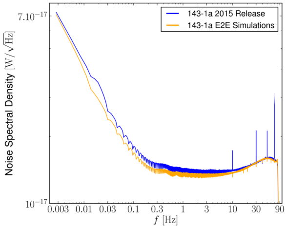
Figure 27. The PSD of the true noise for bolometer 143-1a as compared to that generated with the end-to-end simulation.
