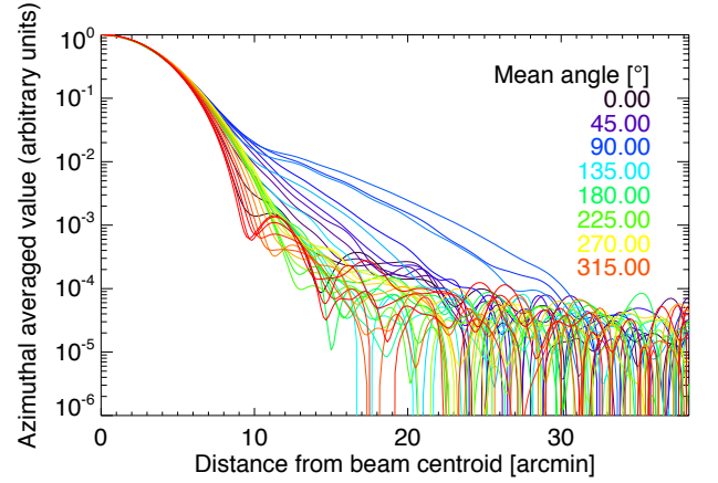
Figure B.8. The 32 radial profiles (averaged over a range of azimuthal angles) for the 143-5 beam. The azimuthal angles are defined so that 90° corresponds to the profile closest to the residual time response feature (dark blue).
