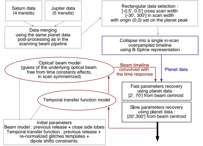
Figure C.1. Schematic diagram of the time-constant fitting process for the 353 GHz channels. The main difference from the CMB channels is the fact that the longest time constants from glitches templates that cannot be constrained by the planet signal are here renormalized so that their relative contribution is injected properly in the temporal model, and the fast part of the time response is re-evaluated to reduce the co-scan distortion and induce a beam closer to optical. This is particularly significant for PSB pairs, where a different distortion for each channel is expected without re-iterating on the fast time constants or if one does not constrain the resulting beam to be symmetric enough in the co-scan profiles where the time constants act, artificially inducing strong beam mismatches within the same horn.
