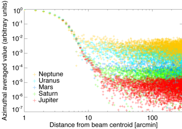
Figure B.5. Renormalized planet data (positive values). Planet scans are prepared for the merging into a single data timeline using the azimuthal profile template process. For illustration purposes, we also show Neptune and Uranus scans.
