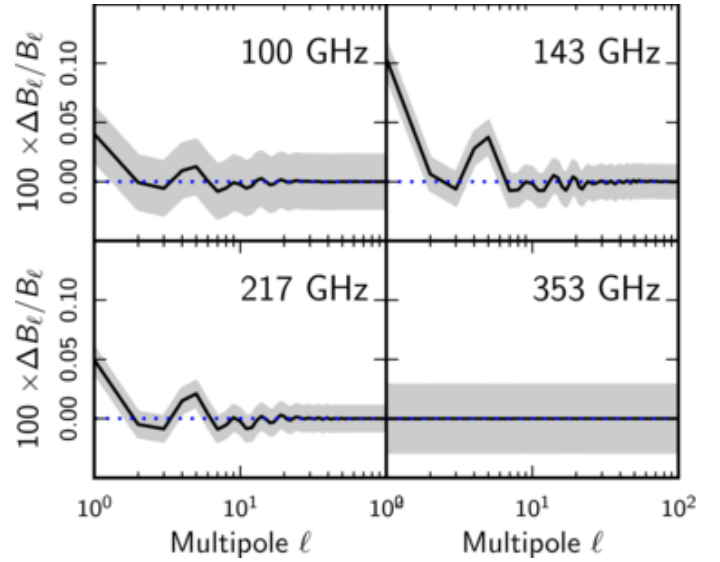
Figure 16. Estimate of the effective beam window function corrections due to far-sidelobe response (more than 5° from the beam axis). Shading indicates \pm 1\sigma errors. The curves in the 353 GHz panel are divided by a factor of 10; for this frequency the far sidelobe response amplitude is very low compared to the estimated errors.
