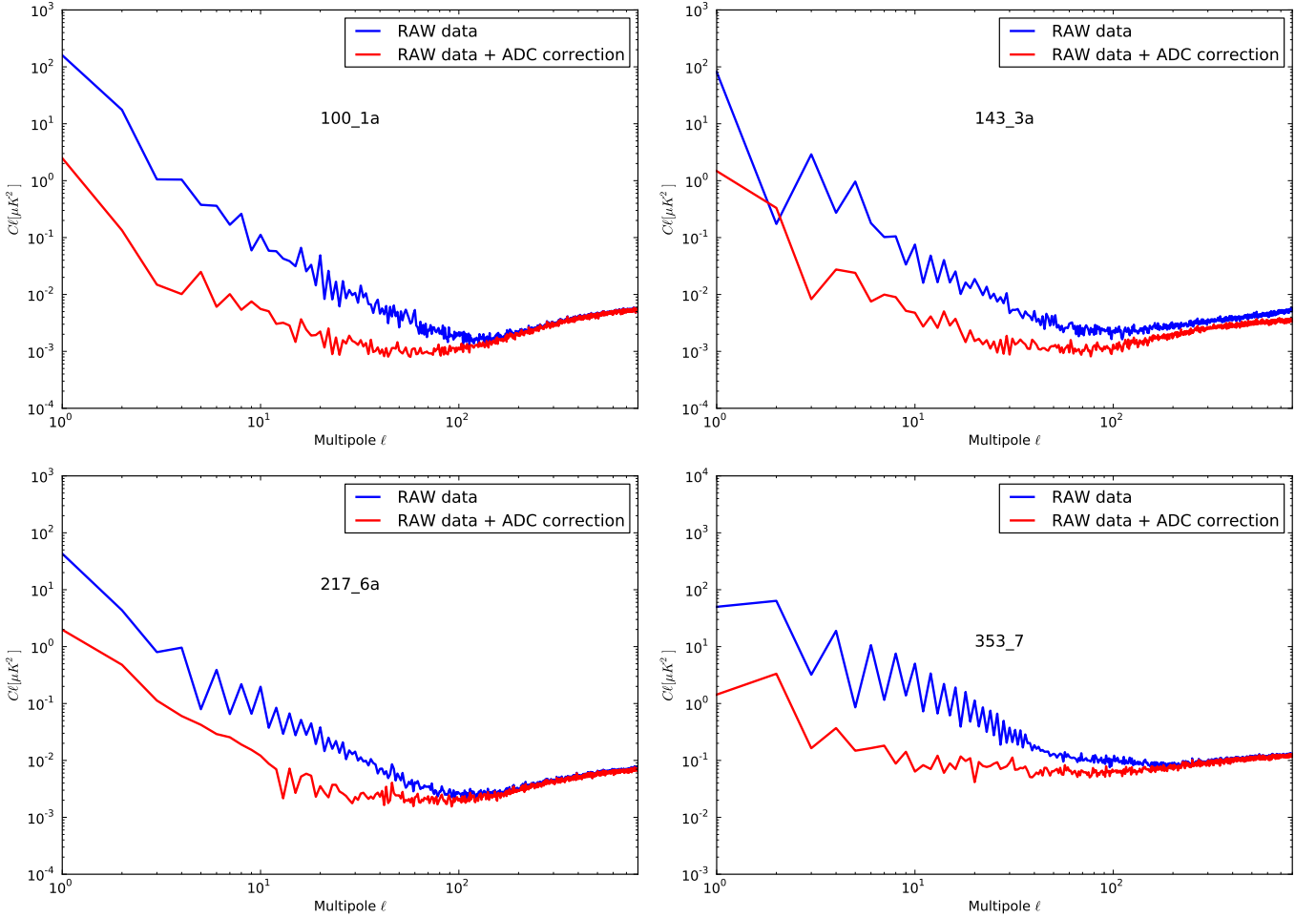
Figure 19. Half parity map difference spectra for the same bolometers as in Fig. 18. Blue : 2013 release without ADC correction. Red : the present data release with ADC correction. Below \ell = 100 the noise should be flat when there is no ADC bias.
