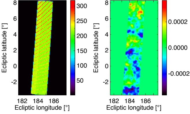
Figure B.1. The hit count map (left panel) of the corresponding background map (right panel) of the first Saturn scan, for bolometer 143-5, in K_{\text{CMB}} .
