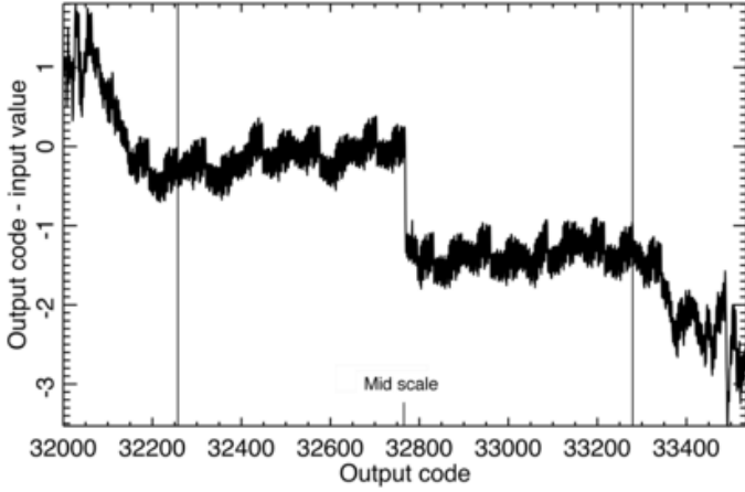
Figure 2. An example of one ADC defect mapping around the mid-scale. The useful range \pm 512 around mid-scale is shown.
