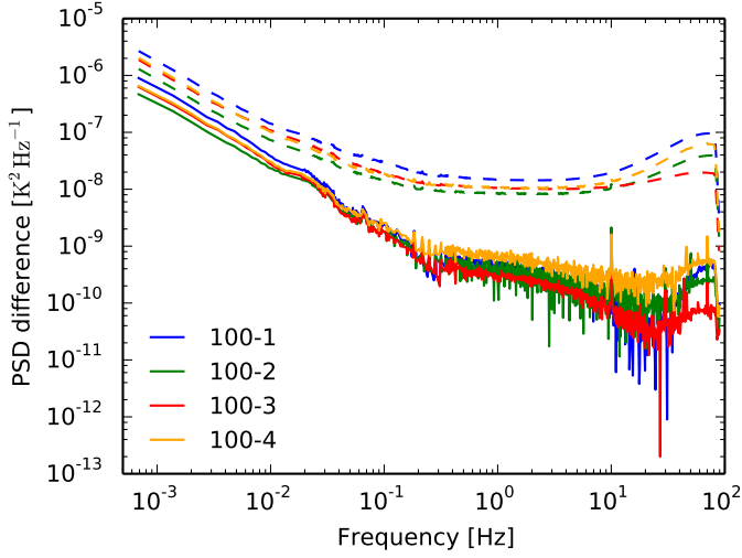
Figure 25. Example of measured summed, (a + b) , time stream noise PSDs (dashed lines) and the difference in the PSD between (a + b) and (a - b) (solid lines). These spectra are bin-by-bin median values across the entire mission and were derived by first measuring the sample autocovariance as described in Planck Collaboration XII (2015) .
