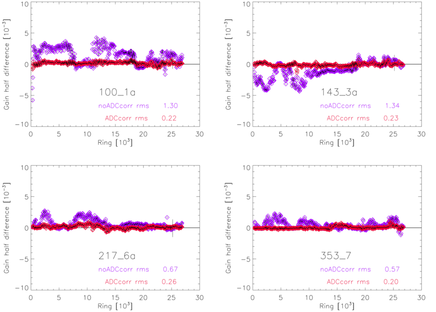
Figure 18. The relative gain difference between parity + and – samples is shown as a function of the ring number. A boxcar average by 101 rings has been applied. The purple data points were processed with the 2013 pipeline, without ADC correction, while the red points refer to the present data release with ADC correction. The median error bars are of the order of 10^{-4} for the ADC-corrected TOI.
