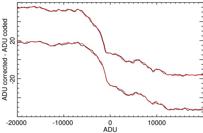
Figure 5. Example ADC correction functions for both parities (upper and lower curve sets) and two different phases (in black and red) relative to the 4K cooler cycle.
