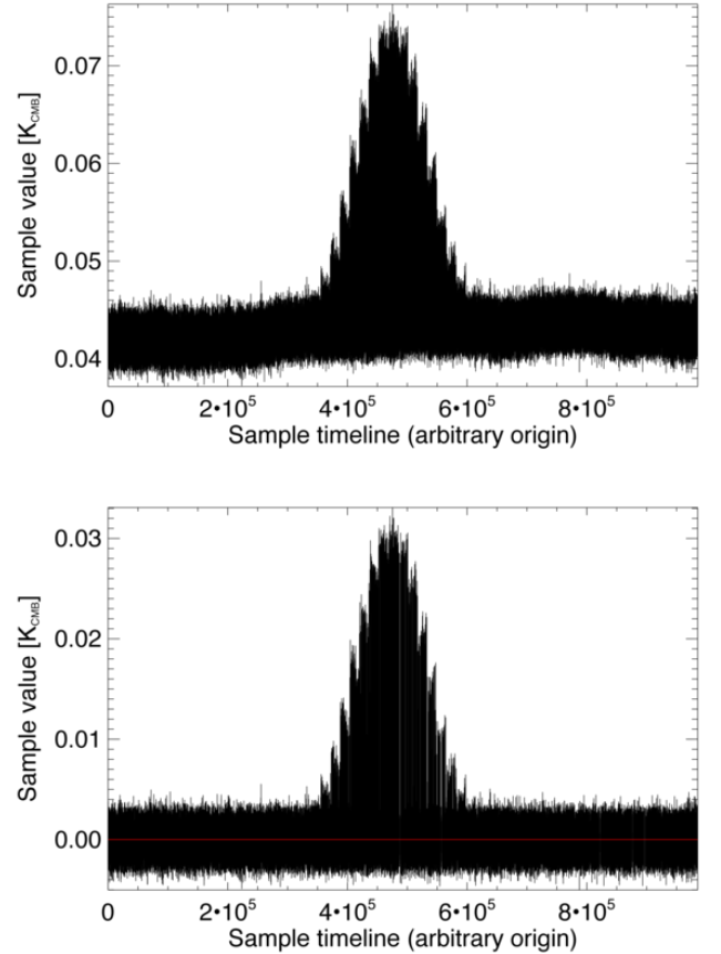
Figure B.3. The TOI for bolometer 100-3b and the first scan of Mars, shown both before (upper panel) and after (lower panel) subtraction of the baseline (Fig. B.2).
