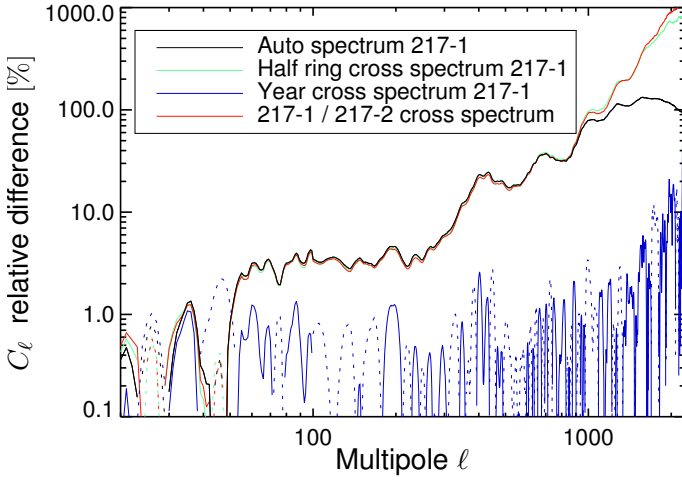
Figure 20. Relative differences of the C_\ell , computed on 60 % of the sky, using data processed with and without the thermal decorrelation. Note that the zero-level has been recomputed in all cases to allow the comparison. The amplitudes of the negative values are shown by dotted lines.
