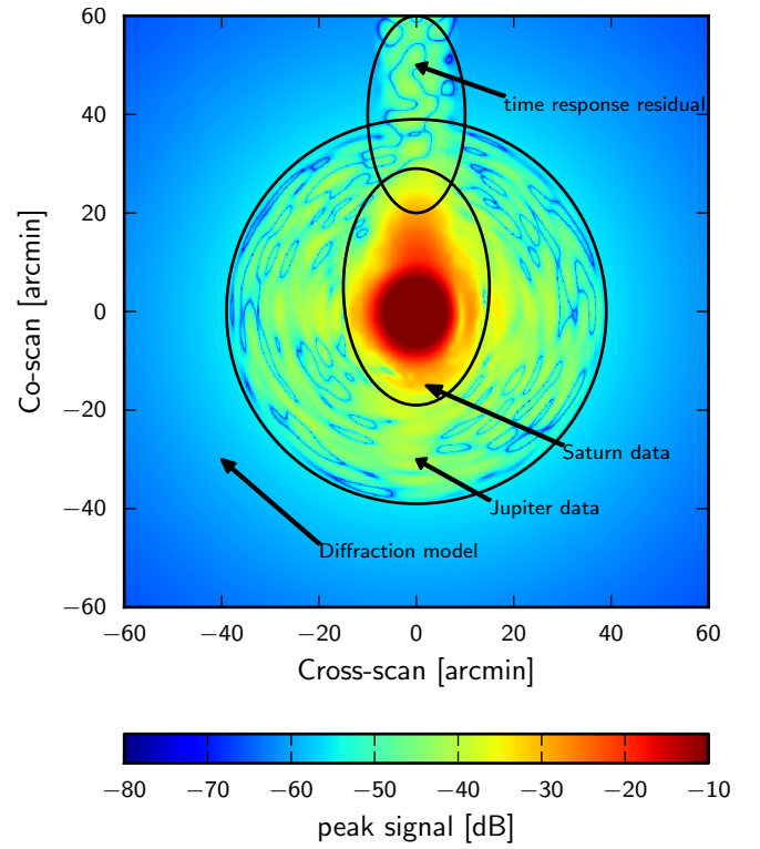
Figure 12. Scanning beam map for detector 143-6 showing a rough diagram of the regions that are handled with a different data selection or binning.
