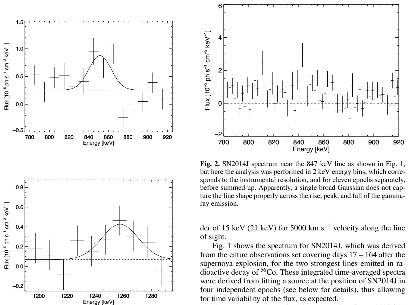
Fig. 1. SN2014J spectrum near the 847 keV line ( above ) and near the 1238 keV line ( below ) as expected from ^{56}\text{Co} decay. These spectra are determined in energy bins of width 10 keV over the entire observing period; the source intensity is fitted at four independent epochs. For illustration, fitted Gaussians indicate the detection of broadened lines near the ^{56}\text{Co} gamma-ray line energies.
