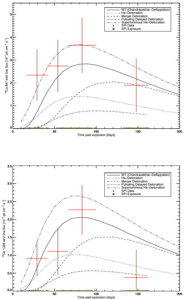
Fig. 4. SN2014J signal intensity variations for the 847 keV line ( above ) and the 1238 keV line ( below ) as seen in our observations and shown in Fig. 3. Here the intensity was derived by Gaussians fitted to the spectra near the respective ^{56}\text{Co} line at four independent epochs, as discussed in the text. The epochs are shown as horizontal bars at each data point. For reference, several candidate model light curves are shown, as extracted from The & Burrows (2014).
