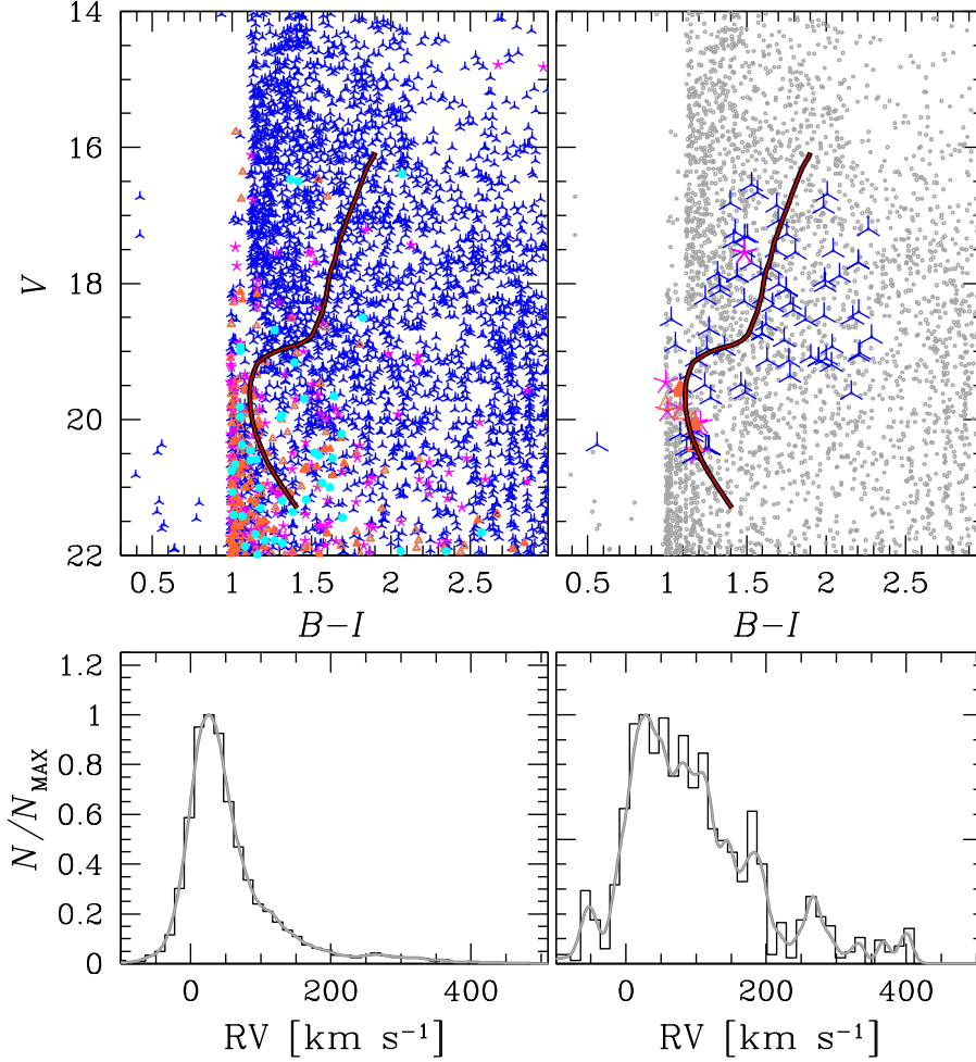
Figure 4. Left panels: V versus (B-I) CMD predicted by the Galactic model by Robin et al. (2003) for all the stars in a 60' \times 60' field of view centered at the same coordinates as the field studied in this paper (top). We used the same symbols introduced in Fig. 3 to represent stars in different radial-velocity intervals. The histogram and the kernel-density distribution of radial velocities predicted by the Galactic model for the same stars are shown in the lower-left panel. Right panels: In gray we represent the same CMD of the upper-left panel; stars that have V and (B-I) similar to the observed stars, belonging to the “equivalent sample” (see Sect. 3.2 for details) have been represented according with symbols and colours corresponding to their radial velocity (see Fig. 3).
