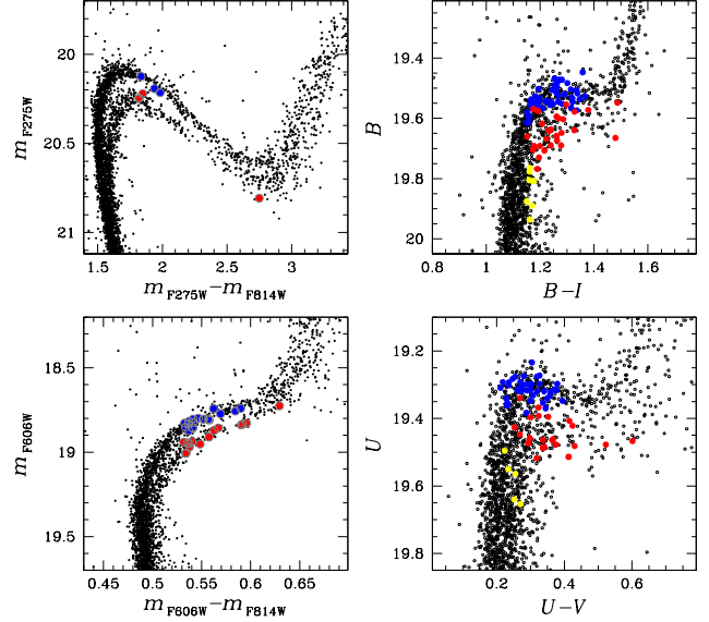
Figure 9. Distribution of the inner field spectroscopic targets on the m_{\text{F275W}} - (m_{\text{F275W}} - m_{\text{F814W}}) (from Piotto et al. 2012), m_{\text{F606W}} - (m_{\text{F606W}} - m_{\text{F814W}}) (from Milone et al. 2008), B - (B - I) , and U - (U - V) CMDs (Milone et al. 2009). Stars assigned to the bSGB and fSGB have been represented in blue and red, respectively, stars with more uncertain location respect to the double SGB have been coloured in yellow.
