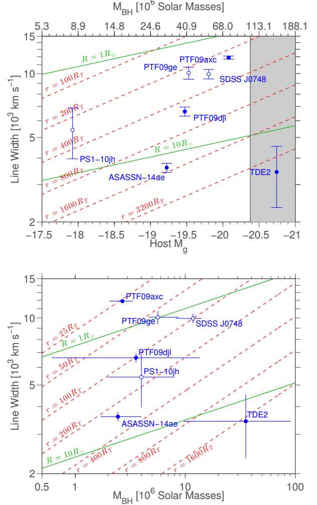
Figure 17. TDE-candidate line widths of H (filled circles) and He (empty circles) emission lines vs. host galaxy K-corrected g -band absolute magnitudes (top) and SED-derived SMBH masses (bottom). The dashed red lines represent the expected velocity correlations for bound material at different radii (assuming a sun-like star). The solid green lines are the Strubbe & Quataert (2009) velocities for the most energetic outflowing material assuming R_P = R_T for a sun-like star or red giant as noted. For the top panel, we use the Bernardi et al. (2003) coefficients for the Faber-Jackson relation to derive these lines and to derive the top x-axis values from the host galaxy g -band absolute magnitudes. For the bottom panel, the SMBH masses are taken from Table 6 (i.e. calculated using the Gadotti (2009) and Häring & Rix (2004) relations from our derived host stellar masses). The shaded region in the top panel denotes SMBH masses above 10^8 M_\odot , for which a TDE is not expected to be observed (assuming a sun-like star and a non-rotating SMBH).
