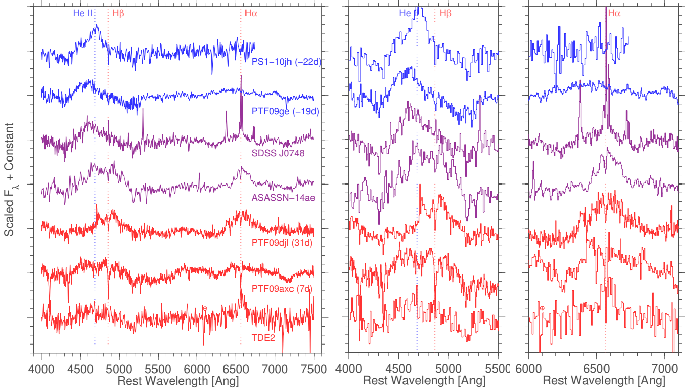
Figure 14. Continuum-subtracted spectra of our three PTF TDE candidates together with PS1-10jh (G12), ASASSN-14ae, SDSS J0748 (Wang et al. 2011) and TDE2 (van Velzen et al. 2011). Phases are shown relative to peak. A progression from He-rich to H-rich events is apparent. The middle and right panels present more detailed views of the regions around the marked lines.
