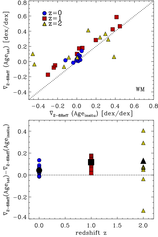
Figure 7. Top panel: Fitted age gradients (at 2 < R/R_{\text{eff}} < 6 ) of the total stellar component versus those of the in-situ stellar component at z = 0, 1 , and 2 (differently coloured symbols) for ten massive galaxies for the WM model. The black dotted line indicates equal total and in-situ gradients. Bottom panel: Difference between the total and in-situ age gradients versus redshift. On average, the total gradient is typically by 0.05 - 0.1 dex higher than the in-situ gradient in the wind model (see black symbols in the bottom panel).
