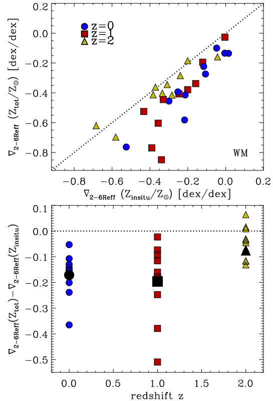
Figure 5. Top panel: Fitted metallicity gradient (at 2 < R/R_{\text{eff}} < 6 ) of the total stellar component versus the in-situ stellar component only at z = 0, 1 , and 2 (differently coloured symbols) for the WM model. The black dotted line indicates equal gradients. Bottom panel: Difference between total and in-situ metallicity gradient versus redshift. At z = 2 the total gradients are similar to those of the in-situ stellar component, whereas towards lower redshifts, the total gradient is typically by \sim 0.2 dex lower than the in-situ gradient. Large filled symbols indicate the mean.
