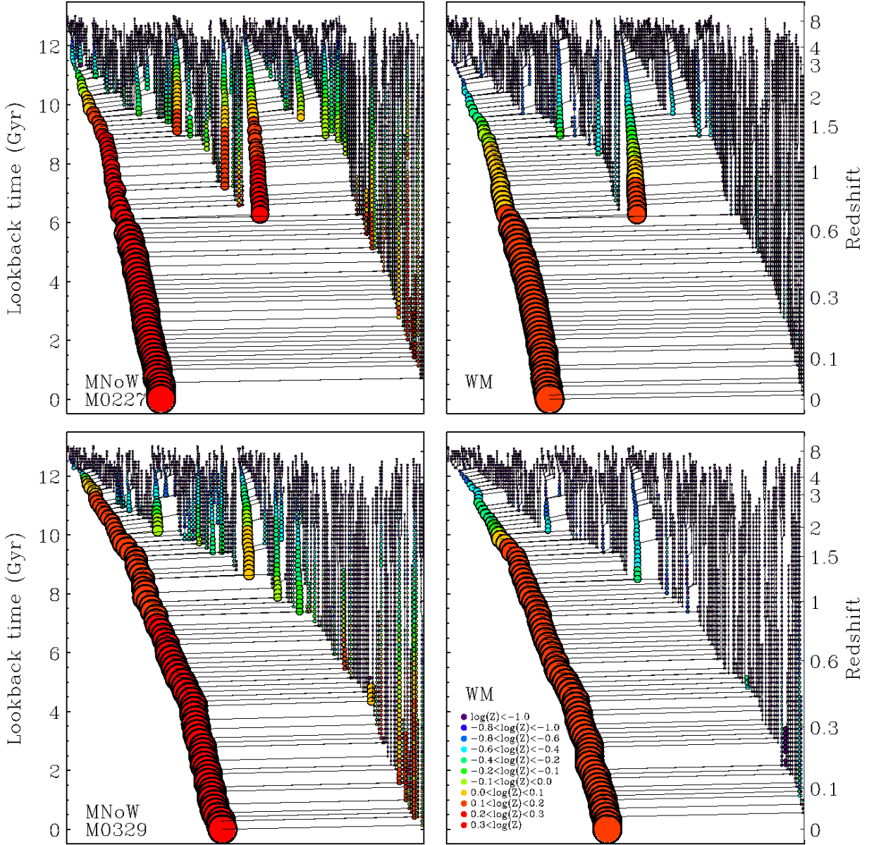
Figure 1. Halo-based merger trees for the two example galaxies M0227 (top panels) and M0329 (bottom panels) for the model without winds (MNoW, left column) and with winds (WM, right column). The size of the circles is scaled to the mass of the central galaxy in the respective halos, the colour is coded by the metallicity of the stellar component from blue (low metallicity) to red (high metallicity). In the no wind models (MNoW, left panels) the satellite halos host more massive galaxies with more metal rich stellar components, in particular at low redshifts. M0227 has a major merger with galaxy of comparable metallicity at z \sim 0.7 , whereas M0329 grows by minor mergers alone. The infalling systems are particularly metal poor in the wind simulations (WM, bottom right panel). Not all galaxies of the halos indicated here merge with the central galaxy by z = 0 (see Fig. 2).
