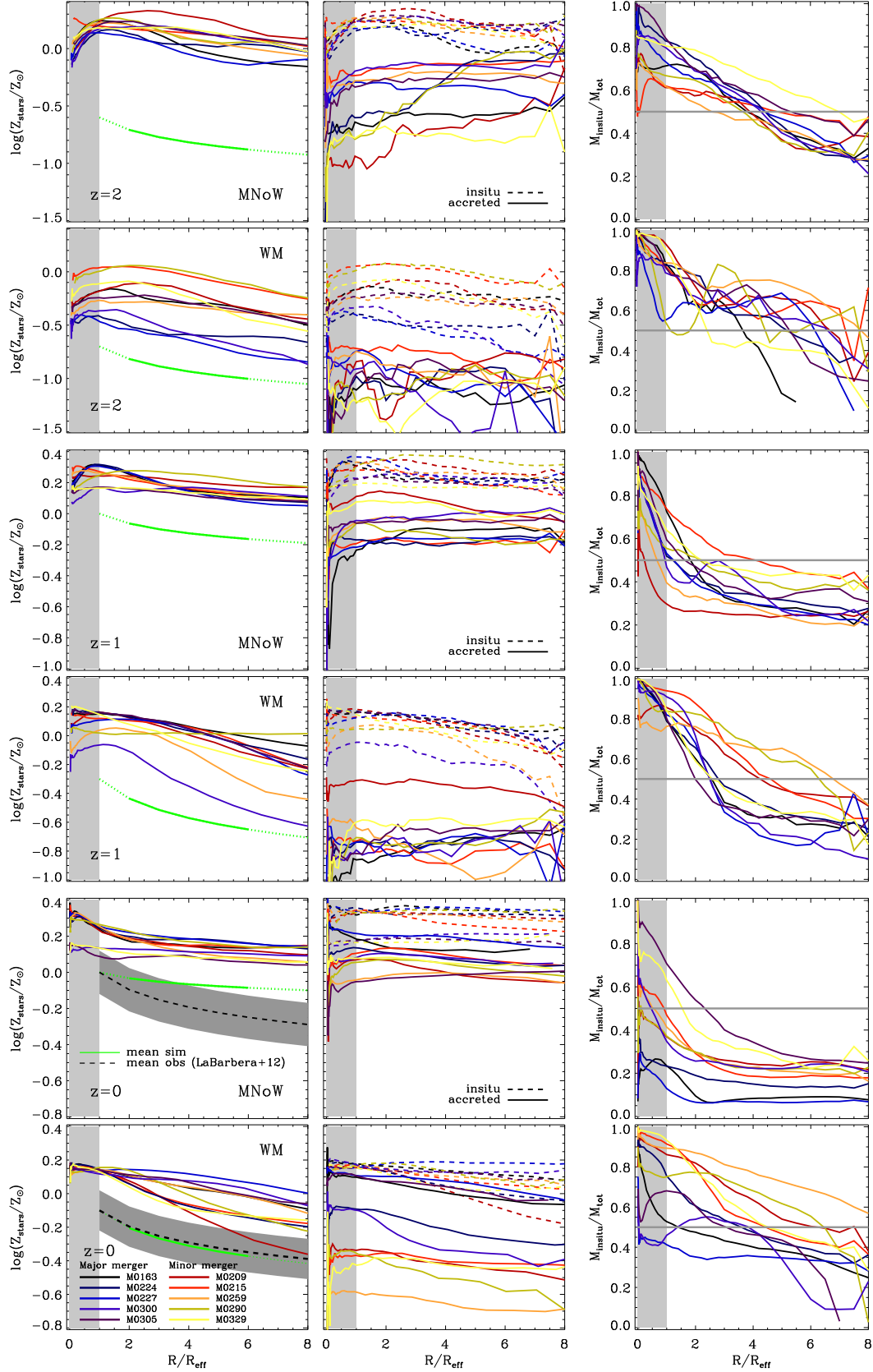
Figure 4. Left column: Total stellar metallicity gradients (mass weighted) at z=2, 1, 0 for the ten main galaxies (different colours) simulated with the MNoW and WM model. The green solid lines indicate the average gradient at 2 < R/R_{\text{eff}} < 6 . Middle panels: Metallicity gradients at z=2, 1, 0 separated into stars formed in-situ (dashed lines) and accreted stars (solid lines) for the ten main galaxies (different colours) simulated with the MNoW and WM model. Right panels: Fraction of in-situ to total stellar mass as a function of radius at z=2, 1, 0 . The grey shaded in all panels indicate the inner regions ( R/R_{\text{eff}} < 1 ) which will be most likely affected by missing AGN feedback.
