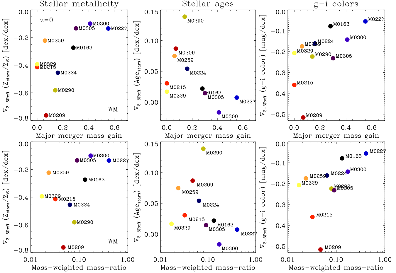
Figure 10. Left panels: Stellar metallicity gradients (between 2 - 6R_{\text{eff}} ) versus the mass gain through major mergers (top panel) and versus the mass-weighted merger mass-ratio (bottom panels) for the ten re-simulated galaxies in the WM simulations at z = 0 . The points are colour-coded according to their past major mergers as in Fig. 4. The higher the major merger mass gain or the mass-weighted mass-ratio, the smaller is the slope of the metallicity gradient. Middle panels: The same as in the left panels, but for stellar age at z = 0 . The higher the major merger mass gain, the flatter are the age gradients. Right panels: The same as in the left panels but for g-i colours at z = 0 . The higher the major merger mass gain or the mass-weighted mass-ratio, the smaller is the slope of the colour gradient. This trend is entirely driven by the negative metallicity gradients.
