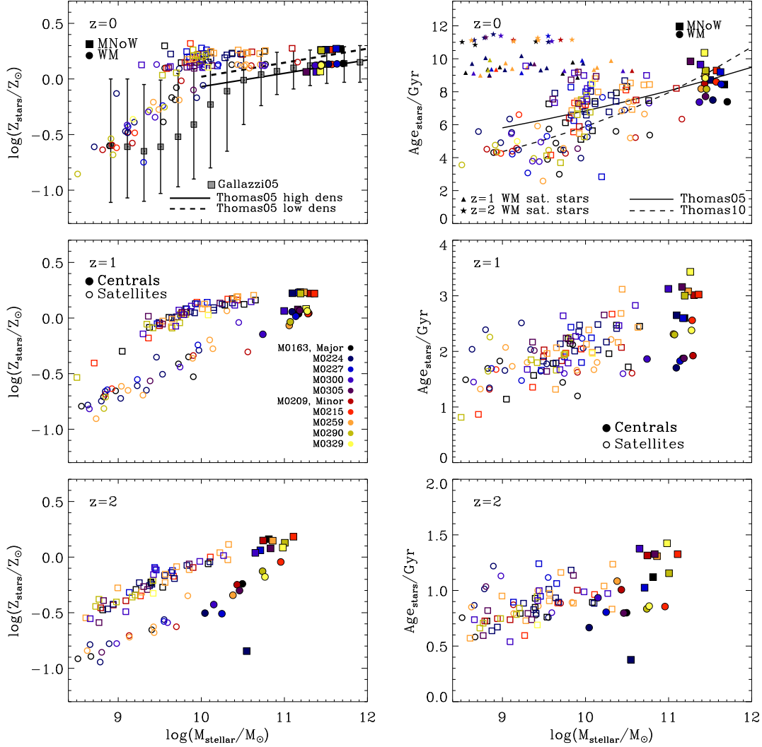
Figure 3. Left column: Mean stellar metallicity as a function of galaxy stellar mass at z = 0, 1 and 2 (from top to bottom) for ten massive galaxies (different colours) simulated with the MNoW model (filled squares) and the WM model (filled circles). The satellite galaxies residing in the respective galaxy halos (same colours) are indicated by open symbols. At all redshifts, the satellite galaxies in the wind model (WM) have significantly lower metallicities than those simulated without winds (MNoW). For this model the z = 0 metallicities agree with observational estimates (Thomas et al. 2005, black lines; Gallazzi et al. 2005, grey squares). Right column: Mean stellar age as a function of galaxy mass at z = 0, 1 and 2 (from top to bottom) for the ten galaxies and their satellites as in the left column. Compared to observations (Thomas et al. 2005, 2010), the central galaxies in the WM model are slightly too young by roughly 2 Gyrs. For the WM model, the small filled triangles and stars indicate the hypothetical present-day ages of the satellites at z = 1 and z = 2 , most of them have merged with the central galaxies until z = 0 .
