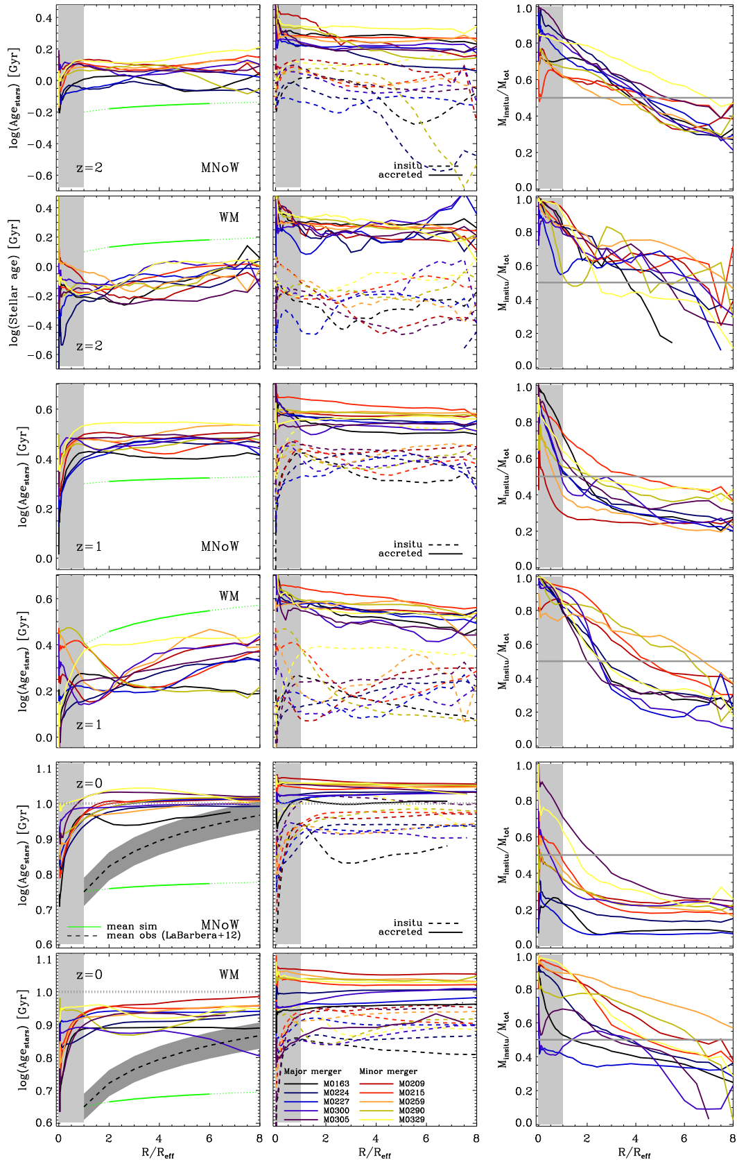
Figure 6. Same as Fig. 4, but now for stellar age gradients at z = 2, 1, 0 (from top to bottom) for the ten galaxies in the MNoW and WM models.
