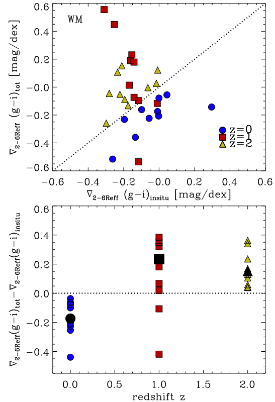
Figure 9. Fitted g-i colour gradients (at 2 < R/R_{\text{eff}} < 6 ) of the total stellar component versus the ones of the in-situ stellar component at z = 0, 1 , and 2 (differently coloured symbols) for the ten massive galaxies in the WM model. The black dotted line indicates equal total and in-situ gradients.
