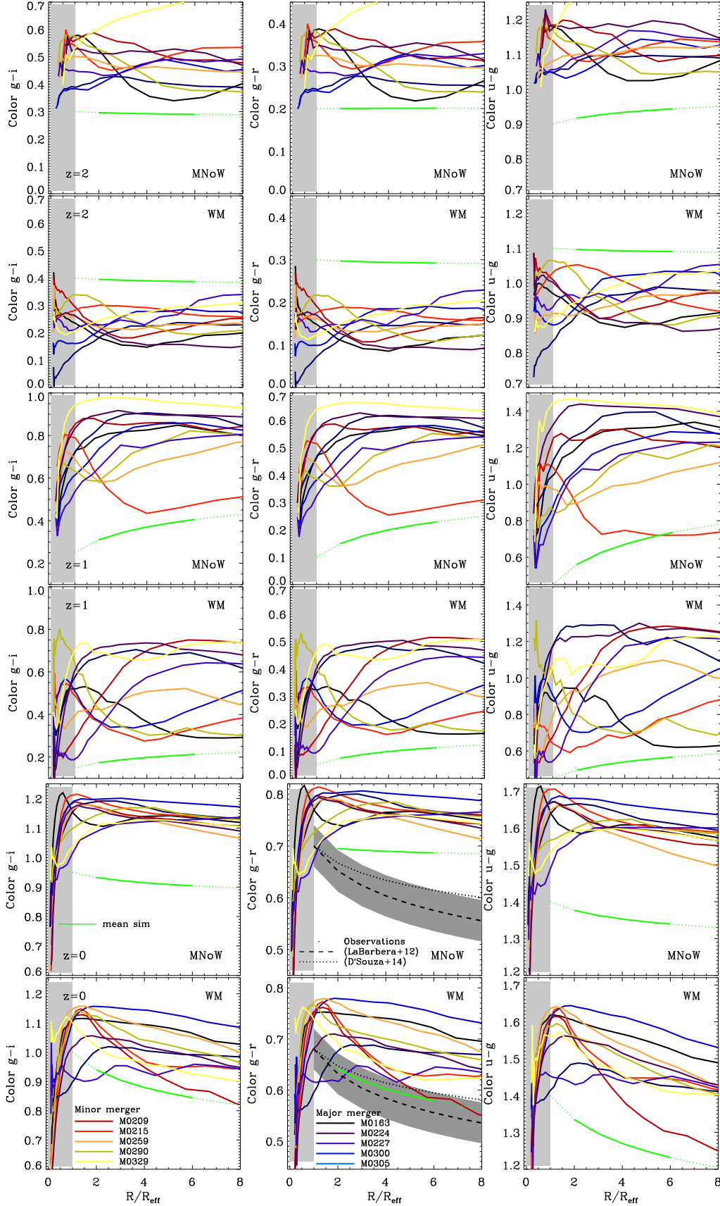
Figure 8. Colour gradients ( g-i , g-r , and u-g , from left to right) at z = 2, 1, 0 (from top to bottom) for the ten galaxies (different colours) in the MNoW and WM models. Galaxies with major mergers since z = 2 are indicated by black-blue colours (those have typically the flattest colour gradients at z = 0 ), while galaxies with only minor mergers since z = 2 are illustrated by red-yellow colors (having steeper gradients). At r > 2R_{\text{eff}} , present-day WM galaxies show negative colour gradients in the outer parts, which are steeper than for the MNoW galaxies.
