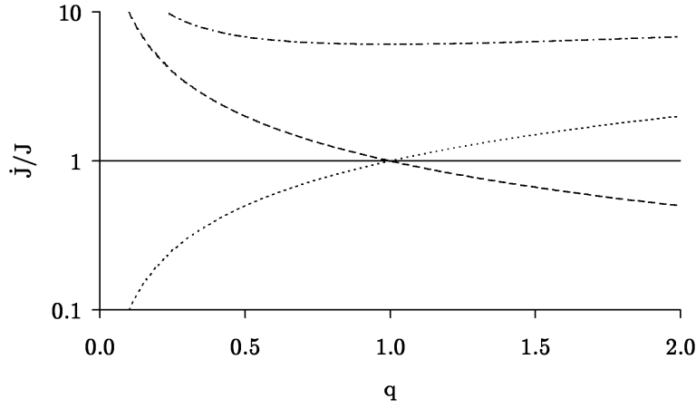
Fig. C.1. Angular momentum loss (in terms of \frac{\dot{M}(1-\beta)}{M_d + M_a} ) as a function of mass ratio for four modes: specific angular momentum loss mode (solid, for \eta = 1 ), Jeans mode (dotted), isotropic re-emission mode (dashed) and in the case of a circumbinary ring (dashed-dotted, for a_{\text{ring}}/a = 2.3 ). See text for definition and explication of modes.
