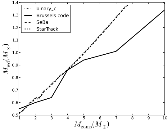
Fig. 7. Initial-final mass relation of single stars that become WDs for the different groups, dotted line shows the results of binary_c, solid line the results of the Brussels code, the dashed line the results of SeBa, and the dash-dotted line the results of StarTrack.
