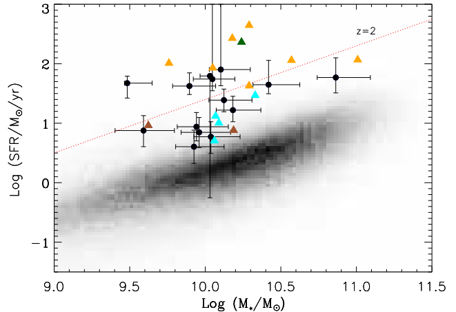
Fig. 1.— High- z sample (colored symbols; see the left panel in Figure 3 for definition of different colours) and the median values of the low- z samples (black circles) in the M_* – SFR plane are shown where main-sequence star-forming SDSS galaxies are shown as a 2D histogram. Error bars shown on the black circles indicate 1 \sigma scatter in the low- z sample of each high- z galaxy. The fit to the main-sequence z \sim 2 star-forming galaxies (Elbaz et al. 2011) is shown by a dashed red line.
