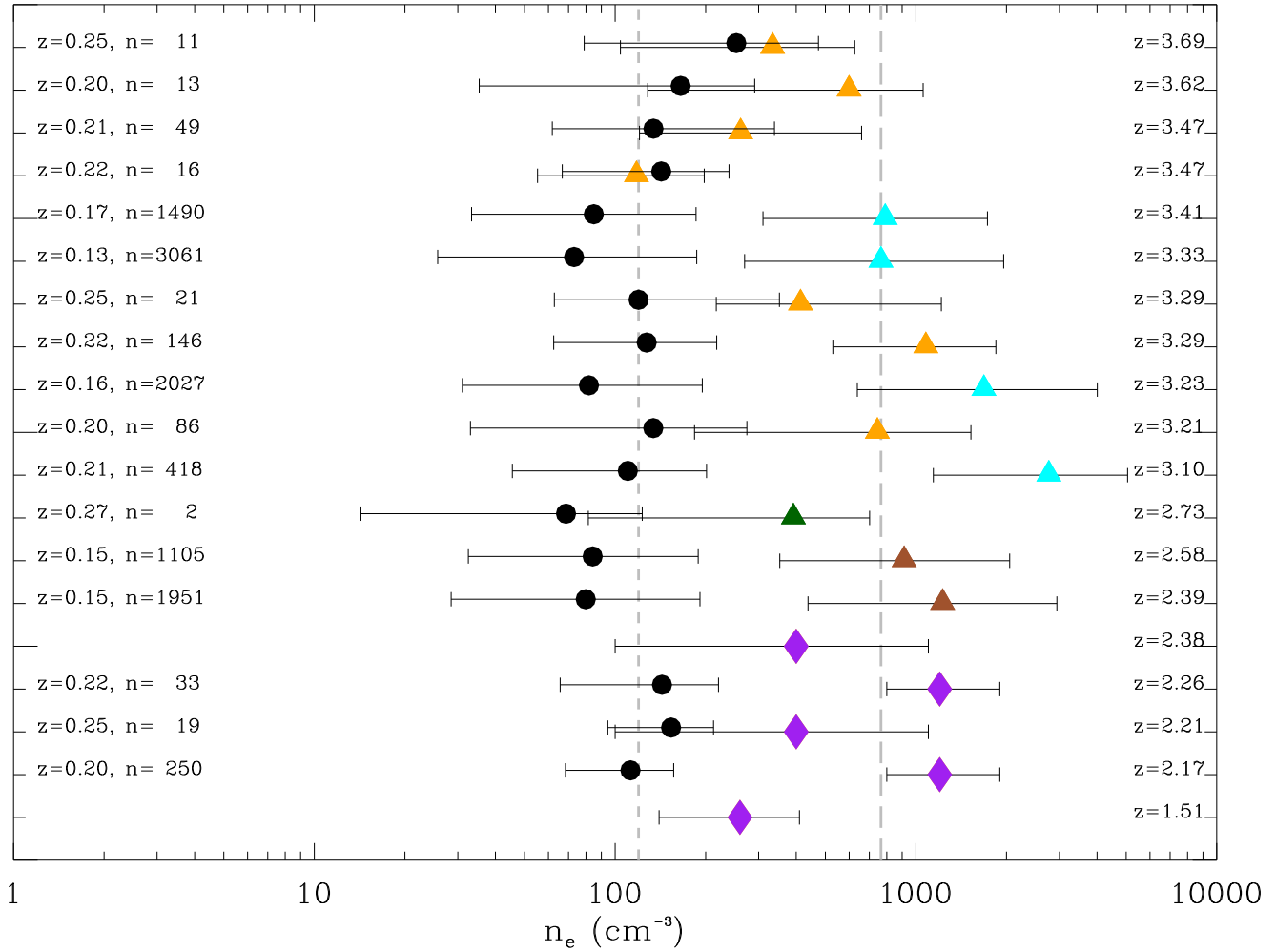
Fig. 4.— Median value of the electron density for the low- z samples inferred from the [S II] 6716, 6731 doublet is shown by the black filled circles. The high- z values are inferred from the low- z values multiplying by n_e(z)/n_e(z=0) ratios shown in Figure 3. Colored symbols show our high- z sample sorted based on their redshifts from bottom to top as indicated in the figure. Five galaxies from the SINS survey that have directly measured electron densities are shown by purple diamonds. The median values of the redshifts of low- z samples are shown in black and the number of low- z analogs in each sample are indicated with n . Error bars span from the 16% to the 84% confidence level (low- z data; they show scatter in the sample, high- z data; they show propagation of uncertainties through Equation 4). The grey small-dashed and long-dashed lines show the median value for the electron density at low- z and high- z , respectively.
