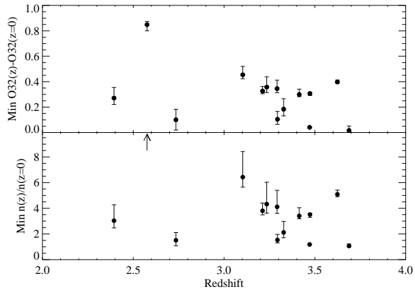
Fig. 5.— Top panel: the minimum difference in O32 between the high- and low- z samples when corrected for metallicity as described in the text. Bottom panel: the resulting minimum density difference between the high- and low- z samples when corrected for metallicity.
