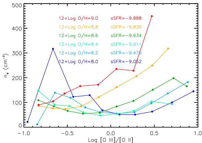
Fig. 6.— Correlation between the metallicity and gas density and O32 in star-forming galaxies in the SDSS that have measured gas density using the [S II] doublet is shown. We bin the data in gas-phase metallicity ( 12 + \log \text{O}/\text{H} = 8 to 9 ) as derived in Tremonti et al. (2004). The figure illustrates quite clearly that at fixed metallicity, an increase in O32 corresponds to an increase in the electron density.
