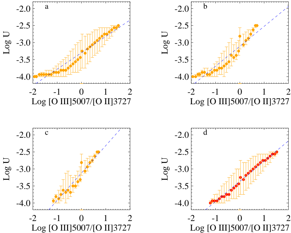
Fig. 2.— Best fit relations between ionization parameters and the [\text{O III}] \lambda 5007/[\text{O II}] \lambda 3727 (O32) ratios are shown by blue dashed lines. The top left panel shows the best fit using all CL01 models ( 0.01 < \tau_V < 4 ), the top right panel shows the best fit using only models with \tau_V \sim 0.2 , the bottom left panel shows the best fit using only models with \tau_V \sim 0.2 and \xi \sim 0.3 (i.e., Galactic dust-to-metal ratio), and the bottom right panel shows the best fit to all models with \xi \sim 0.3 . The results in the paper are presented for the fit shown in the bottom right panel.
