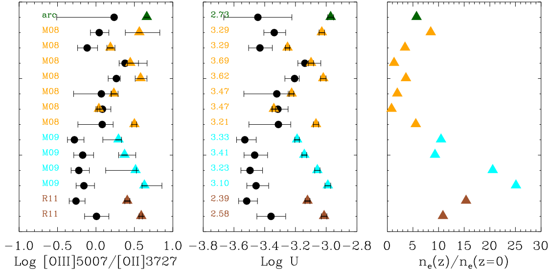
Fig. 3.— Comparison between [\text{O III}] \lambda 5007/[\text{O II}] \lambda 3727 ratio, ionization parameter, and electron density at low- z and high- z . The x axis of the left panel shows the [\text{O III}] \lambda 5007/[\text{O II}] \lambda 3727 ratio, the middle panel shows the ionization parameter, and the right panel shows the electron density at high- z relative to that of low- z . Colored symbols show high- z galaxies with their redshift indicated and black circles show the median values for the low- z sample of each high- z galaxy. Error bars span from the 16% to the 84% confidence level. We see that high- z galaxies show higher [\text{O III}] \lambda 5007/[\text{O II}] \lambda 3727 ratios than their low- z analogs (up to \approx 0.8 dex higher), even though their masses and sSFR are the same. The middle panel shows the ionization parameters derived using our new calibration between the [\text{O III}] \lambda 5007/[\text{O II}] \lambda 3727 ratio and the ionization parameter. We see that high- z galaxies show up to \sim 0.5 dex higher (median \sim 0.3 dex) ionization parameters than their low- z analogs. This translates to up to 25 times higher electron density for high- z galaxies relative to their low- z analogs.
