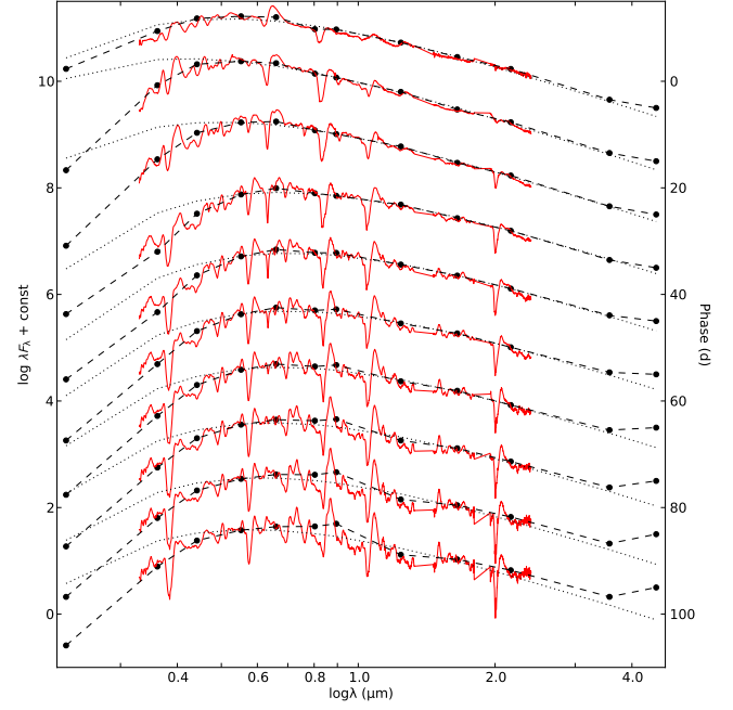
Fig. 10. The evolution of the SED as calculated with the photometric method (black dots and dashed lines) overplotted with the blackbody fits discussed in Sect. 3.2 (black dotted lines) as well as the observed spectra interpolated as described in Sect. 2.3.2 (red solid lines).
