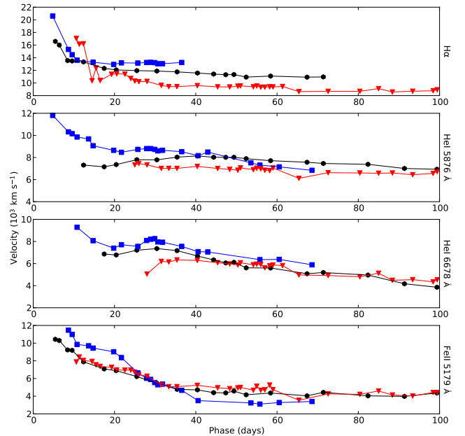
Fig. 19. Velocity evolution of the absorption minimum for the H \alpha (upper panel), He I 5876 Å (upper middle panel), He I 6678 Å (lower middle panel) and Fe II 5179 Å (lower panel) lines for SNe 2011dh (black circles), 2008ax (blue squares) and 1993J (red triangles) measured as described in Sect. 3.4.
