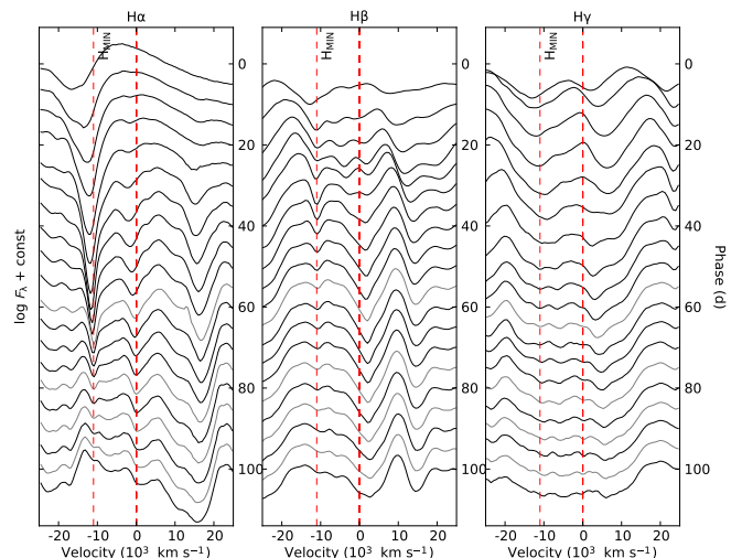
Fig. 12. Closeup of (interpolated) spectral evolution centred on the H \alpha (left panel), H \beta (middle panel) and H \gamma (right panel) lines. All panels in this and the following figure show the minimum velocity for the H \alpha absorption minimum (marked H _{\text{MIN}} ) interpreted as the interface between the helium core and hydrogen envelope.
