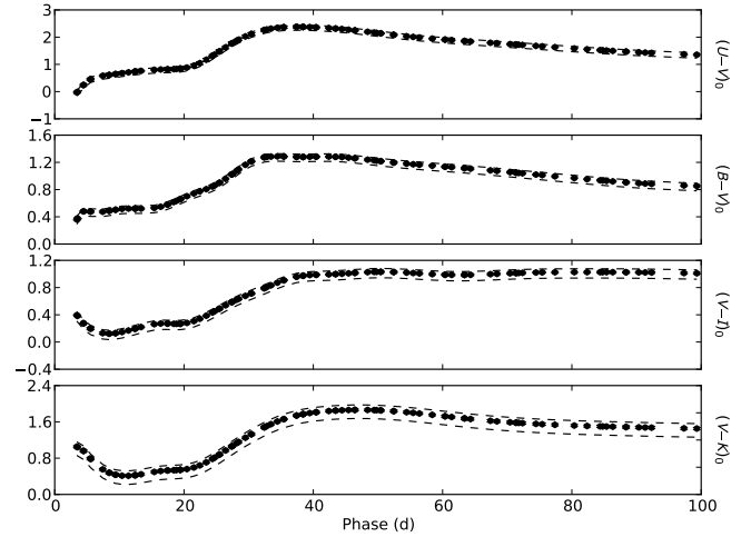
Fig. 4. U-V , B-V , V-I and V-K intrinsic colour evolution for SN 2011dh for the adopted extinction (black dots). The upper and lower error bars for the systematic error arising from extinction (black dashed lines) are also shown.
