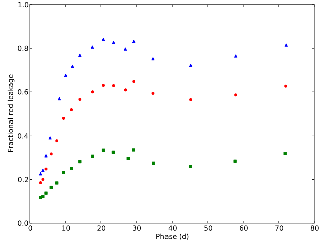
Fig. A.6. Fractional red leakage in the SWIFT UVW1 (red circles), UVM2 (green squares) and UVW2 (blue triangles) filters.
