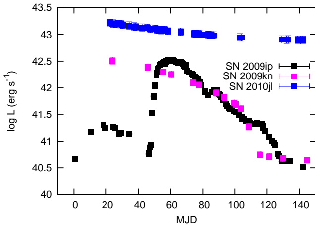
Figure 17. The uvoir bolometric lightcurve of SN 2009ip (black), together with two other well observed Type II SNe; SN 2009kn (Kankare et al. 2012) and SN 2010jl (Zhang et al. 2012). The lightcurves of SNe 2009kn and 2010jl are relative to their explosion date, while that of SN 2009ip is relative to the start of the 2012a event.
