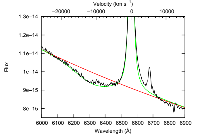
Figure 2. The region of H\alpha in our Oct 8 spectrum of SN 2009ip, showing the shallow broad absorption. In red is a blackbody fit to the continuum, while in green is the same blackbody, with a Lorentzian line of FWHM 17 \text{ Å} and a Gaussian absorption with FWHM 270 \text{ Å} superimposed. The Lorentzian plus continuum is an excellent fit to the red wing of H\alpha (with the exception of \text{He I } \lambda 6678 ), whereas in the blue wing there is an apparent absorption which is fitted by the Gaussian. As discussed in the text, it appears that the absorption may have two components, although a single Gaussian (as shown here) also gives a reasonable fit. The second x axis shows the velocity with respect to the rest wavelength of H\alpha .
