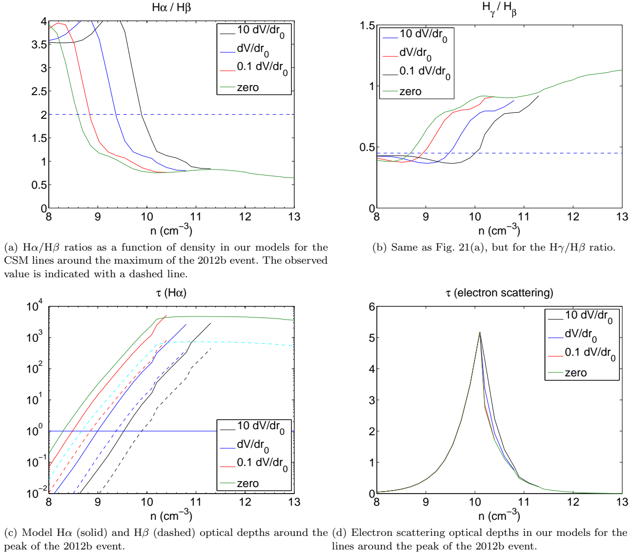
Figure 21. Results from our modeling as described in Section 5.
