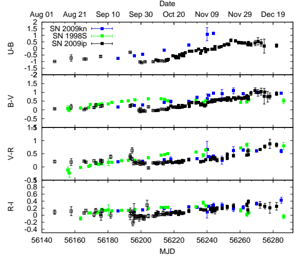
Figure 14. Optical colour curves for SN 2009ip during the 2012a and 2012b events. Open symbols are from P13, while closed symbols are from this paper. SNe 2009kn and 1998S (Kankare et al. 2012; Fassia et al. 2000) are also shown, these objects have been shifted so that their explosion epoch is at MJD=56140.
