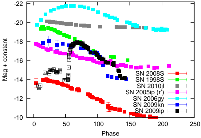
Figure 13. Comparison of the absolute R -band lightcurve of SN 2009ip with a selection of interacting transients (SN 2008S, t_0=54485.5 , A_R=1.6 , \mu=28.7 , Botticella et al. 2009; SN 1998S, t_0=50874.7 , A_R=0.56 , \mu=31.15 , Fassia et al. 2000; SN 2010jl, t_{max}=54887.5 , A_R=0.06 , \mu=33.44 , Zhang et al. 2012; SN 2005ip, t_{disc}=53679.2 , A_R=0.011 , \mu=32.71 , Stritzinger et al. 2012; SN 2006gy, t_0=53976.0 , A_R=1.68 , \mu=34.32 , Smith et al. 2007; SN 2009kn, t_0=55115.5 , A_R=0.25 , \mu=34.23 , Kankare et al. 2012). Lightcurves are plotted with respect to the explosion epoch ( t_0 ), or where a good estimate of this is unavailable, to the discovery date ( t_{disc} ) or epoch of maximum light ( t_{max} ). Distances and extinctions are taken from the literature.
