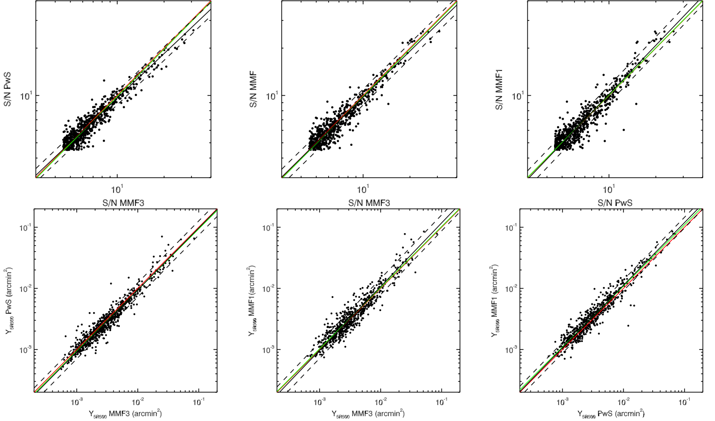
Fig. 6: Comparison of S/N (top panels) and maximum likelihood Compton-parameter values (bottom panels) from the three detection algorithms, MMF3 and PwS, down to S/N = 4.5 after removing obvious false detections (see Sect. 2.3). In each panel, the red line denotes the equality line. The black line is the best fit to the data, and the dashed lines correspond to the \pm 1\sigma dispersion about the fit relation. For clarity, error bars are omitted on Y_{5R500} values in the plot, but are taken into account in the fit. The green line of slope fixed to unity corresponds to the mean offset between the two quantities.
