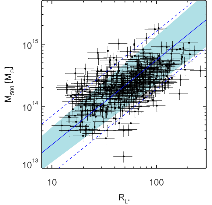
Fig. 15: Mass to richness scaling relation, M_{500} – R_{L*} , for the 444 MCXC clusters included in the WHL12 catalogue (Wen et al. 2012). The best-fit relation, from BCES fit, is given by the solid blue line. We adopted 15% uncertainties on the MCXC masses as prescribed in Piffaretti et al. (2011). As no uncertainty is provided for the WHL12’s richness, we arbitrarily assumed a 20% uncertainty for all richness values. The blue shaded area shows the associated errors on the best-fit, while the dashed line marks the intrinsic scatter.
