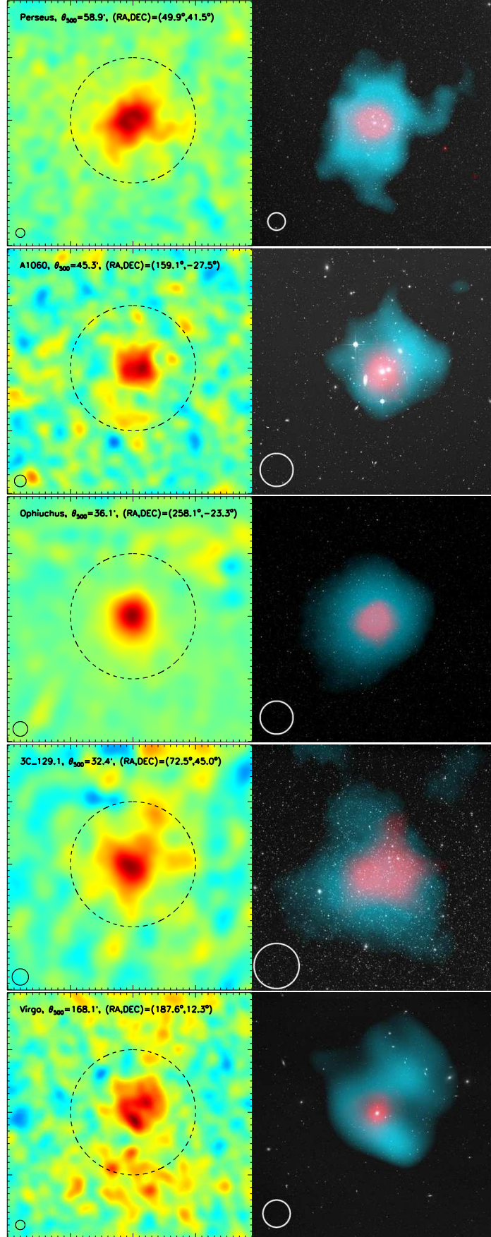
Fig. 19: Five selected nearby and extended clusters not included in the PSZ catalogue. All exhibit an extended SZ signal detected in the Planck survey. From top to bottom: Perseus cluster and Abell 1060 (in the point-source mask); Ophiuchus cluster and 3C 129.1 (in the Galactic mask); and Virgo cluster (below the S/N threshold of the catalogue). Left panels : reconstructed thermal SZ maps from the MILCA algorithm (Hurier et al. 2010). The dashed circles represent the apertures of \theta_{500} from the MCXC catalogue. Each SZ-map covers an area of 4\theta_{500} \times 4\theta_{500} . Right panels : composite images of the optical (DSS), X-ray (ROSAT) and SZ signal ( Planck ). The size of the composite images is adapted to optimize the display (Perseus: 2 \times 2 square degrees; Abell 1060: 1 \times 2\frac{1}{2} square degree; Ophiuchus: 1 \times 1 square degree; 3C 129.1: 0.77 \times 0.77 square degrees; Virgo: 3.84 \times 3.84 square degrees). The solid circle in the left corner shows, both in the SZ Planck map and in the composite image, a 10 arcmin field of view; except for Virgo for which it shows a 30 arcmin field of view.
