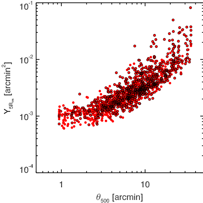
Fig. 5: Distribution of the maximum likelihood SZ flux Y_{5R_{500}} and size \theta_{500} for Planck SZ detections in the union catalogue down to S/N = 4.5 . Detections associated with known or new confirmed clusters are shown as open black circles. SZ cluster candidates are shown as filled-red circles.
