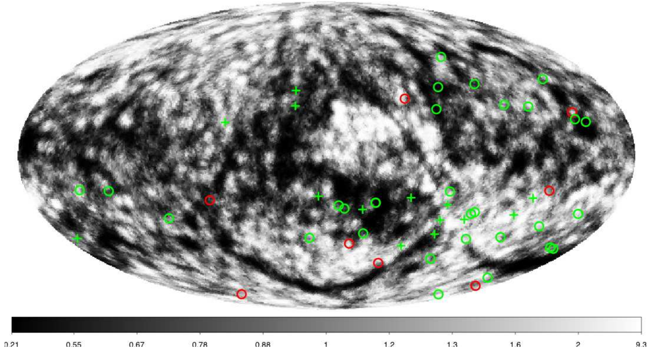
Fig. B.1: XMM-Newton validation results overlotted on density map of the RASS-Bright Source Catalogue (BSC). The source density map has been normalised by the median of the pixel density distribution. Confirmed candidates are plotted in green and false candidates are plotted in red. Pluses (+): good association with a BSC source. Circles (○): no association with a BSC source.
