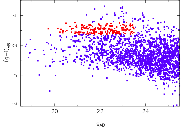
Fig. A.2: A g-i vs. g colour-magnitude diagram of non-stellar objects in the field of PLCK G147.3–16.6, observed with NOT/MOSCA. Galaxies plotted as red squares, in the region defined by g-i = 3.15 \pm 0.40 and g < 23.5 , form the red sequence constituted by early-type galaxies in the cluster.
