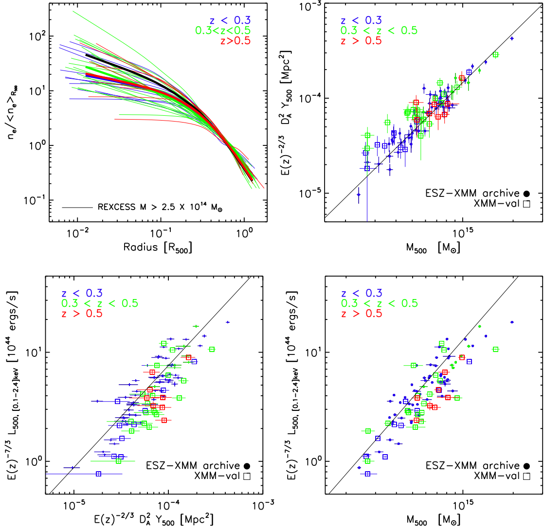
Fig. 12: Scaling properties of Planck clusters, colour-coded as a function of redshift. In all figures, R_{500} and M_{500} are estimated from the M_{500} – Y_X relation of Arnaud et al. (2010) . Top left panel : The scaled density profiles of the new clusters confirmed with XMM-Newton observations. The radii are scaled to R_{500} . The density is scaled to the mean density within R_{500} . The thick lines denote the mean scaled profile for each sub-sample. The black line is the mean profile of the REXCESS sample ( Arnaud et al. 2010 ). Other panels : Scaling relations. Squares show the new clusters confirmed with XMM-Newton observations. Points show clusters in the Planck -ESZ sample with XMM-Newton archival data as presented in Planck Collaboration XI (2011) . Relations are plotted between the intrinsic Compton parameter, D_A^2 Y_{500} , and the mass M_{500} ( top right panel ), between the X-ray luminosity and Y_{500} ( bottom left panel ) and between mass and luminosity ( bottom right panel ). Each quantity is scaled with redshift, as expected from standard self-similar evolution. The lines in the left and middle panel denotes the predicted Y_{500} scaling relations from the REXCESS X-ray observations ( Arnaud et al. 2010 ). The line in the right panel is the Malmquist bias corrected M – L relation from the REXCESS sample ( Pratt et al. 2009 ; Arnaud et al. 2010 ). The new clusters are on average less luminous at a given Y_{500} , or more massive at a given luminosity, than X-ray selected clusters. There is no evidence of non-standard evolution.
