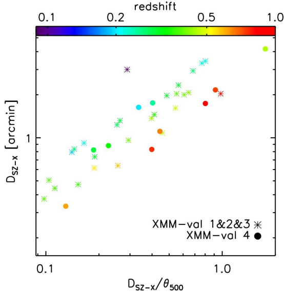
Fig. 4: Distance of blind SZ position to X-ray position, D_{\text{SZ-X}} , as a function of D_{\text{SZ-X}}/\theta_{500} for single confirmed systems. The clusters are colour-coded according to redshift.
