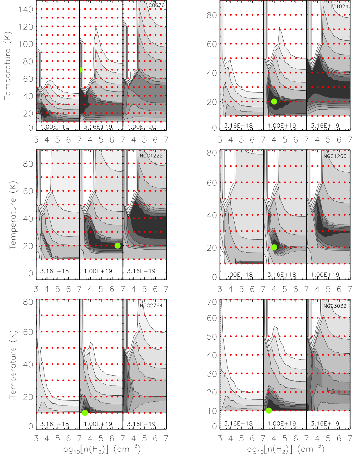
Figure 2. Best-fit models for the CO gas component. Each panel shows the \Delta\chi^2 \equiv \chi^2 - \chi^2_{\min} contours of the CO gas component as a function of the kinetic temperature T_K and H_2 volume density n(H_2) , for three values of the CO column density N(CO) (hence three plots) centered on the best-fit value and indicated at the bottom of each plot. The model grid is shown with dark-grey dots (red dots in the online version), whereas the best-fit model of each galaxy ( \chi^2_{\min} or \Delta\chi^2 = 0 ) is labeled with a light-grey filled circle (green filled circle in the online version). The \Delta\chi^2 contours and greyscales are for 1 to 5\sigma confidence levels (i.e. \Delta\chi^2 = 3.54, 6.25, 7.81, 9.35 and 11.34 when three line ratios are used and \Delta\chi^2 = 4.73, 7.78, 9.49, 11.14 and 13.27 when four line ratios are used). Additional contours of \Delta\chi^2 = 50, 100, 200 and 300 are used in these figures only for guiding the eyes further and see better how the confidence contours are spreading within the model grid. The low \sigma , high confidence level contours containing 'good' models are represented by the darkest areas. The galaxy name is indicated in the top-right corner of each panel.
