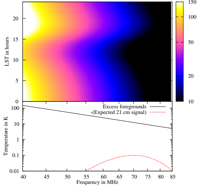
Figure 7. Plot showing the differential antenna temperature due to the inclusion of ionospheric effects in our simulations. Top panel shows the difference between the simulated dynamic spectra obtained with and without the inclusion of ionospheric effects, and the bottom panel shows the differential spectrum averaged in time. Also shown for comparison is (the negative of) the expected 21 cm signal.
