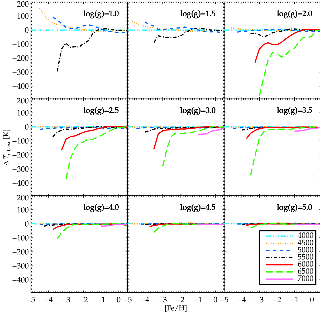
Figure 6. The lines mark the estimated NLTE effect on effective temperatures derived from excitation balance of un-saturated Fe I lines, given that other stellar parameters are fixed by independent means. All models shown have \xi_t = 2.0 km/s.
