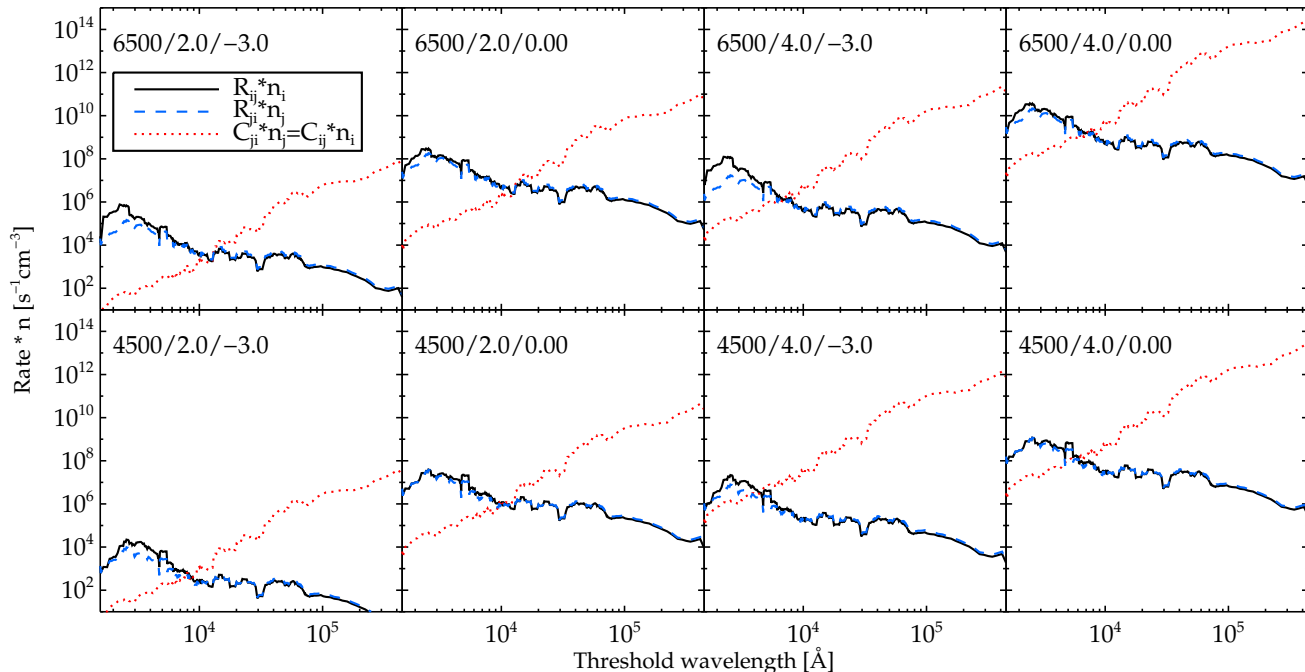
Figure 3. The panels show the total number of Fe I–Fe II ionisation and recombination events per unit time and volume for selected models at line forming layers ( \log(\tau_{500} = -2) ). The abscissa marks the threshold wavelength, n_i is the LTE level population of the lower level, and n_j the LTE population of the upper level of the corresponding transition, i.e. the ground state of Fe II. The curves have been constructed by applying a smoothing factor of ten to the individual values, so that each point on the curve represents the average of ten adjacent rates.
