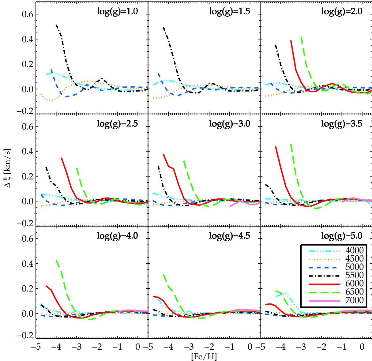
Figure 7. The lines mark the estimated NLTE effect on microturbulence velocities derived from high-excitation Fe I lines, given that other stellar parameters are fixed by independent means. The reference value in LTE is 1 \text{ km s}^{-1}
