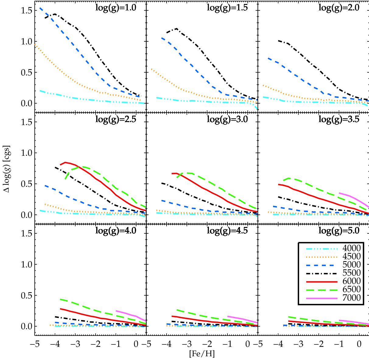
Figure 4. The lines mark the estimated NLTE effect on surface gravities derived from ionisation balance of high-excitation, unsaturated Fe I and Fe II lines, given that other stellar parameters are fixed by independent means. All models shown have \xi_t = 2.0 km/s.
