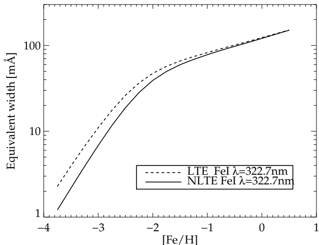
Figure 1. Example LTE and NLTE curves-of-growth for a UV Fe I transition. The model parameters are T_{\text{eff}} = 6500 K, \log(g) = 4.0 , and \xi_t = 2 km/s. The NLTE abundance correction at a given equivalent width, \Delta A(\text{Fe})_I , is defined as the difference between the two curves.
