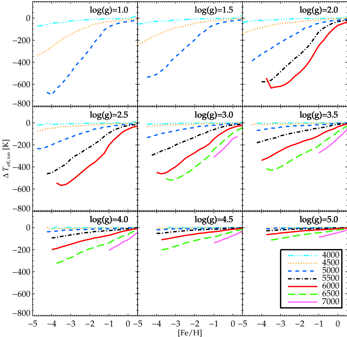
Figure 5. The lines mark the estimated NLTE effect on effective temperatures derived from ionisation balance of high-excitation, unsaturated Fe I and Fe II lines, given that other stellar parameters are fixed by independent means. All models shown have \xi_t = 2.0 km/s.
