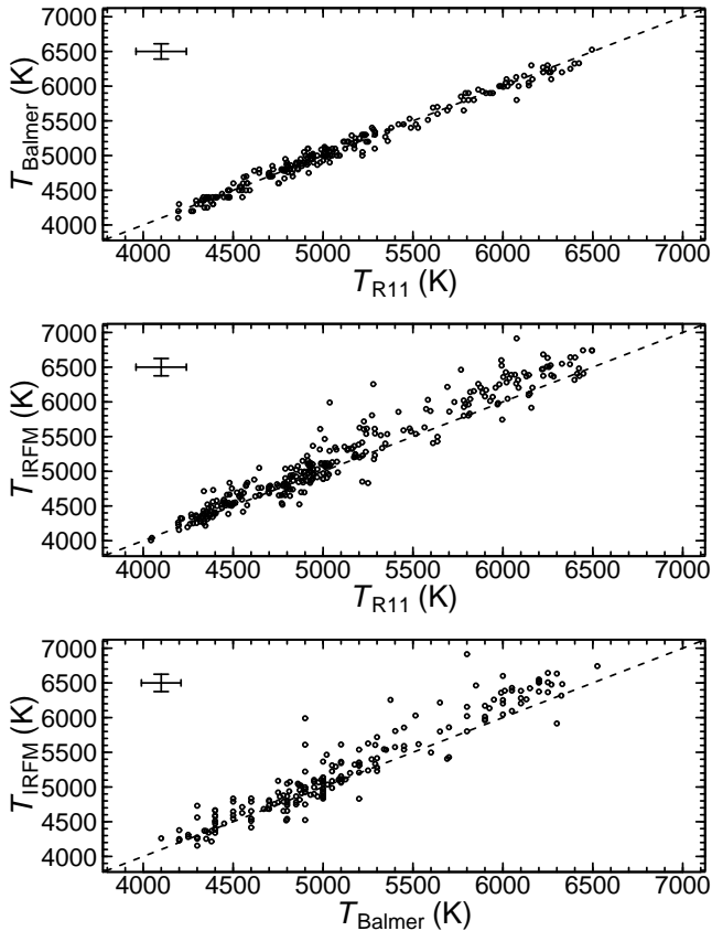
Figure 4. Comparison of the three different T_{\text{eff}} scales. Both the estimate from R11 ( T_{\text{R11}} ) and the Balmer lines ( T_{\text{Bal}} ) agree within \sim 80 K, while that from IRFM ( T_{\text{IRFM}} ) is systematically higher than both, and shows an increasing dispersion with increasing effective temperature. Error bars, which show the mean error in each T_{\text{eff}} scale, are displayed in the upper left corner.
