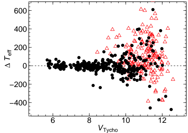
Figure 5. An illustration of the difference between different effective temperature estimates as a function of V_{\text{Tycho}} . The black, filled circles represent the difference between T(V_{\text{Tycho}}-K_s) and T(V_{\text{JC}}-K_s) for the sample of stars in C10. The red, open triangles show the difference between T_{\text{IRFM}} and T_{\text{Bal}} for the stars in our sample. For V_{\text{Tycho}} \geq 9 , both samples display an increased scatter in \Delta T_{\text{eff}} . This clearly indicates that the uncertainty in V_{\text{Tycho}} is poorly constrained for those stars.
