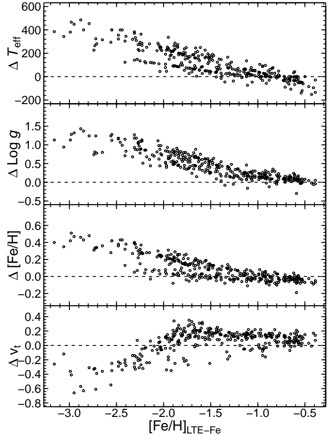
Figure 6. Comparison of stellar parameters derived using the LTE-Fe method and the NLTE-Opt stellar parameters vs. [\text{Fe}/\text{H}]_{\text{LTE-Fe}} . The difference in effective temperature, surface gravity, and metallicity show a large systematic increase with decreasing metallicity. The dual trends seen in \Delta T_{\text{eff}} , \Delta \log g , and \Delta [\text{Fe}/\text{H}] are a result of the R11 effective temperature calibration, in which the authors found that stars with effective temperatures less than 4500 K only required a small correction to T_{\text{LTE-Fe}} . Therefore, these stars stand out in the plots.
