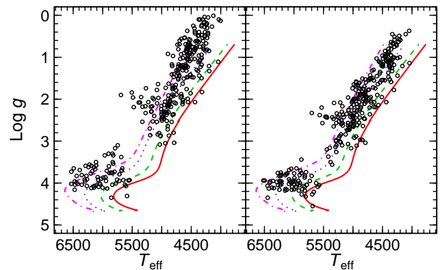
Figure 7. Stellar positions in the \log g vs. T_{\text{eff}} plane in LTE-Fe (left panel) and NLTE-Opt (right panel). The curves shown are evolutionary tracks computed using the GARSTEC code (Weiss & Schlattl 2008). Each track was computed assuming a mass of 0.8 M_{\odot} and an [\text{Fe}/\text{H}] of -0.5 (solid, red), -1.0 (long-dashed, green), -1.5 (short-dashed, blue), and -2.5 (dot-dashed, magenta). Note, those stars around \log g = 2.0 that lie away from the tracks are most likely horizontal branch stars.
