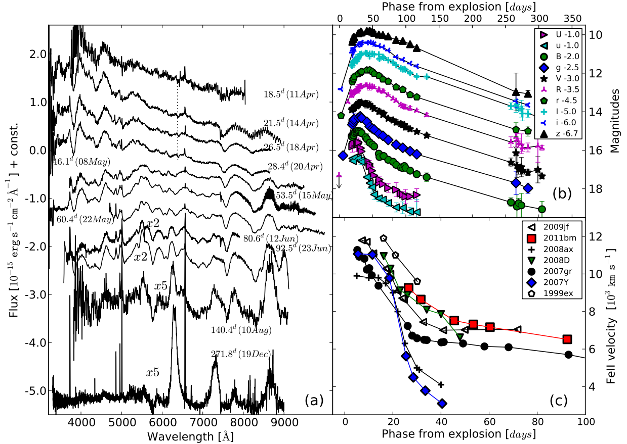
Fig. 1.— Spectroscopic and photometric follow-up of SN 2011bm. All data have been reduced with standard IRAF routines, using the QUBA pipeline (see Valenti et al. 2011 for information). For the NOT spectra, a second order correction was performed using the method described in Stanishev (2007). a: Sub-sample of our spectra in the host-galaxy frame. The dashed line marks the position of the narrow absorption line at \sim 6390 \text{ \AA} visible in our earliest four spectra. b: Multi-band light curves of SN 2011bm. c: Photospheric velocities (measured from Fe II \lambda 4924 , \lambda 5018 and \lambda 5169 ) for a sample of stripped-envelope core-collapse SNe. Data sources: SN 2007gr, Hunter et al. (2009); SN 2008D, Mazzali et al. (2008); SN 2007Y, Stritzinger et al. (2009); SN 2008ax, Taubenberger et al. (2011); SN 2009jf, Valenti et al. (2011); SN 1999ex, Stritzinger et al. (2002).
