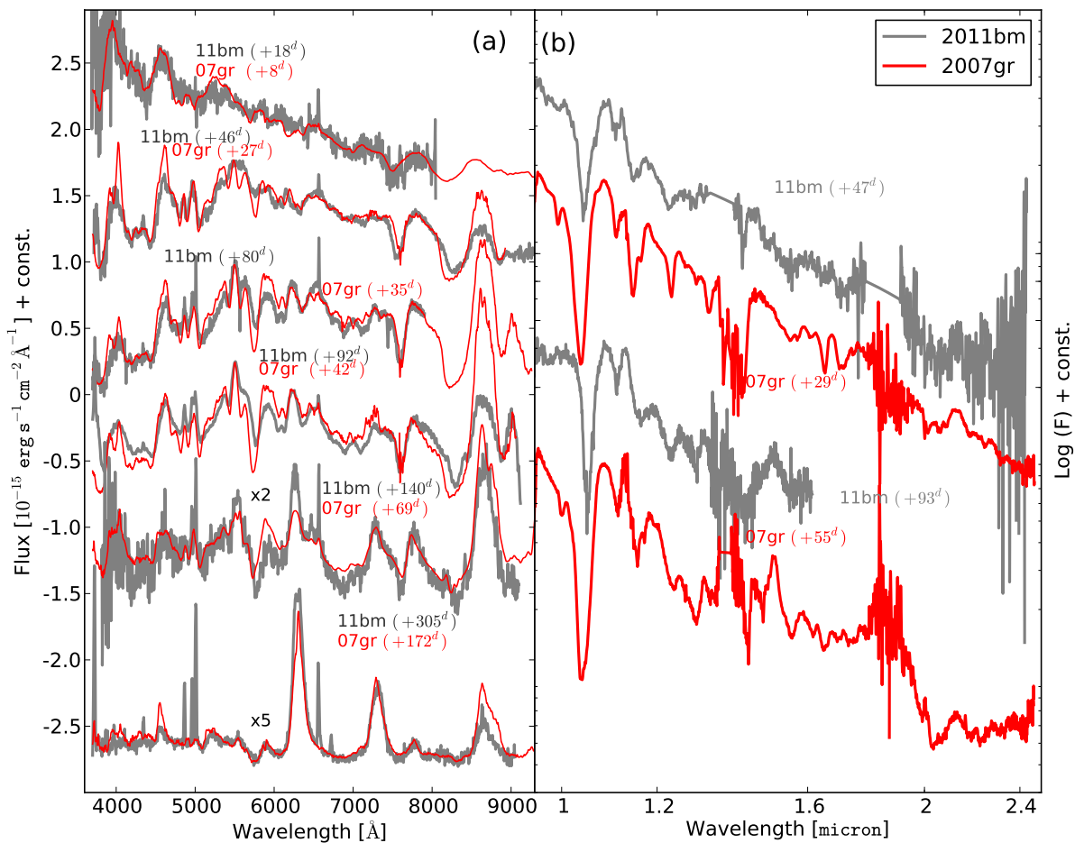
Fig. 2.— a : Spectral evolution of SN 2011bm, and comparison with spectra of SN 2007gr. The spectra of SN 2007gr have been scaled to match those of SN 2011bm. b : Infrared spectra of SN 2011bm compared with spectra of SN 2007gr.
