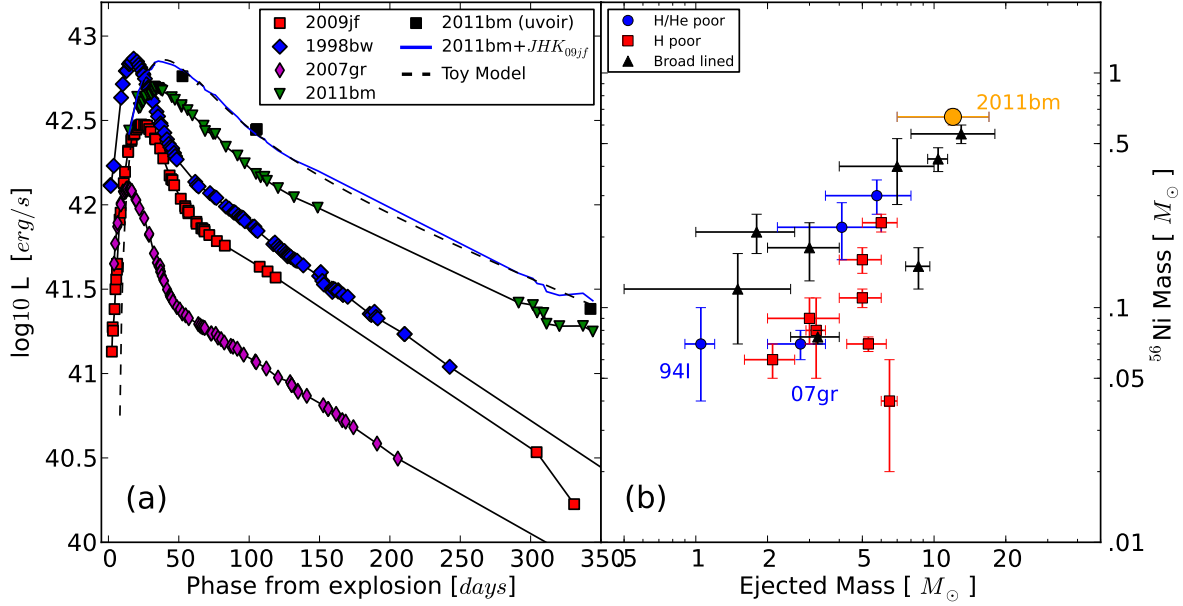
Fig. 3.— a : Pseudo-bolometric (UBVRI) light curve of SN 2011bm, compared with a set of pseudo-bolometric light curves of other stripped-envelope SNe. The blue solid line is the uvoir bolometric luminosity of SN 2011bm, computed with the UBVRI-light curve mentioned before corrected by the fractional NIR contribution of SN 2009jf (Valenti et al. 2011). The resulting uvoir bolometric light curve is consistent with the uvoir bolometric luminosity obtained for the few epochs in which JHK photometry of SN 2011bm is available (labelled as uvoir ). The dashed line corresponds to the fit to the computed uvoir bolometric luminosity with the toy model described in Valenti et al. (2008a). b : Synthesized ^{56}\text{Ni} mass versus ejecta mass for a heterogeneous sample of core-collapse SNe. Data are from Tanaka et al. (2009); Hunter et al. (2009); Valenti et al. (2011); Stritzinger et al. (2009).
