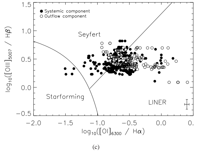
Figure 13. BPT (Baldwin, Phillips & Terlevich 1981) type diagrams for the inner parts of NGC 1266. The Y-axis of each plot shows the [\text{OIII}]/\text{H}\beta ratio derived from our SAURON data, and it is plotted versus the [\text{NII}]/\text{H}\alpha (panel a; top), [\text{SII}]/\text{H}\alpha (panel b; middle) and [\text{OI}]/\text{H}\alpha (panel c; bottom) line ratios from our GMOS observations. In the bottom right of each plot is the typical error bar associated with each point, derived from the formal fitting errors and a monte-carlo error analysis of the fluxes returned by our fitting routines. We overplot the diagnostic lines of Kewley et al. (2001, 2006), which indicate the dominant line excitation mechanism.
