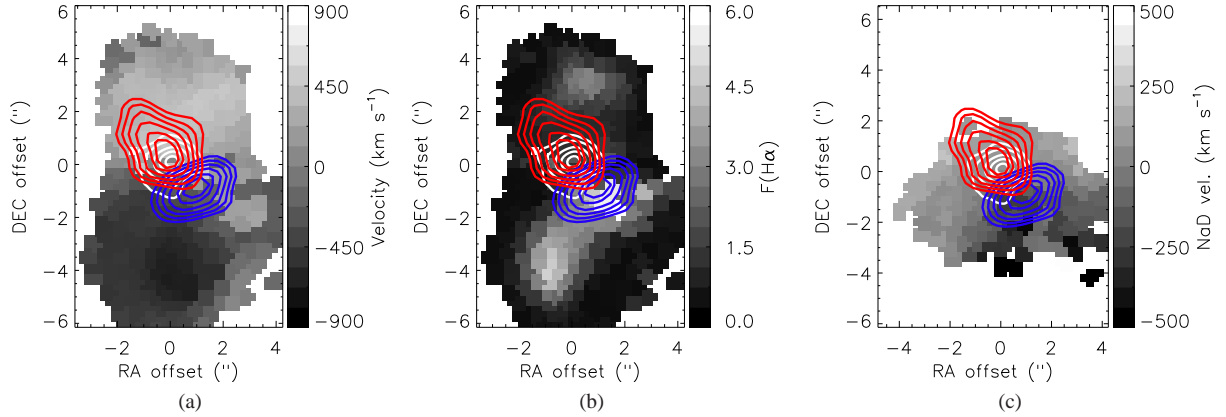
Figure 10. GMOS Ionised gas outflow kinematics (panel a), H \alpha outflow EW (panel b) and NaD kinematics (panel c), as in Figures 7, 8 and 9 but plotted in greyscale. These are overplotted with the CO observations of A2011. White contours show the molecular core, and blue and red contours the redshifted and blue shifted gas, respectively.
