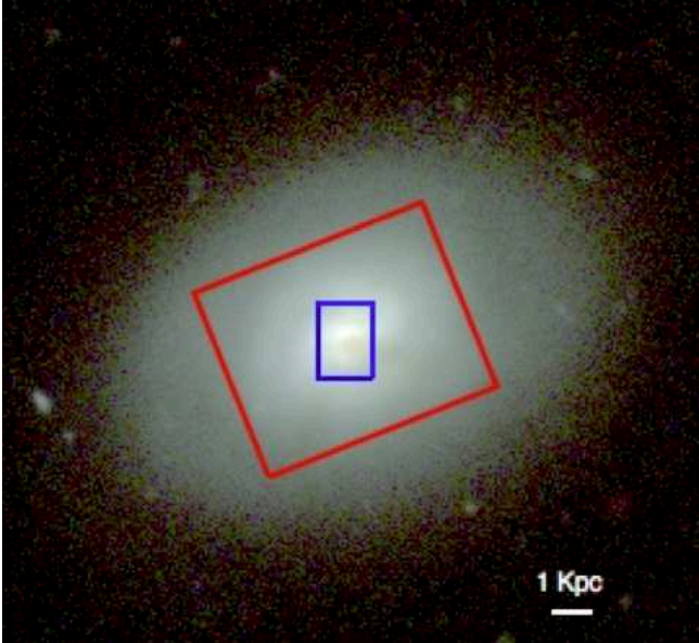
Figure 1. SINGs (Kennicutt et al. 2003) B , V and R band composite three colour image of S0 galaxy NGC 1266. The white bar shows a linear scale of 1 Kpc ( 6''.94 at an adopted distance of 29.9 Mpc; ATLAS 3D Paper I). Overlaid are the total field of view of our SAURON IFU (red) and GMOS IFU (blue) observations.
