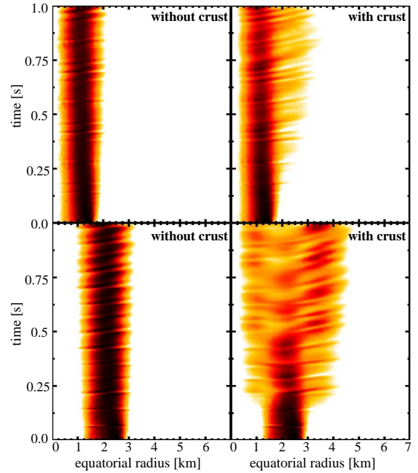
Figure 11. Evolution of the magnetic plus kinetic energy per field line divided by the sum of the energy of all field lines for the model APR+DH 1.4. The field lines are labeled by their crossing point with the equator. The pulse reaches the surface at around 70 ms for the first time and the crossing time is about 130 ms. Left panels: simulation without crust, right panels: simulation including crust. The upper and low panels differ by the location of the initial perturbation. Color scale ranges from white (minimum) to red-black (maximum).
