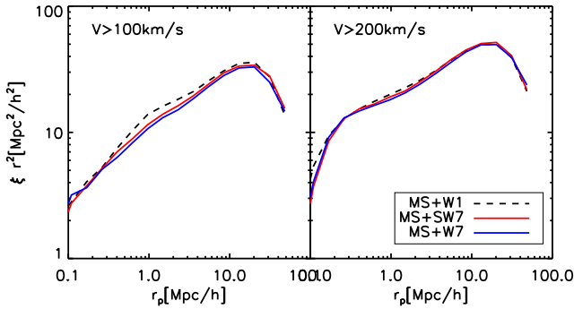
Figure 4. Autocorrelation functions for (sub)haloes with V_{max,infall} > 100 (left panel) and 200 km/s (right panel). Solid red curves are for the MS scaled to the WMAP7 cosmology while solid blue curves are for MS-W7. Dashed black curves refer to the original MS in its WMAP1 cosmology.
