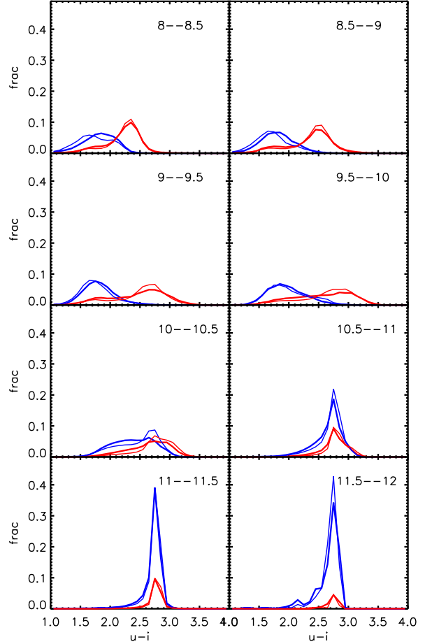
Figure 10. u-i colour distributions as a function of stellar mass for centrals (blue) and satellites (red). Thick curves are results for WMAP7 while thin curves are for WMAP1.
