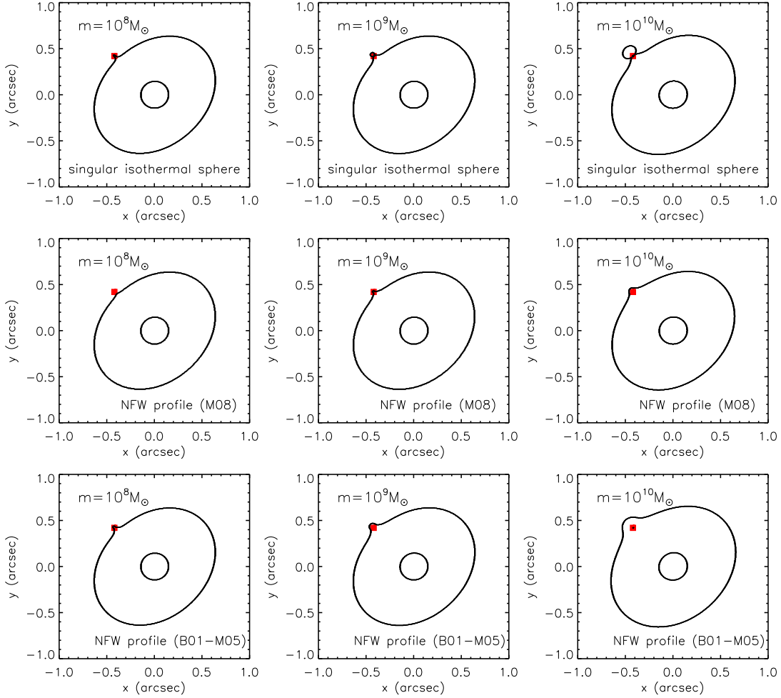
Figure 6. Critical curves for smooth lens potential with a single perturbing halo (located at z = 0.6 ), plotted as a red square. In columns from left to right the perturber has a mass of 10^8 M_\odot , 10^9 M_\odot , and 10^{10} M_\odot , respectively. The rows from top to bottom correspond to different assumptions for the density profile: a truncated singular isothermal sphere, a truncated NFW profile with the M08 concentration-mass relation, and a truncated NFW profile with the B01-M05 concentration-mass relation, respectively.
