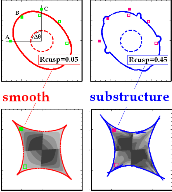
Figure 2. An illustration of how the presence of substructures affects the cusp-caustic relation. The upper panels show the critical curves in the image plane; the bottom panels are the contour maps of R_{\text{cusp}} for sources within the tangential caustic in the source plane. Squares indicate positions of close triple images and the corresponding sources in the two planes. The image opening angle \Delta\theta is labelled for one case in the top left panel. The left column shows cases with a smooth lens potential. In the right column, we show cases where substructures are present. The cusp-caustic relation is violated when a perturbing structure is projected near the image positions around the critical curve (see text).
