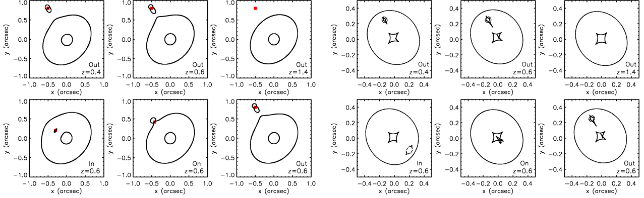
Figure 4. Critical curves (six panels on the left) and caustics (six panels on the right) produced by the same smooth lens potential plus a m = 10^{10} M_{\odot} perturber (indicated by red squares), modelled by a truncated singular isothermal sphere. Top row: the perturber’s angular position is fixed and its redshift set at z = 0.4 (in the foreground, left panel), z = 0.6 (in the primary lens plane, middle panel) and z = 1.4 (in the background, right panel). Bottom row: The redshift of the perturber is fixed ( z = 0.6 ) and its impact parameter is changed from inside the tangential critical curve (left panel, labelled as “In”), to overlapping (middle panel, labelled as “On”) to outside (right panel, labelled as “Out”). Parameters are noted in each panel. Note the wiggles induced in the critical curves and the production of secondary critical curves and caustics.
