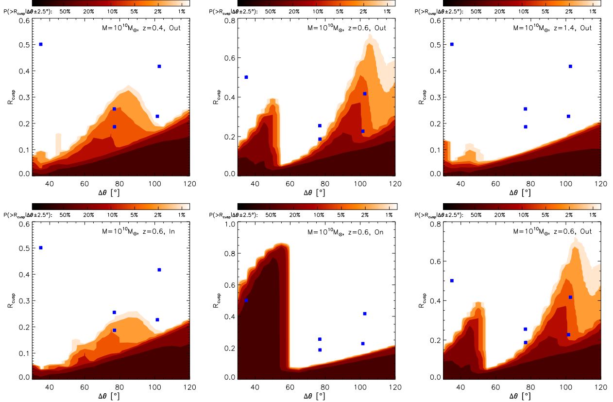
Figure 5. Corresponding probability contour maps of P(\geq R_{\text{cusp}} | \Delta\theta \pm 2.5^\circ) for cases presented in Fig. 4. Symbols and contour levels are the same as in Fig. 3. The top row presents cases where a perturber (of 10^{10} M_{\odot} ) is projected at the same angular position as shown in the upper panels of Fig. 4, but located at different redshifts: z = 0.4 (foreground), z = 0.6 (in the main-lens plane) and z = 1.4 (background); the second row shows cases where the perturber is located at z = 0.6 but projected at three different angular positions as shown in the lower panels of Fig. 4.
