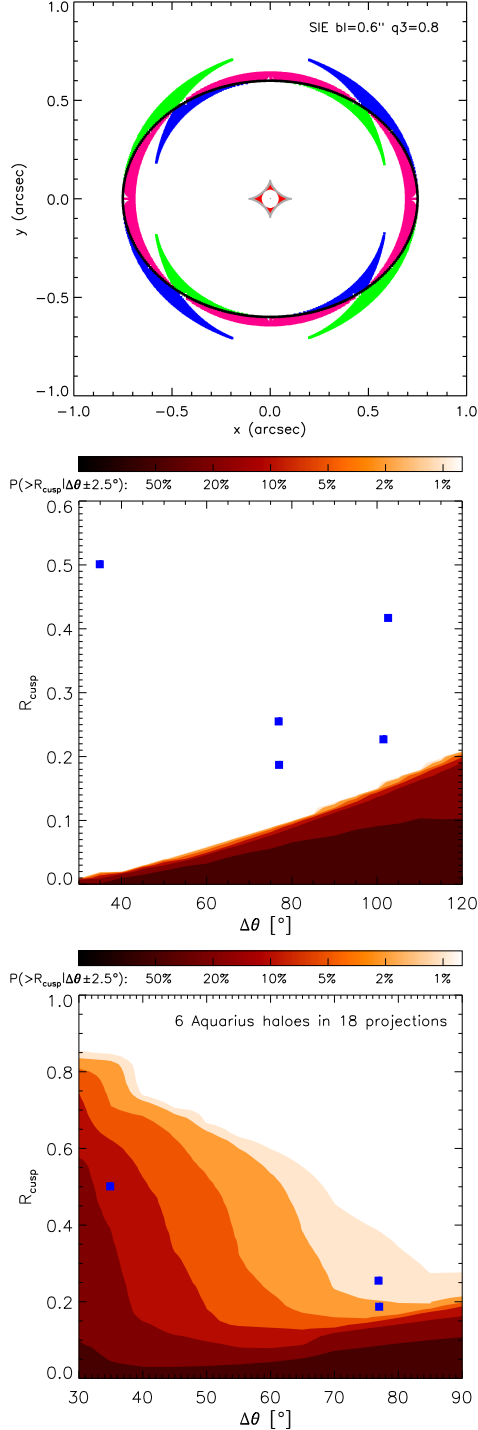
Figure 3. Top panel: Close triple image configurations for a SIE lens with b_I = 0.6'' and q_3 = 0.8 . The critical curve of the lens is shown in black and its caustics in grey. The regions sampled by “cusp sources” are shown in red, and the corresponding distributions of the three images are shown as green, pink and blue regions around the critical curve. Middle panel: the corresponding probability contour map for P(\geq R_{\text{cusp}} | \Delta\theta \pm 2.5^\circ) . Contour levels of 1%, 2%, 5%, 10%, 20% and 50% (from top to bottom) are plotted. Blue squares are the five radio measurements (with \Delta\theta \leq 120^\circ ) so far available. Bottom panel: the average probability contour map (for \Delta\theta \leq 90^\circ ) of violations due to substructures in the Aquarius haloes (using results from Xu et al. 2009).
