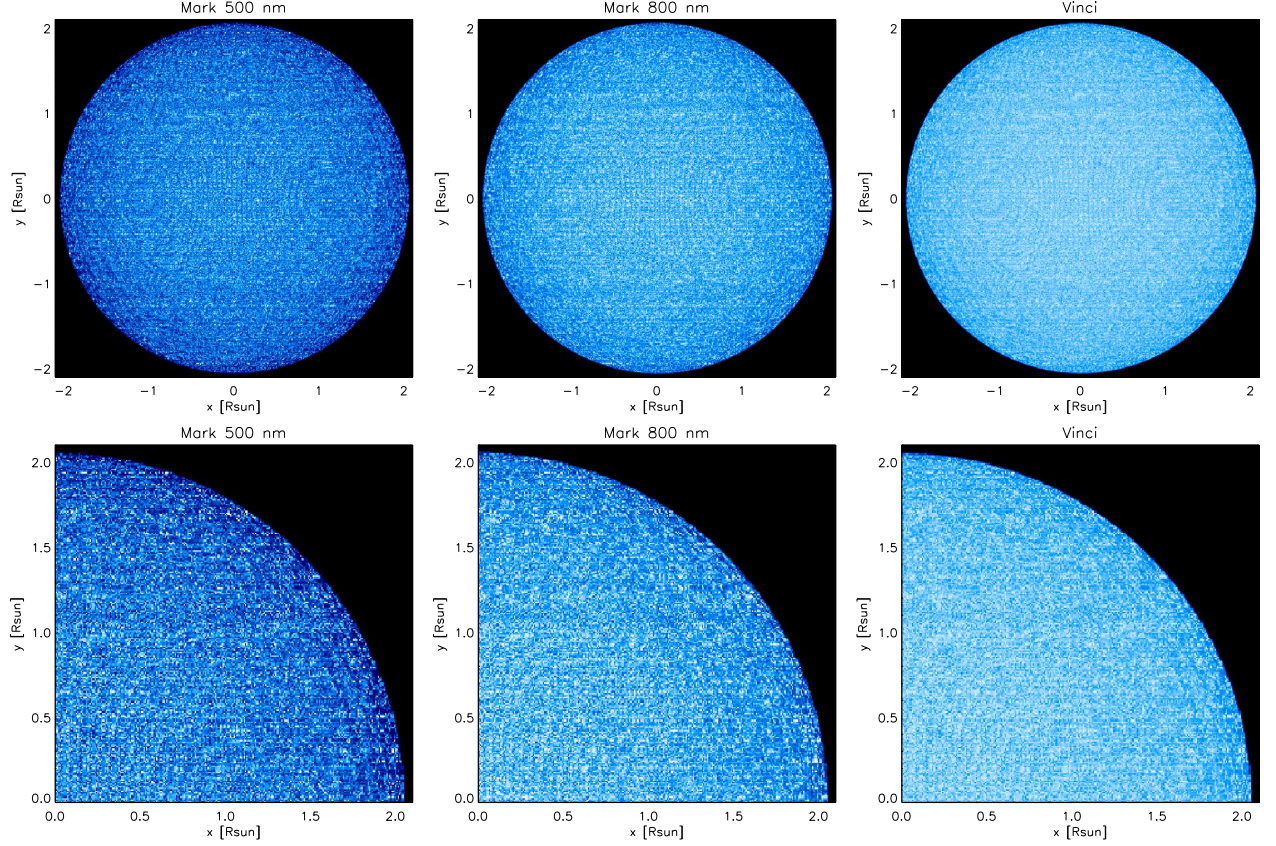
Fig. 3. Top row: synthetic stellar disk images of the RHD simulation. The intensity range is [0.3 - 1.0 \times 10^6] , [0.3 - 5.2 \times 10^5] , and [0.3 - 0.9 \times 10^5] erg cm -2 s -1 Å -1 for MARK 500 nm, MARK 800 nm, and VINCI filters, respectively. Bottom row: enlargements of the images above.
