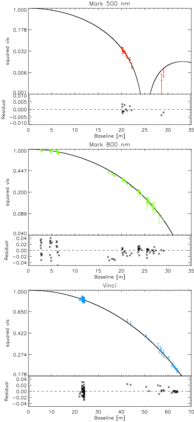
Fig. 7. Best matching synthetic visibility from Fig. 6 for the MARK 500, MARK 800, and VINCI data. The stellar disk maps in each filter have been scaled to match the radius of the star. For the MARK 500 nm filter, we used only the data with baselines higher than 20 meters.
