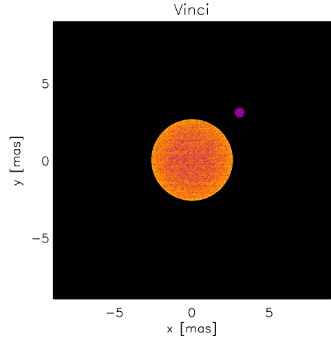
Fig. 11. Synthetic stellar disk images (yellow-orange scale) of the simulation in VINCI filter (the intensity range is [0.3 - 0.9 \times 10^5] \text{ erg cm}^{-2} \text{ s}^{-1} \text{ \AA}^{-1} ) together with a hot Jupiter (pink) at a distance of 0.1 AU for a star with a parallax of 284.56 mas (van Leeuwen 2007). The intensity of the hot Jupiter is \sim 11 times lower than the maximum stellar surface intensity.
