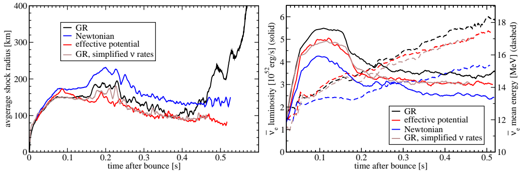
Figure 1: Left: Average shock radius for the 15M_{\odot} model as obtained in GR with our best set of opacities (black curve) and with simplified neutrino rates (light brown curve), in the purely Newtonian approximation (blue), and with an effective gravitational potential (red). Right: Electron antineutrino luminosities (solid) and mean energies (dashed) at the gain radius for these three cases.
