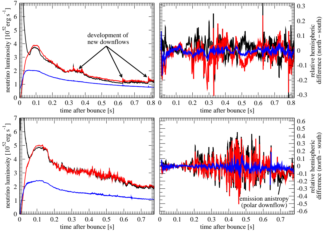
Figure 3: Left panels: Neutrino luminosities (defined as the total angle-integrated neutrino flux from the supernova) for the relativistic 11.2M_{\odot} (top) and 15M_{\odot} (bottom) models. Right panels: Relative differences of the angle-integrated neutrino fluxes L_{\text{north}} and L_{\text{south}} in the northern and southern hemisphere, computed as 2(L_{\text{north}} - L_{\text{south}})/(L_{\text{north}} + L_{\text{south}}) . Black, red, and blue curves are used for \nu_e , \bar{\nu}_e , and \nu_{\mu/\tau} , respectively.
