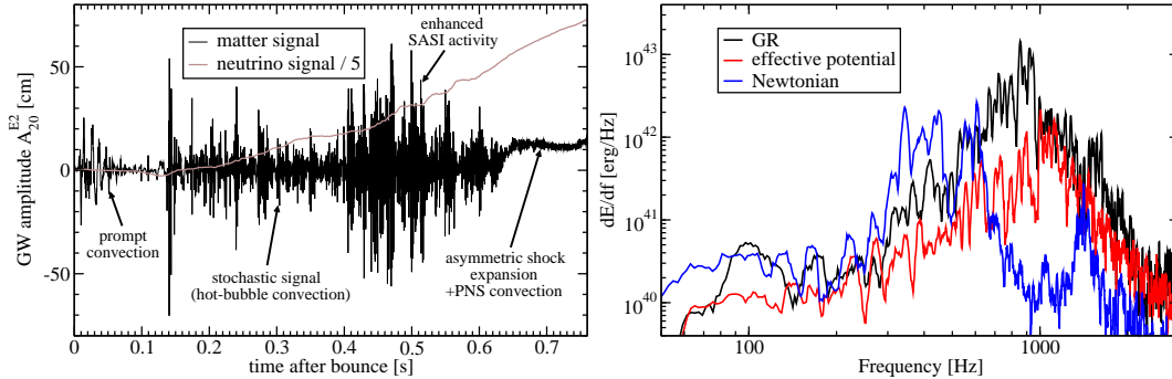
Figure 4: Left: Matter (black) and neutrino (light brown) gravitational wave signals for the general relativistic 15M_{\odot} explosion model. Right: Influence of the treatment of gravity (black: GR hydro, red: Newtonian hydro + effective potential, blue: purely Newtonian) on the gravitational wave energy spectrum for the first 500 ms of the post-bounce evolution of the 15M_{\odot} progenitor.
