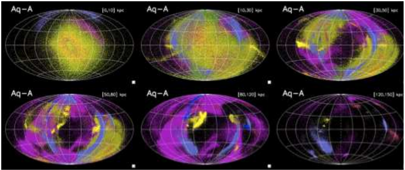
FIG. 1.— Distribution of “field” RGB stars on the sky at various distances from the “Sun” for the stellar halo of Aq-A . The different colors correspond to stars originating in different progenitors. The total number of progenitors is 163, out of which 53 contribute more than 10^4 M_{\odot} in stars. There are 35 different progenitors contributing at least 50 RGB stars in the innermost bin, and 48 at distances between 10 and 30 kpc. This number drops down to 10 in the most distant bin considered here. Thus the Aq-A stellar halo is most diverse between 10 and 30 kpc.
