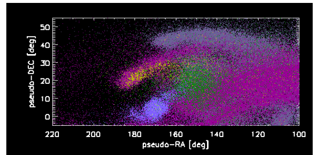
FIG. 4.— Distribution of MSTO stars in the Aquarius “Field of Streams” colored according to provenance. The region of the sky shown here has a similar extent to the SDSS footprint, but the model “stars” are located in a thin slice of 1 kpc width at a distance of \sim 35 kpc.
