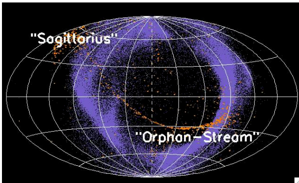
FIG. 3.— Sky distribution of RGB stars in Aq-A from the “Sagittarius” (blue) and “Orphan” (orange) streams analogues. Only those stars located at distances smaller than 80 kpc from the “Sun” are shown.
