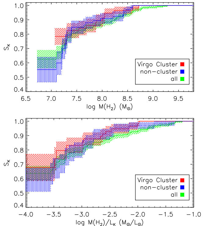
Figure 11. The Kaplan-Meier estimators for the cumulative M(\text{H}_2) and M(\text{H}_2)/L_K distribution functions ( S_K ) for ATLAS 3D Virgo Cluster members, galaxies outside of the Virgo Cluster (but at distances D \leq 24 Mpc from Earth), and for all ATLAS 3D members. The shaded regions indicate 1\sigma uncertainties on the estimated distribution functions.
