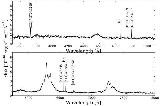
Figure 15. Host-galaxy emission lines in the late-time spectrum of SN 2009jf at +266 days from B -band maximum.
