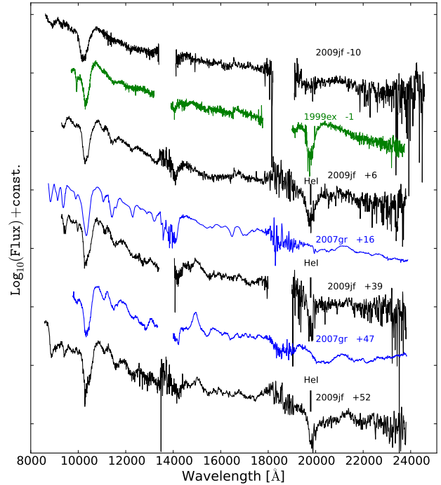
Figure 6. The infrared spectra of SN 2009jf are shown at the SN rest wavelength together with those of SN 2007gr (Ic) and SN 1999ex (Ib). He I 2.058 \mu\text{m} is marked in the spectra of SN 2009jf.
