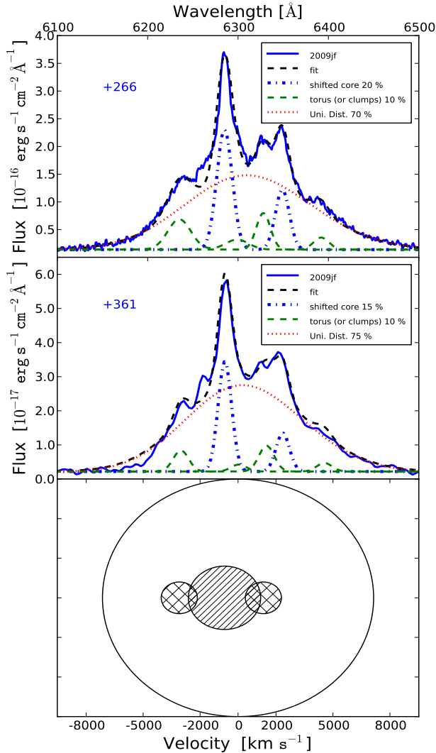
Figure 12. Oxygen line profile of SN 2009jf at +266 and +361 days from B maximum (upper and middle panel). If we assume that the oxygen line flux to trace the oxygen mass, SN 2009jf could be an asymmetric explosion, with an off-axis core ( \sim 20\% of the oxygen flux/mass) surrounded by clumps. The remaining oxygen ( \sim 70\% ) is distributed uniformly throughout the ejecta. In the lower panel a schematic reconstruction of the geometry is shown.
