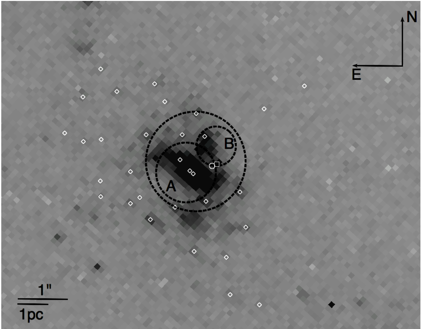
Figure 16. The HST +WFPC2 F569W image of the location of SN 2009jf. Scale and orientation are indicated. The position of the SN, as determined from the post-explosion NaCo image is located with a white circle. The radius of the circle corresponds to the 57 mas uncertainty in the SN coordinates and the geometric transformation. All sources detected by HSTPHOT within a distance of 31 pixels of the SN location (corresponding to a 500 pc radius at the distance of NGC 7479) at the 3\sigma level in both filters are indicated with white diamonds. The source located close to the SN in the F569W filter is indicated with a white square. The regions used for aperture photometry of the complexes as discussed in the text are indicated with dashed circles, and labelled accordingly.
