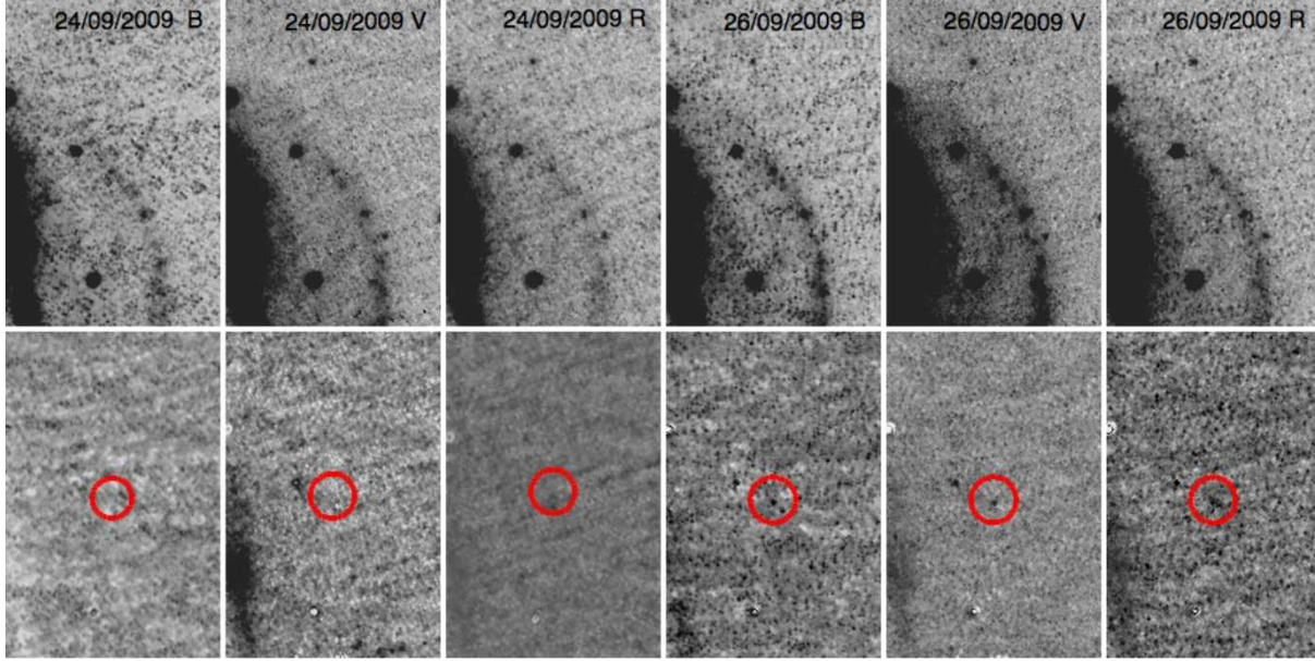
Figure 2. BVR images of SN 2009jf obtained on 24th and 26th September 2009 (upper panels) together with difference images obtained by subtracting images in the same filters obtained on 23rd September 2009 (lower panels). The marginal detections on September 26th and the non-detections on September 24th constrain the explosion epoch to 2009 September 25th ( \text{JD}=2455099.5 \pm 1 ) which is one of the best constrained explosion epochs for a stripped-envelope SN. North is up and East to the left.
