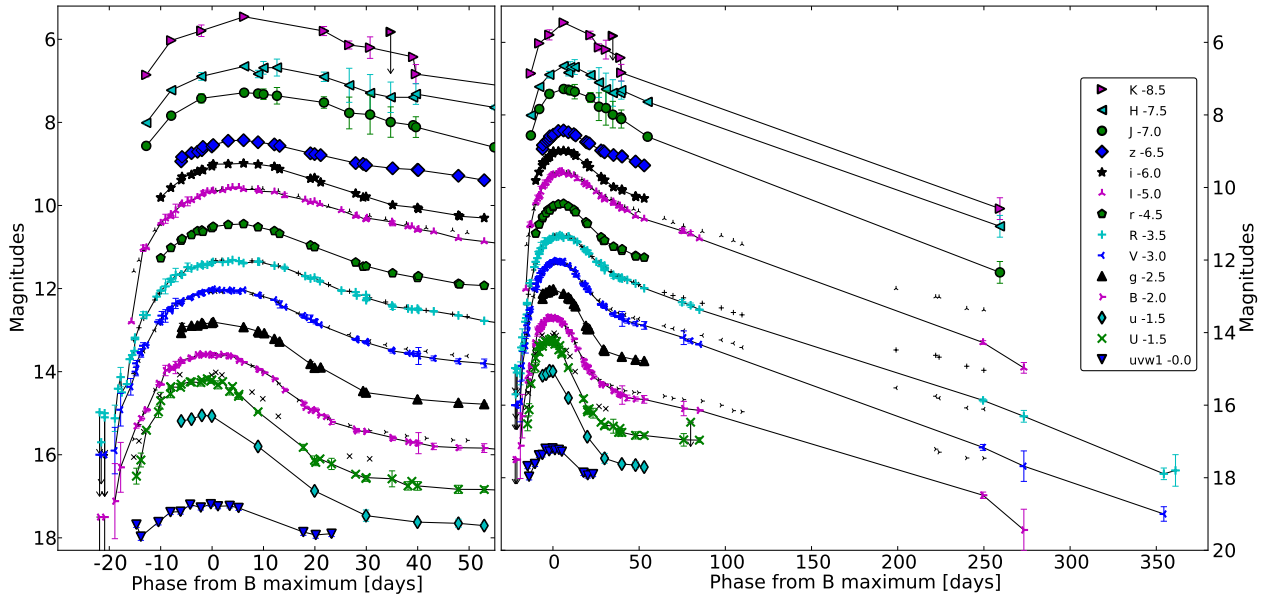
Figure 3. The light curves of SN 2009jf in the uvw1 – UuBgVrRiIzJHK bands. In the left panel we show the data from explosion to two months after B maximum ( \text{JD}=2455119.4 \pm 1.0 , 2009 Oct. 14). In the right panel, we show the full light curves in all bands. The data of Sahu et al. (2011) are overplotted with smaller symbols for comparison.
