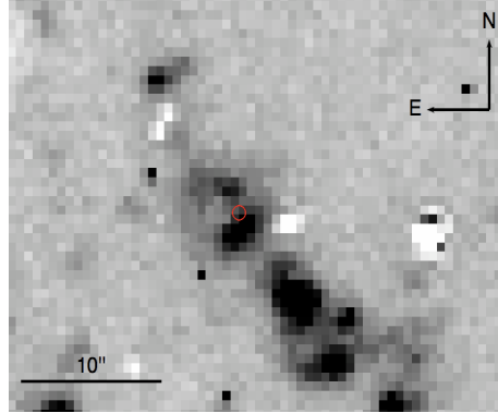
Figure 13. Continuum-subtracted H\alpha image of NGC 7479 with the SN position indicated with a circle. The radius of the circle is 10 times the uncertainty in transformation used to determine the SN position.
