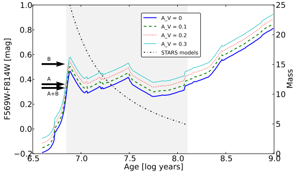
Figure 18. Padova integrated model F569W-F814W colours of a stellar population (on the left y-axis), are plotted against the age of the population for a range of extinctions. The observed colours of regions A and B, together with the total colour of the entire region (A+B) are indicated with arrows, these values have been corrected for Milky Way extinction only. The range of population ages (approximately 10 - 100 Myr) which are consistent with the cluster colours are indicated by the shaded region. Unfortunately there is a strong degeneracy in the F569W-F814W colour of the models. On the right y-axis, the ZAMS mass of single stars from the STARS code are plotted against their lifespan. A population age of 10 Myr is consistent with a progenitor mass of 25 M_{\odot} , while for an older population the progenitor must be less massive, likely \sim 8 M_{\odot} .
