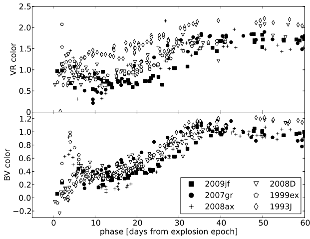
Figure 4. The B - V and V - R colour curves for a sample of stripped-envelope core-collapse supernovae.
