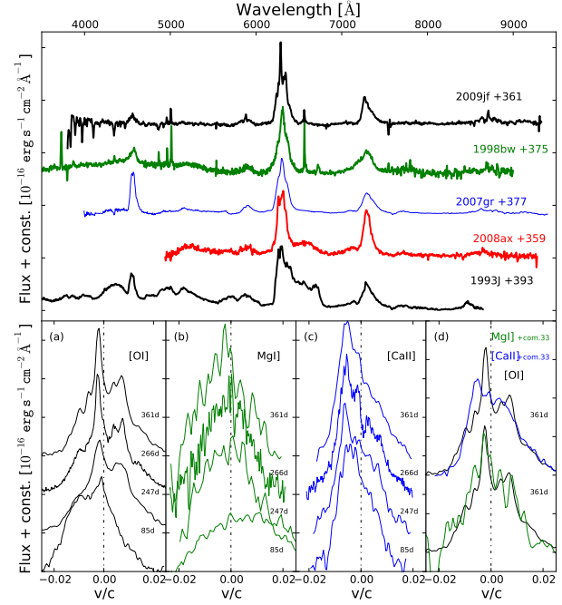
Figure 11. Upper panel: Nebular spectra (at rest frame) of a sample of stripped-envelope SNe at 1 year from B -band maximum. Bottom panel. Evolution of the main nebular features visible in the nebular spectra of SN 2009jf: (a) [\text{O I}] , (b) \text{Mg I} and (c) [\text{Ca II}] . In panel (d) we show at 361 days after B -band maximum, the comparison between the [\text{O I}] profile and profiles of the [\text{Ca II}] and \text{Mg I} modified with a second component to reproduce the [\text{O I}] doublet (see text).
