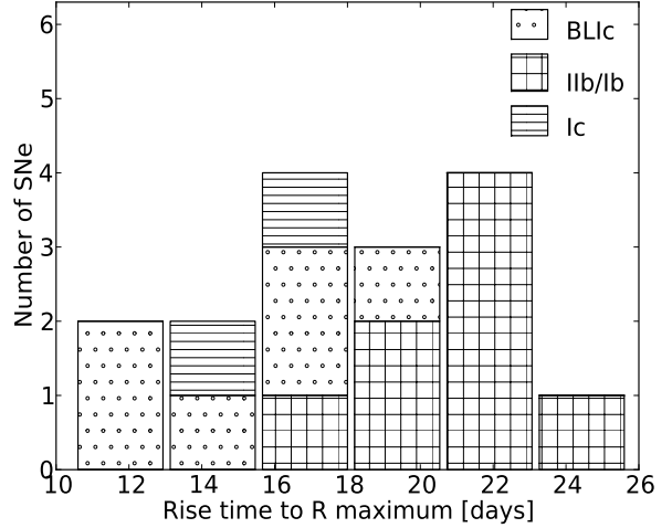
Figure 20. The rise times of a sample of stripped-envelope SNe. References for each SN: -1998bw: (from GRB 980425, Soffitta et al. 1998); -1994I: (modelling, Sauer et al. 2006); -2003jd: (pre-explosion limit Valenti et al. 2008a); -1999ex: (early discovery, Stritzinger et al. 2002); -2002ap: (modelling, Mazzali et al. 2002); -1997ef: (modelling, Mazzali, Iwamoto & Nomoto 2000); -2006aj: (from GRB060218, Cusumano et al. 2006); -1993J: (early discovery, Lewis et al. 1994); -2007gr: (good pre-explosion limit, Valenti et al. 2008b); -2008D: (from swift detection, Berger & Soderberg 2008); -2008ax: (pre-discovery limit, Pastorello et al. 2008); -1996cb: (1 day from early discovery Qiu et al. 1999); -1983N: (1 day from early discovery, Richtler & Sadler 1983); -2007Y: (1 day from early discovery, Stritzinger et al. 2009); -2009bb: (good pre-explosion limit, Pignata et al. 2011).
