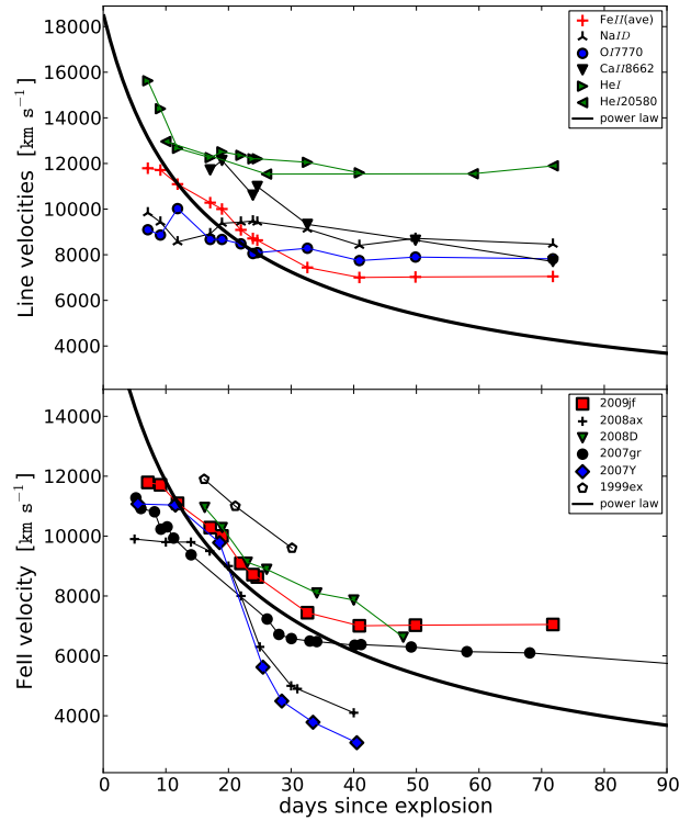
Figure 10. Upper panel: Line velocities of SN 2009jf. The Na I D and He I minima have been measured by simultaneously fitting two gaussians to the absorption feature at \sim 5600 \text{ Å} . Lower panel: The photospheric velocity evolution of SN 2009jf in comparison with those of a set of stripped-envelope SNe. All velocities were measured in IRAF with a Gaussian fit to the minimum of the line. In the both panel the solid curve show the power-law fit to the photospheric velocities of a sample of SNe Ib from Branch et al. (2002).
