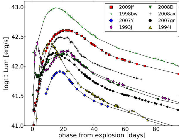
Figure 19. The bolometric light curve of SN 2009jf compared with those of other core-collapse SNe. References for each SN: - SN 2009jf: this work; - SN 1998bw: E(B - V) = 0.06 mag, \mu = 32.76 mag, phot. data: Patat et al. (2001); - SN 1994I: E(B - V) = 0.04 mag, \mu = 29.60 mag (Sauer et al. 2006), phot. data: Richmond et al. (1996); - SN 1993J: E(B - V) = 0.079 mag (Barbon et al. 1995), \mu = 27.8 mag (Freedman et al. 1994), phot. data: Barbon et al. (1995); - SN 2008D: E(B - V) = 0.65 , \mu = 32.29 mag (Mazzali et al. 2008), phot. data: Mazzali et al. (2008); Modjaz et al. (2009); - SN 2007gr: E(B - V) = 0.092 mag, \mu = 29.84 mag, phot. data: Valenti et al. (2008b); Hunter et al. (2009); - SN 2008ax: E(B - V) = 0.40 mag (Taubenberger et al. 2011), \mu = 29.92 mag (Pastorello et al. 2008), phot. data: Pastorello et al. (2008); Taubenberger et al. (2011); - SN 2007Y: E(B - V) = 0.112 mag, \mu = 31.13 mag, phot. data: Stritzinger et al. (2009).
