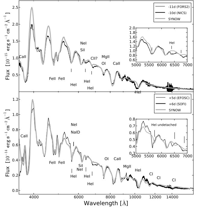
Figure 8. SYNOW fit of the spectra of SN 2009jf at -11 days and +6 days from B-band maximum light. Before maximum the He lines are present in the SYNOW fit, while in the inset, using Na instead of He, the line at \sim 6500 Å, which is likely He I L6678 is not reproduced. After maximum most of the line at 5700 Å is reproduced by Na I D. Only undetached lines of He are identified. The inset shows a SYNOW spectrum with undetached He. The spectra are at rest frame.
