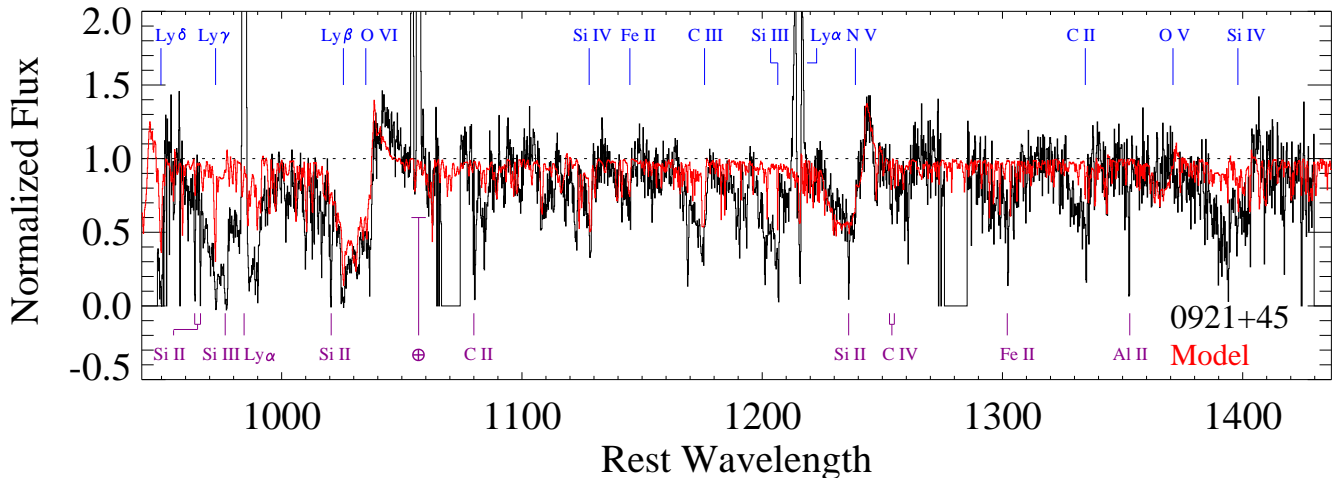
FIG. 2.— The full COS G130M and G160M spectrum of LBA0921+45 is shown in black, while an illustrative Starburst99 model spectrum is shown in red (constant star formation for ten Myr with 0.4 solar metallicity and a Chabrier IMF). Both spectra have been normalized to unit flux (see text). Prominent spectral features in the starburst are labeled at the top, while Milky Way and geocoronal features are labeled at the bottom.
