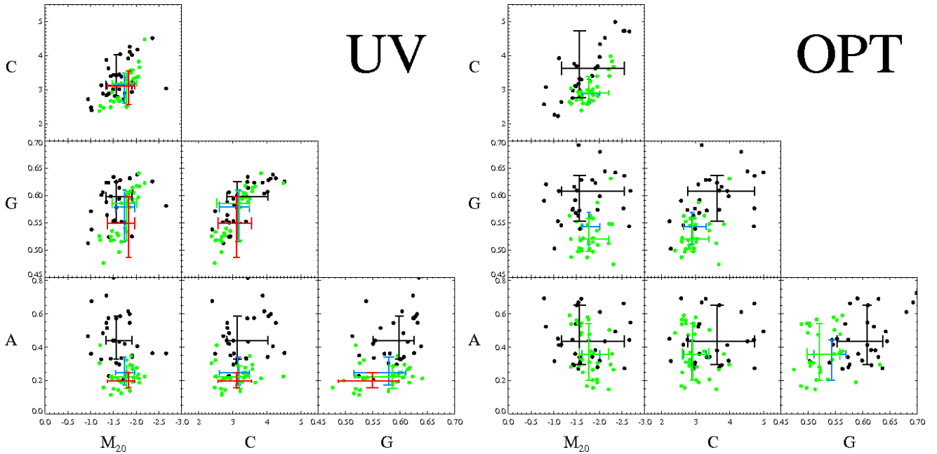
FIG. 5.— Distributions of the morphological parameters G , C , A , M_{20} for the LBAs at their true and simulated redshifts in the rest-frame UV (left) and optical (right). Black crosses indicate the 15–85 percentile ranges measured off the true (low-redshift) images. For comparison we indicate the ranges found for LBAs redshifted to z = 2 (blue crosses), z = 3 (green crosses), and z = 4 (red crosses). The z \sim 4 sample is not shown on the right as we lack a sufficiently red band to probe the rest-frame optical light. Small symbols indicate the individual measurements for the LBAs at their intrinsic (low) redshift (black points) and LBAs simulated at z = 3 (green points).
