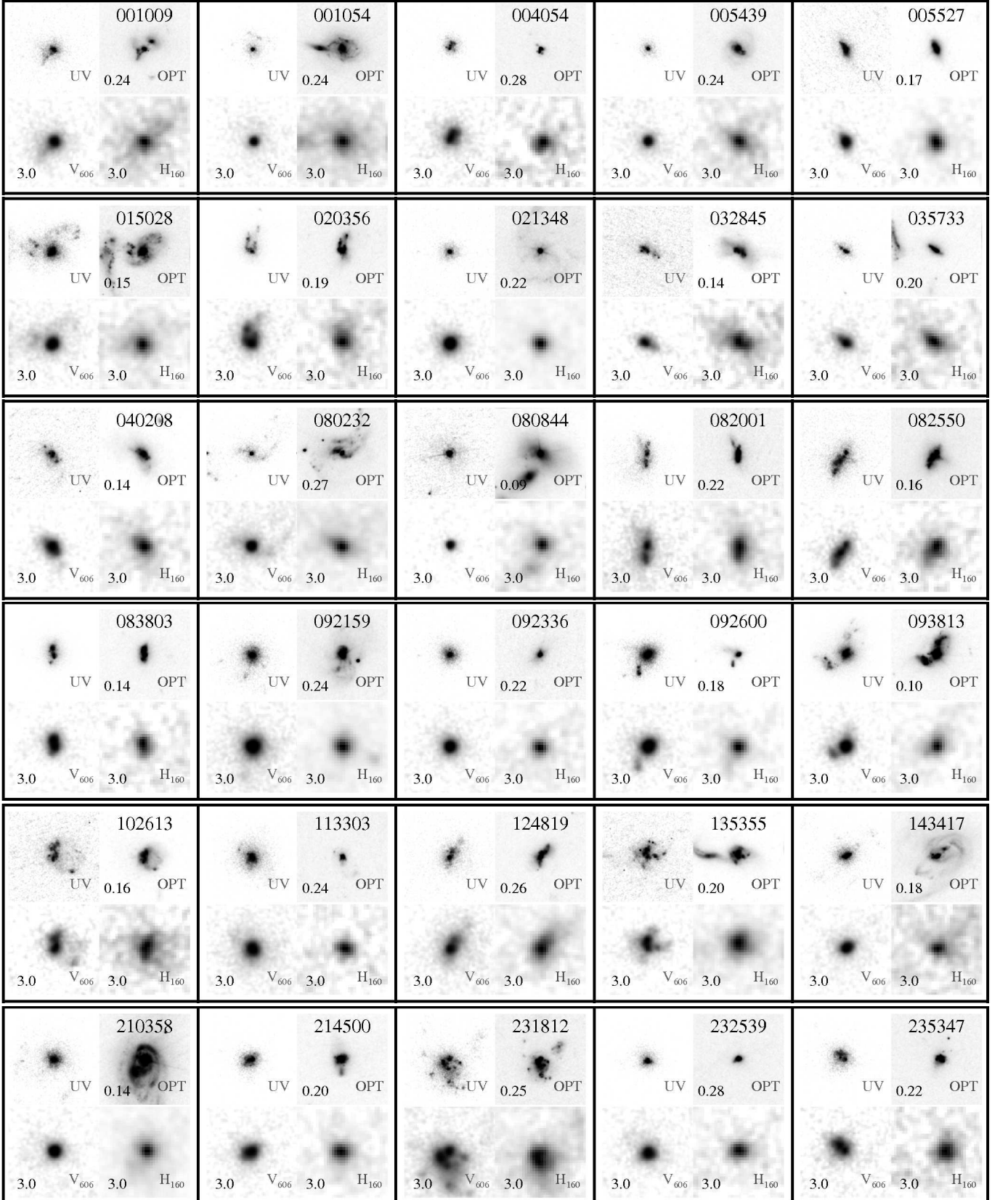
FIG. 1.— HST images of LBAs in the UV and optical at their true and simulated redshifts. For each object, we show a set of four postage stamps. The top-left and top-right show the observed UV ( 6'' \times 6'' ) and optical ( 10'' \times 10'' ) images, respectively. The ID numbers and redshifts from Overzier et al. (2009) are indicated in the optical (‘OPT’) stamps. Below these images we show the same object simulated at z = 3 and observed at the HUDF depth through the ACS/WFC V_{606} and WFC3/IR H_{160} filters probing the rest-frame UV (bottom-left) and optical (bottom-right), respectively. The simulated images measure 2'' \times 2'' . The observed UV images most often show one to several high surface brightness clumps, while in many of the optical images faint tidal features and companions suggest that the UV-bright starburst regions are triggered by mergers between small galaxies. In most cases the UV and optical light distributions are very similar, although in a small number of cases (e.g., objects 080844 and 210358) the UV emission is dominated by a single point-like source situated in a more extended and often disturbed disk seen in the optical (these objects were referred to as Dominant Central Objects (DCOs) in Overzier et al. (2009)). In most cases, the loss in sensitivity and resolution in the artificially redshifted images causes the UV clumps to blend into larger regions and hides the underlying structures and subtle features associated with the mergers seen in the optical. For color
