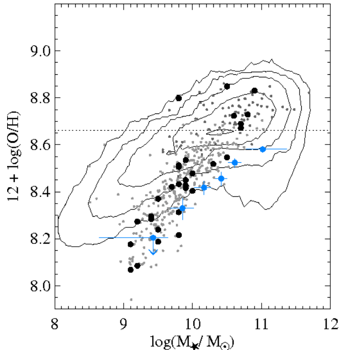
FIG. 3.— The stellar mass-metallicity ( M_* - Z ) relation. Contours indicate the distribution from a large sample of star-forming and composite objects at z < 0.3 extracted from the SDSS/DR7 spectroscopic sample. Large black symbols indicate the values measured for individual objects in our LBA sample from Overzier et al. (2009). Blue symbols indicate the average values found for star-forming galaxies at z \sim 2 in several mass bins from Erb et al. (2006). The grey points indicate the M_* - Z distribution of a statistical sample of \sim 500 LBAs extracted from the GALEX/GR5 and SDSS/DR7 crossmatched samples (Overzier et al. 2010, in prep.). Objects identified as star-forming/AGN composites have been indicated using a darker shade of grey. All metallicities have been estimated using the “N2” method based on the [NII]/H \alpha ratio from Pettini & Pagel (2004). The horizontal dotted line indicates solar metallicity, and we note that the metallicities derived using the N2 method saturate near this line.
