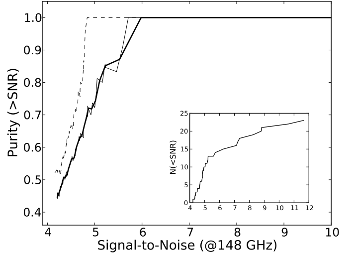
Figure 13. The SZE sample purity greater than a given SNR in the ACT 148 GHz maps. The purity is defined as the ratio of the number of confirmed clusters to the number of observed clusters. The thick solid line represents the purity binned in n=2 events, while the thin line represents no binning. The dashed line represent the fraction of candidates from the sample greater than a given SNR that were actually observed. The inset plot shows the cluster cumulative distribution as a function of SNR for the optically-confirmed cluster sample.
