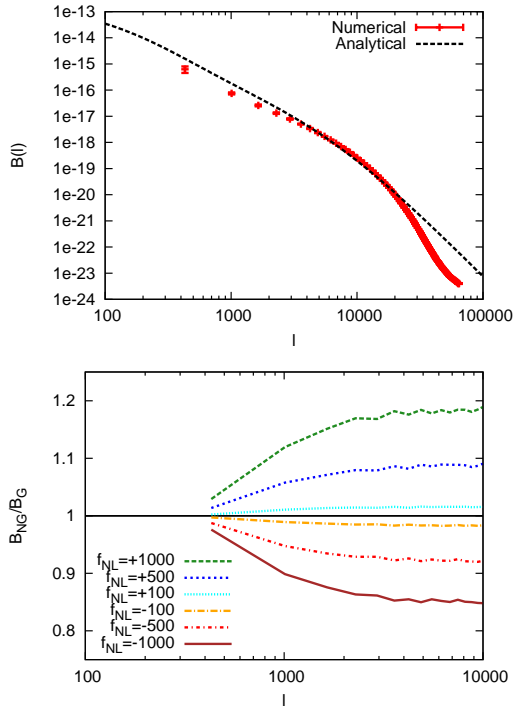
Figure 6. Top panel: comparison between theoretical predictions and our numerical estimates, derived as average of 60 different realizations of the bispectrum for the effective convergence. Error bars represent the r.m.s. of the 60 different realizations. The results refer to the Gaussian model only. Bottom panel: the ratio between non-Gaussian and Gaussian estimates for the bispectrum as a function of the multipole \ell . Different color lines refer to various values of f_{\text{NL}} as indicated in the labels.
