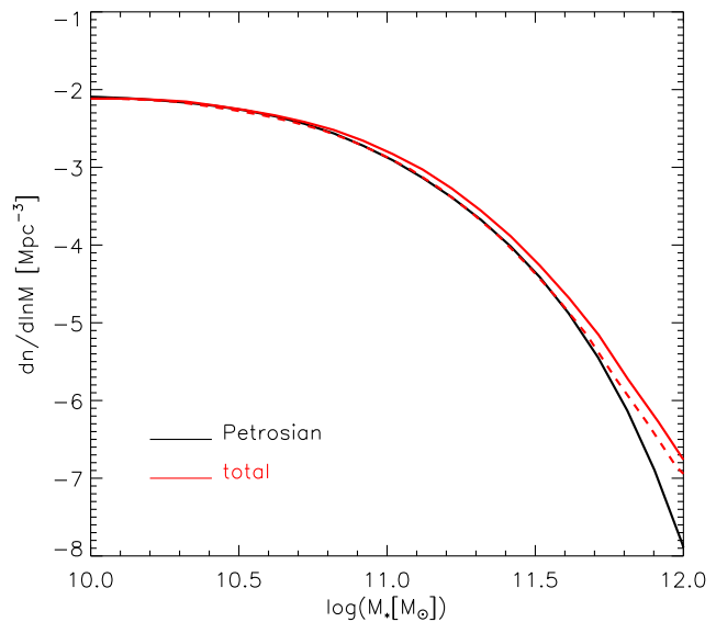
Figure 7. A comparison of the stellar mass function of Li & White (2009), which was based on the SDSS r -band Petrosian magnitudes, to a similarly calculated “total” stellar mass function based on the SDSS r -band model magnitudes. The dashed line shows the latter function shifted to smaller masses by 0.04 dex. Except at the highest masses, this is a good representation of the difference between the two mass functions.
