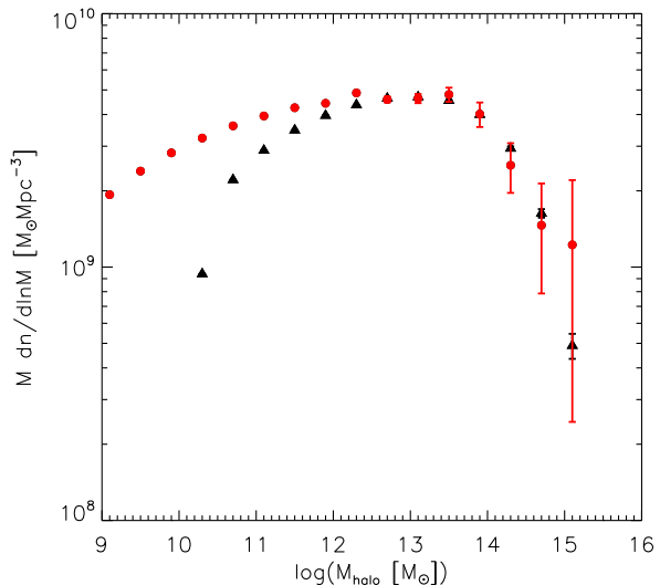
Figure 1. Dark matter halo mass functions at z = 0 where “halo” is defined to include both main subhalos and satellite subhalos. Halo mass, M_{halo} , is defined as the current virial mass for main subhalos and as the virial mass immediately prior to accretion for satellite subhalos. In both cases this is normally the maximum mass attained over the subhalo’s history. Black triangles are for the MS and red dots are for the MS-II. Poisson error bars based on halo counts are shown for both simulations.
