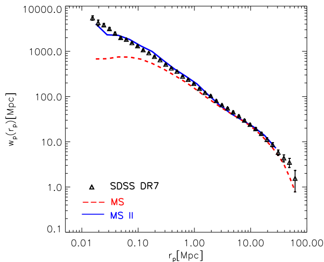
Figure 4. The projected stellar mass autocorrelation function in the SDSS/DR7 as measured by Li & White (2009) is plotted as triangles with error bars and is compared to the result obtained if z = 0 (sub)halos in the MS (dashed line) and the MS-II (solid line) are populated with galaxies according to the M_* - M_{halo} relation of Fig. 2.
