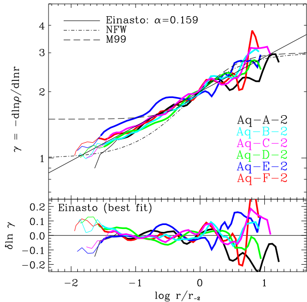
Figure 6. As Fig. 5, but for all level-2 resolution Aquarius halos, after scaling radii to r_{-2} .
