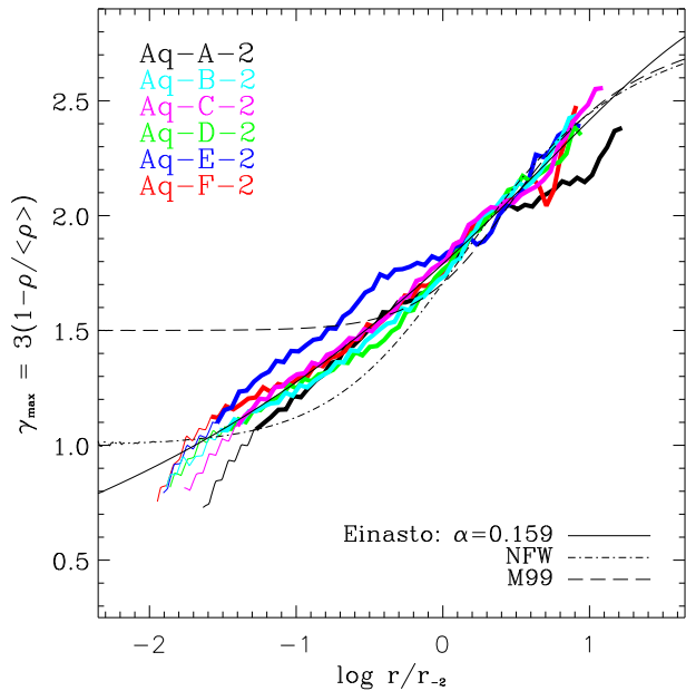
Figure 8. As Fig. 7, but for our six level-2 Aquarius halos. Results are similar in all cases and rule out cusps steeper than r^{-1} for \Lambda CDM halos.
