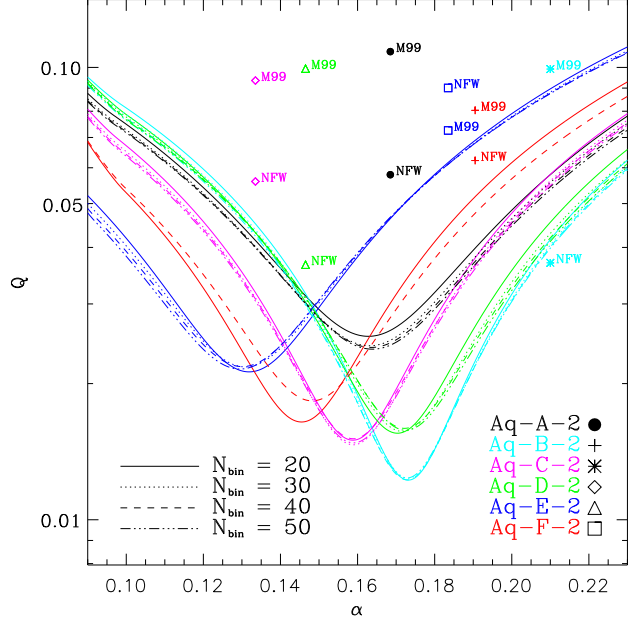
Figure 4. Minimum- Q values as a function of the Einasto parameter \alpha for best fits to all level-2 halo profiles in the radial range 0.01 < r/r_{-2} < 5 . Colors identify different halos, and line types the number of bins chosen for the profile. The minimum- Q values obtained for NFW and M99 best fits are also shown, and are plotted at arbitrary values of \alpha for clarity. Note that Einasto fits are consistently better than NFW which are consistently better than M99, and that a significant improvement in Q is obtained when letting \alpha vary in the Einasto formula. Q is approximately independent of the number of bins used in the profile, and is minimized for different values of \alpha for each individual halo. See text for further details.
