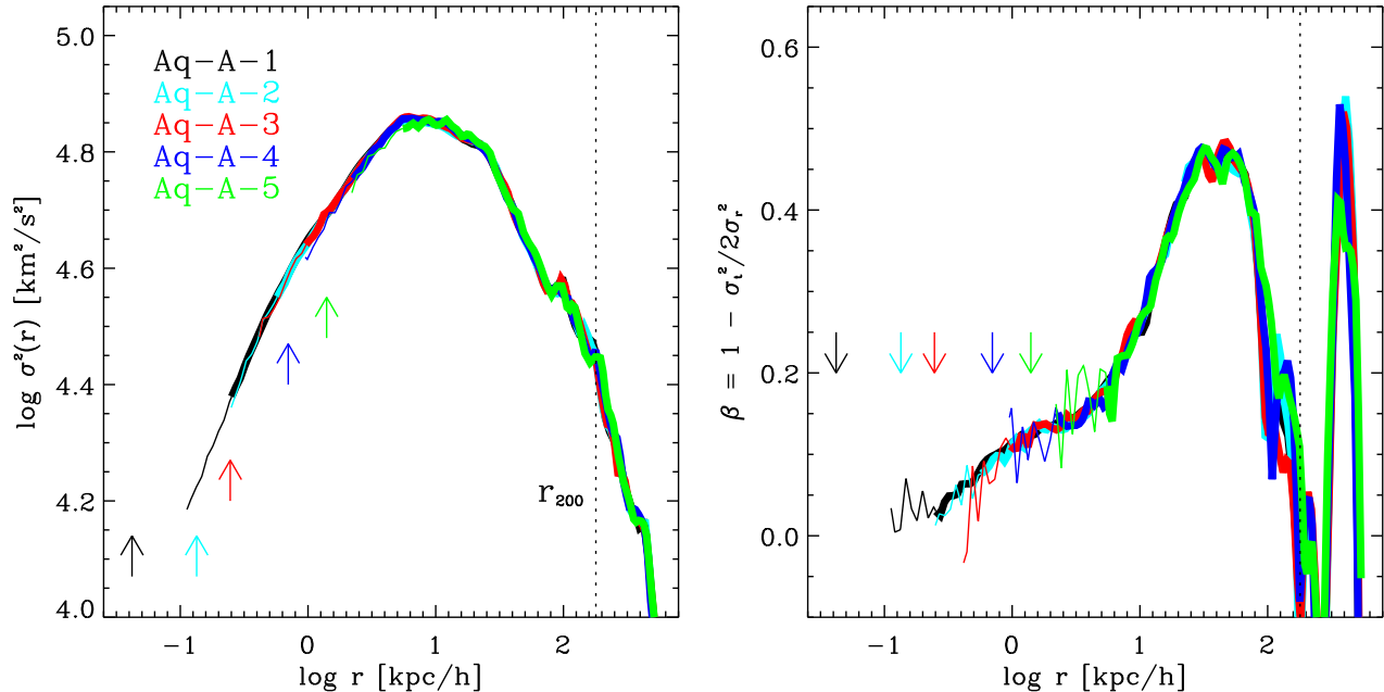
Figure 9. Left panel: Velocity dispersion profiles for our Aq-A convergence series. Arrows, line-types and colours are as in Fig. 1. Note the excellent numerical convergence. The shape of the velocity dispersion profile is remarkably similar to that of the r^2\rho profile shown in Fig. 1, highlighting the intimate connection between the density and velocity dispersion profiles which is responsible for the power-law behaviour of the pseudo-phase-space density profile discussed in Sec. 4.4. Right panel: Anisotropy profiles for the Aq-A convergence series. Note the non-monotonic variation with radius: the halo is nearly isotropic near the centre, is dominated by radial motions at intermediate radii, but becomes markedly less anisotropic near the virial radius.
