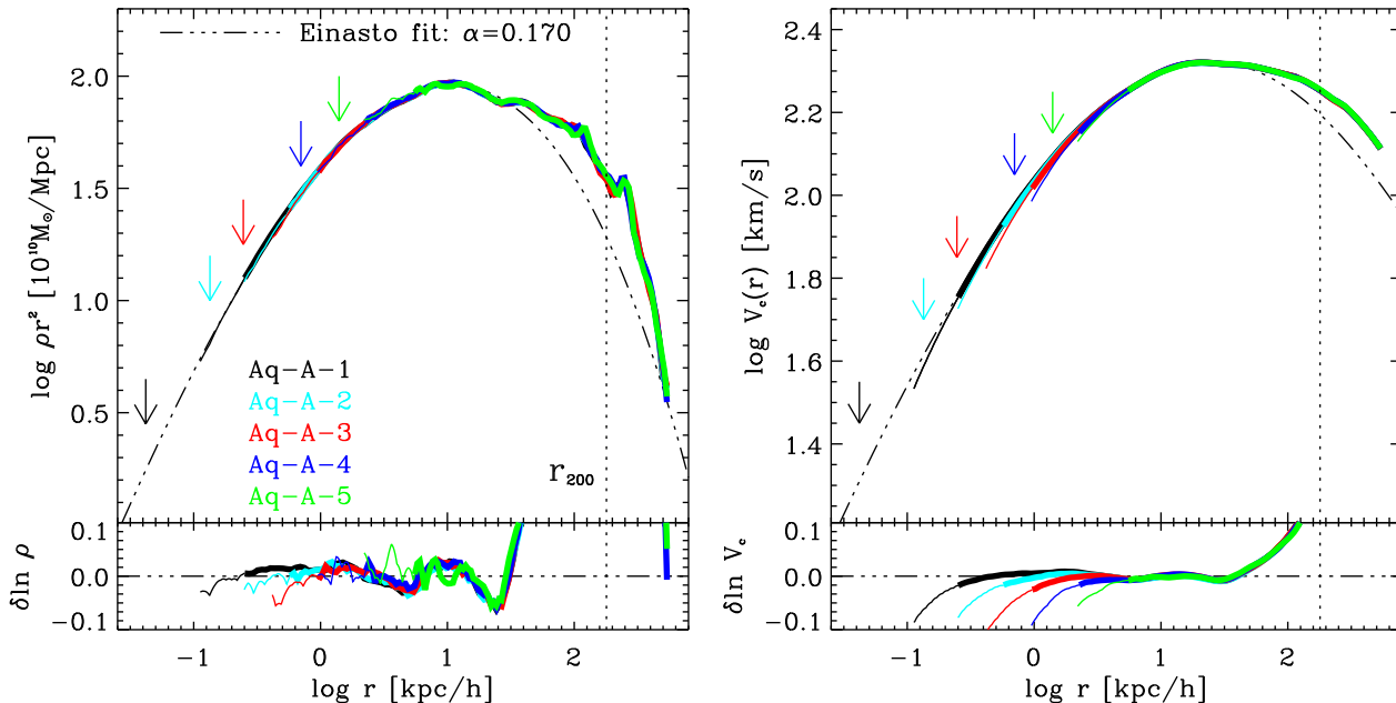
Figure 1. Spherically-averaged density (left) and circular velocity (right) profiles for the Aq-A halo simulation series. Different colours correspond to different resolution runs, as labeled in the figure. The density profile is multiplied by r^2 in order to emphasize small deviations. The bumps in the outer regions may be traced to the presence of substructure and unrelaxed tidal debris. Profiles are shown from \sim 3r_{200} down to the “convergence radius”, r_{\text{conv}}^{(1)} , corresponding to the radius where the relaxation time, t_{\text{relax}} , is of the order of the age of the Universe. The thick portion of each profile indicates the region r > r_{\text{conv}}^{(7)} where t_{\text{relax}} is more than 7 times the age of the universe and where stricter convergence is achieved. Outside r_{\text{conv}}^{(7)} circular velocity estimates converge to better than 2.5% (see Fig. 2). The dot-dashed line shows an Einasto profile with \alpha = 0.17 matched at (r_{-2}, \rho_{-2}) , the peak in the r^2\rho profile. This provides an excellent fit to the structure of the inner regions of the halo, as shown by the residuals plotted in the bottom panels. Arrows indicate the softening length h_s of each simulation.
