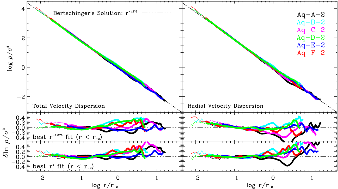
Figure 13. Pseudo-phase-space density profiles of all six level-2 Aquarius halos. Radii have been scaled to r_{-2} , and the pseudo-phase-space densities to maximise agreement within r_{-2} . Note that for all six halos these profiles are very well approximated by power laws with an exponent very close to that of the Bertschinger solution. All halos, including those that were outliers in the density, velocity dispersion, and anisotropy profiles, are almost indistinguishable in this plot. Deviations from the Bertschinger law are typically more pronounced when radial velocity dispersion is used instead of the full 3D velocity dispersion. Residuals from the best-fit power-laws, \rho/\sigma^3 \propto r^\chi , are shown in the bottom panels. The values of \chi are listed for each halo in Table 2.
