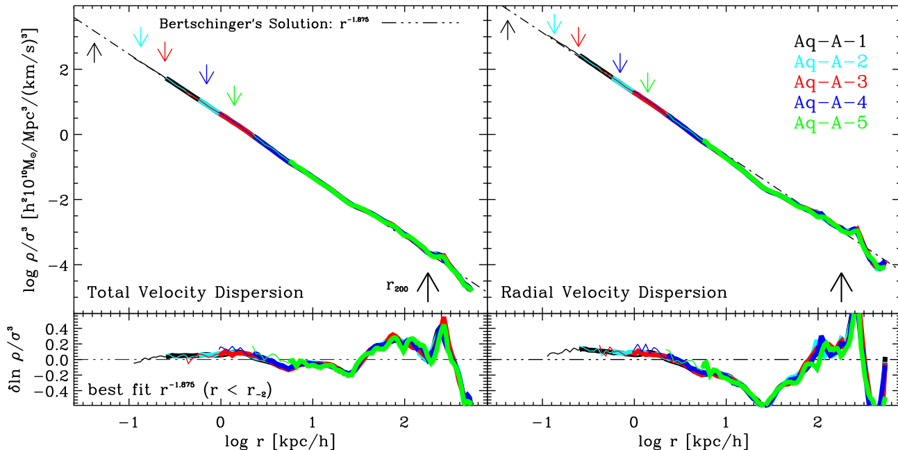
Figure 12. Pseudo-phase-space density profiles for our Aq-A convergence series, estimated as \rho/\sigma^3 , computed in concentric spherical shells. Arrows, line-types, and colours are as in Fig. 1. Note the remarkable power-law behaviour of this quantity, a result already noted by Taylor & Navarro (2001). The dot-dashed line is not a fit to the data, but rather the prediction of the similarity solution of Bertschinger (1985) for infall onto a point mass in an otherwise unperturbed Einstein-de Sitter universe, \rho/\sigma^3 \propto r^{-1.875} . This has been scaled to match Aq-A at r < r_{-2} . Residuals from the Bertschinger solution are shown in the bottom panels. Note that this power-law behaviour is most evident when the full 3D velocity dispersion is used (left panels). When only the radial velocity dispersion is used (right panels) deviations from the Bertschinger solution are considerably larger.
