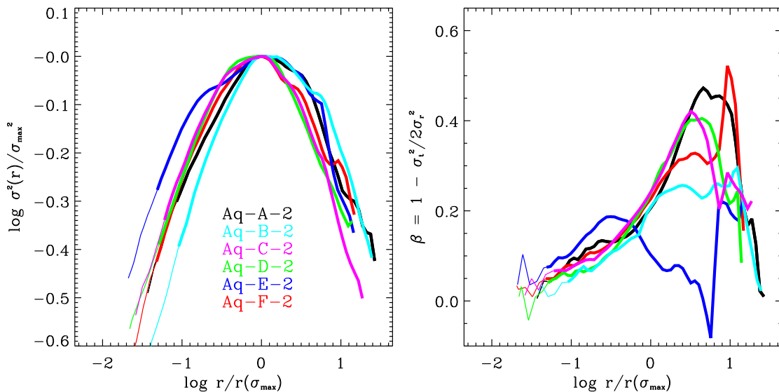
Figure 10. As Fig. 9, but for all six level-2 resolution Aquarius halos, scaled to match at the peak of the profile, identified by \sigma_{\max} and r(\sigma_{\max}) . This scaling highlights small but significant departures from similarity in the velocity dispersion structure of \Lambda CDM halos. Note the correspondence in shape between the velocity dispersion and r^2\rho profiles shown in Fig. 1, which reflects the “universal” pseudo-phase-space density profile of the halos (Fig. 13). Note also that the non-monotonic behaviour of the anisotropy highlighted in Fig. 9 is common to all six halos.
