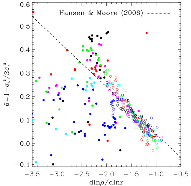
Figure 11. Local values of the logarithmic slope of the density profile plotted versus velocity anisotropy. The relation proposed by Hansen & Moore (2006) is shown as a dashed line. Because the density profile steepens gradually from the centre outwards whereas the velocity anisotropy is non-monotonic, no simple relation between these two quantities is valid throughout the halos. The Hansen & Moore formula approximates our results quite well in the inner regions, but large deviations may be seen outside r_{-2} , particularly at the largest radii where our halos are approximately isotropic but their density profiles are steepest. Open circles correspond to r_{\text{conv}}^{(1)} < r < r_{-2} , filled circles to r_{-2} < r < r_{200} . Colors are as in Fig. 3.
