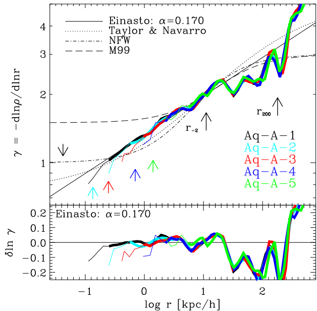
Figure 5. Logarithmic slope of the density profile as a function of radius for our Aq-A convergence series. As in other plots, thick lines show results for r > r_{\text{conv}}^{(7)} , thin lines extend the profiles down to the less strict convergence radius r_{\text{conv}}^{(1)} . Comparison shows that excellent numerical convergence for the slope is achieved down to a radius intermediate between these two convergence radii. Applied to the highest-resolution Aq-A-1 simulation, this implies that the slope is shallower than the asymptotic value of the NFW profile ( r^{-1} ) in the inner regions. We see no sign of convergence to an asymptotic inner power-law. Instead, the profiles get shallower toward the centre as predicted by the Einasto formula (a straight line in this plot). The “critical solution” of Taylor & Navarro (2001) (which has a r^{-0.75} asymptotic inner cusp) does better than NFW but not as well as Einasto in reproducing the inner profile of the halo.
