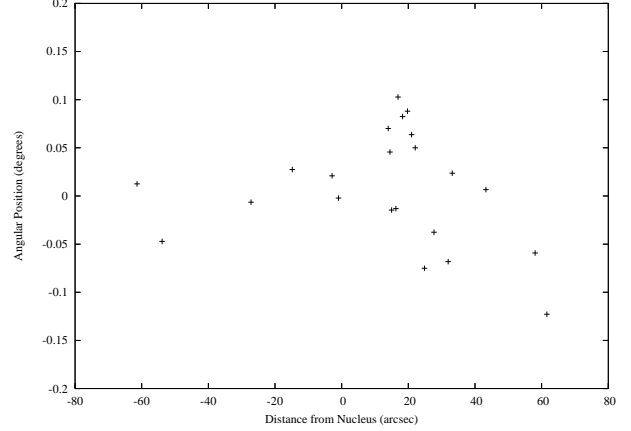
FIG. 3.— The offset between the position angle of the jet in Cen A ( 54^\circ ) and the transverse position of the radio knots as a function of the projected distance from the nucleus for the knots in the jet and counterjet (negative distances). The knots do not appear to lie at the PA 54^\circ for the entire length of the jet.
