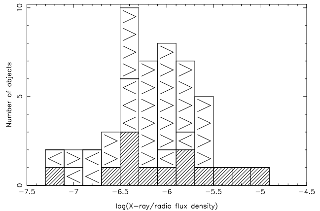
FIG. 9.— A histogram of the X-ray/radio flux density ratios for the paired knots (hashed region), the lower limits on the X-ray/radio flux density ratio for the X-ray-only knots ( > ), and the upper limits on the X-ray/radio flux density ratio for the radio-only knots ( < ) in Cen A.
