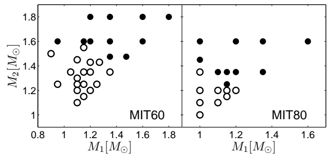
FIG. 1: Computed models for MIT60 and MIT80 in the M_1 - M_2 -plane of the gravitational masses of the SS binaries. Filled circles denote prompt collapse to a BH, while open circles indicate the formation of a HMO.
