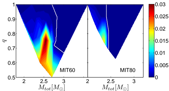
FIG. 2: Ejected mass per merger event, color-coded and measured in M_{\odot} , as function of the mass ratio q = M_1/M_2 and the total system mass M_{tot} = M_1 + M_2 of the binary configurations for the MIT60 and MIT80 EoSs. The white line separates binary mergers with and without ejecta.
