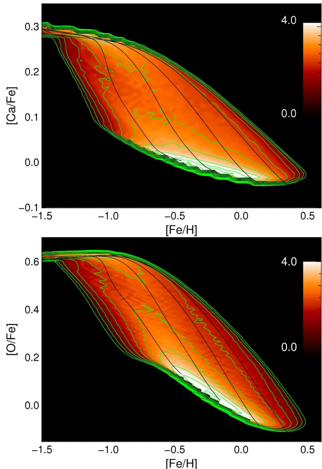
Figure 3. Logarithmic stellar densities for a simulated GCS stellar sample in the ([Ca/Fe], [Fe/H]) (top) and ([O/Fe], [Fe/H]) planes. Contours have a 0.5 dex spacing. Black lines track the development of the cold ISM in annuli of radii of (from right to left) 2.5, 5.0, 7.5 and 10 kpc.
