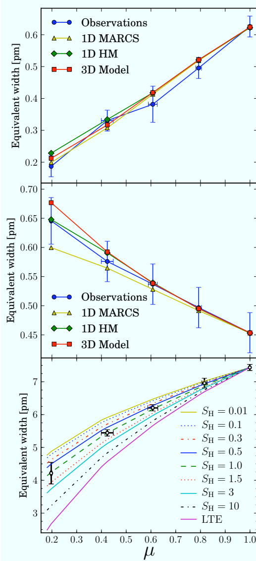
Fig. 1. Centre-to-limb variation of the oxygen lines. Top: O I 615.81 nm line (including blends). Middle: [O I] 630.03 nm line (including blends). Bottom: O I 777.41 nm line, only for the 3D model and for different scalings of the H I collisions.
