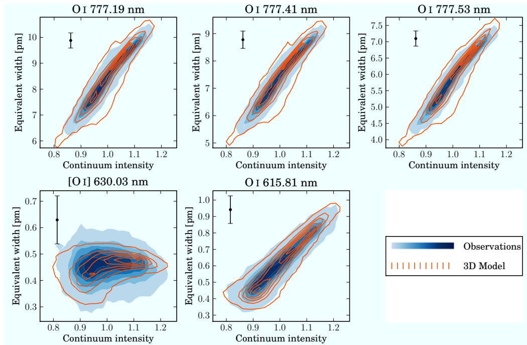
Fig. 2. Distribution of equivalent widths over the solar granulation at disk-centre, for five oxygen lines. The 3D model results have been degraded to account for the atmospheric turbulence and the telescope’s resolution. For each spatially-resolved spectrum the equivalent width has been computed and the resulting histogram of points is represented by the contours, as a function of the normalized local continuum intensity. The line profiles of the O I 777 nm lines were computed in NLTE, for S_H = 1 . For the other two lines LTE was assumed.
