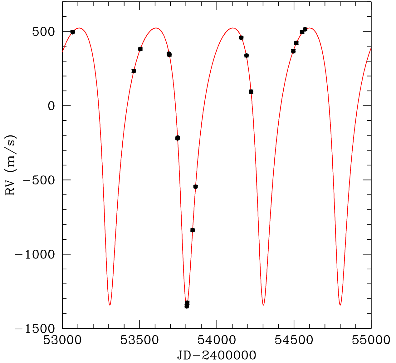
Fig. 1.— Keplerian orbital solution for HD 91669. The residual rms about this fit is 6.3 \text{ m s}^{-1} .
