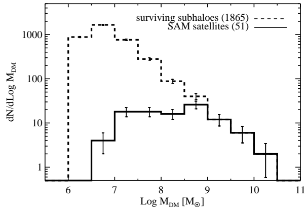
Figure 1. The solid histogram shows the present-day mass function for the satellites in our model. Error bars show the corresponding 1\text{-}\sigma Poisson uncertainties. The dashed histogram shows the subhalo mass function, which steeply rises up to the resolution limit of our simulation.
