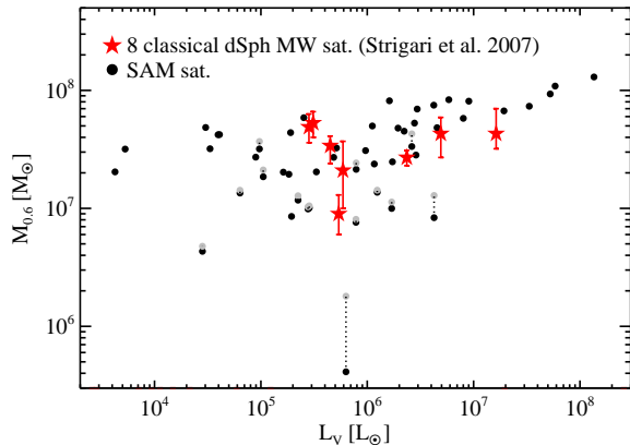
Figure 2. Mass within 600 pc as a function of the V-band luminosity for our model satellites (black and grey solid circles), and for the eight brightest dwarf spheroidal galaxies of the Milky Way (asterisks), where the Sagittarius dwarf has been excluded because it is clearly not in dynamical equilibrium. Black solid circles correspond to M_{0.6} measured via direct particle counting. For the model satellites which show clear signs of tidal disruption of the associated subhaloes, we also plot the Einasto M_{0.6} estimates shown with grey symbols.
