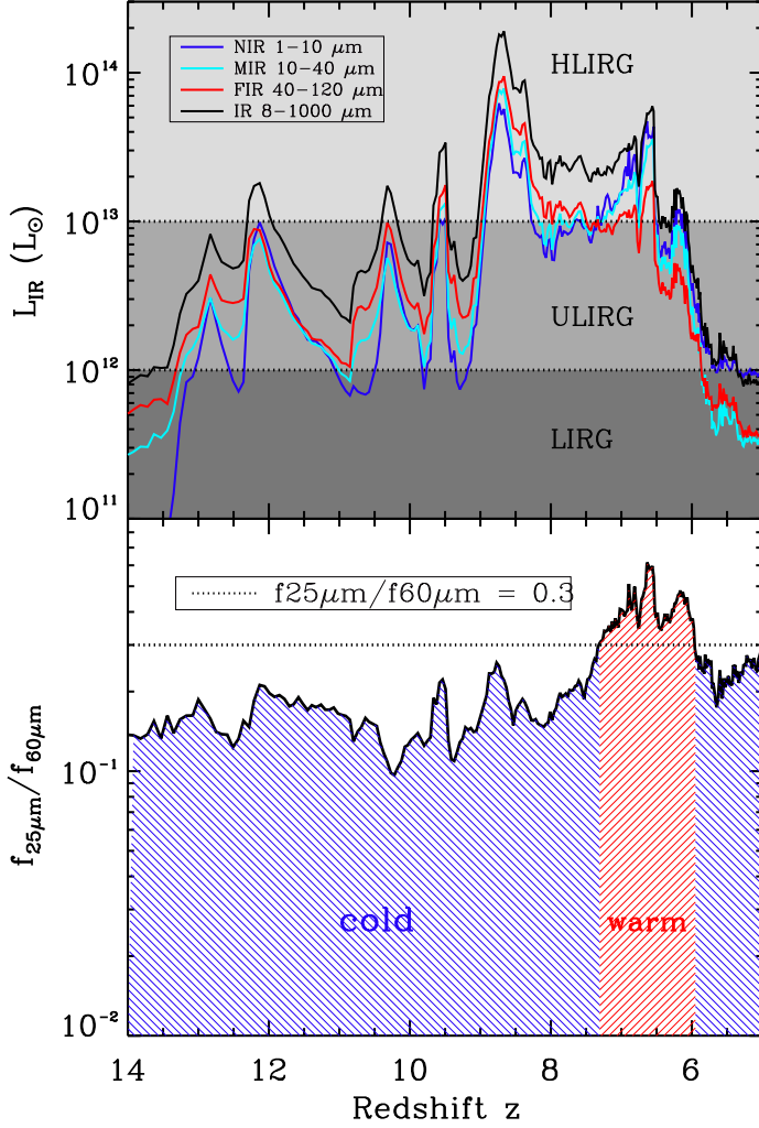
FIG. 17. — Evolution of rest-frame infrared luminosities of the quasar system (top panel) and the rest-frame color f_{25\mu\text{m}}/f_{60\mu\text{m}} (bottom panel). In the top panel, the solid curves represent the luminosity in near-IR ( 1-10\mu\text{m} ), mid-IR ( 10-40\mu\text{m} ), far-IR ( 40-120\mu\text{m} ), and IR ( 8-1000\mu\text{m} ), respectively. The grey shades indicate regimes for LIRG ( L_{\text{IR}} > 10^{11} L_{\odot} ), ULIRG ( L_{\text{IR}} > 10^{12} L_{\odot} ), and HLIRG ( L_{\text{IR}} > 10^{13} L_{\odot} ), respectively, as classified by Sanders & Mirabel (1996). The ratio f_{25\mu\text{m}}/f_{60\mu\text{m}} in the bottom panel is an indicator of the coldness of the SED with a critical value of 0.3 (Sanders & Mirabel 1996). The quasar system in our model evolves from “cold” ULIRG ( f_{25\mu\text{m}}/f_{60\mu\text{m}} < 0.3 ) to “warm” ULIRG (including HLIRG, f_{25\mu\text{m}}/f_{60\mu\text{m}} \geq 0.3 ) as it transforms from starburst to quasar phases.
