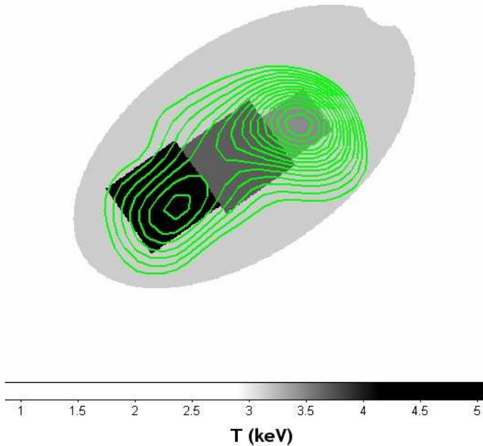
Fig. 9. The temperature map of the cluster. Overlaid are the contours of the X-ray surface map. The circle represents the region where a subpart of the cluster is visible in the raw and smoothed images (see Figs. 3 and 5). This area was excluded from the spectral analysis.
