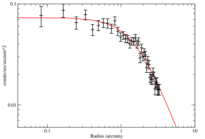
Fig. 7. The surface brightness profile around the NW peak (the X-ray brightest). The profile declines rapidly outside \sim 2 arcmin, a feature most likely caused by a shock due to a merger (see Sect. 5.1).
