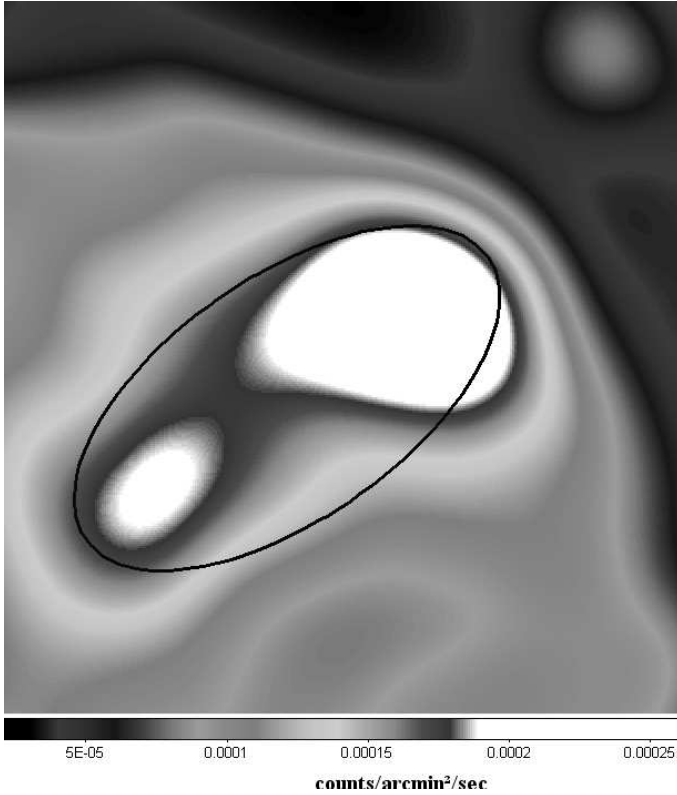
Fig. 5. A smoothed image of the whole cluster. This image is corrected for vignetting and smoothed with an adaptive smoothstyle with a signal to noise ratio of 40. It shows two subclumps and the overall elongated shape of the cluster. The size of the box is about 25 arcmin ( \sim 2.05 Mpc). The elliptical region indicates the area where we extracted a spectrum for the whole cluster.
