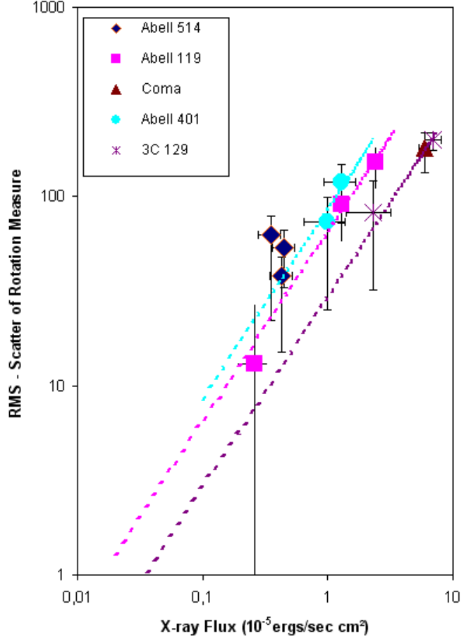
Fig. 13. The X-ray flux - \sigma_{RM} relation with the new data points for Abell 514. The new values are in good agreement with the general slope of the relation
