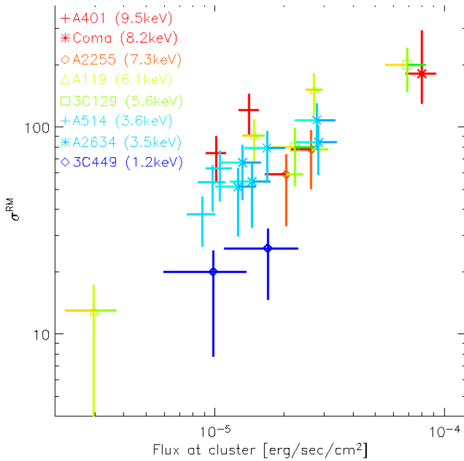
Fig. 1. The scatter of the root mean square of the Faraday Rotation measure (RMS) against the X-ray flux of a sample of clusters, for which both measurements are available.
