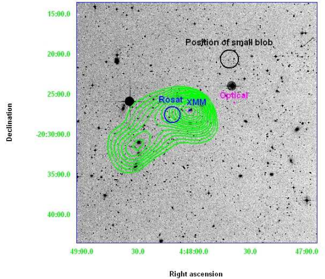
Fig. 4. The optical image overlaid with the X-ray contours. The two main X-ray clumps correspond well with the distribution of the galaxies, especially the area around the most X-ray bright emission shows the highest density in galaxies.
