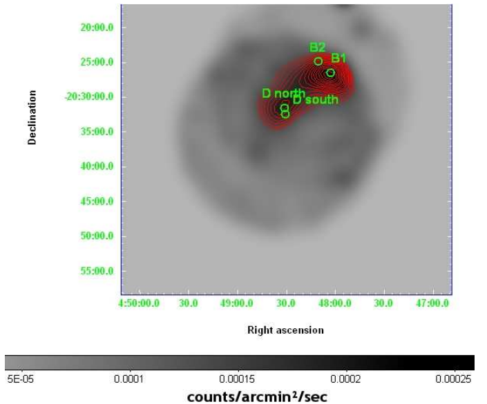
Fig. 2. The location of three of the radio sources within the cluster Abell 514 (D north and D south are measurements from the same source, but in two slightly offset positions). The other three radio sources lie outside the field of view of this X-ray observation.
