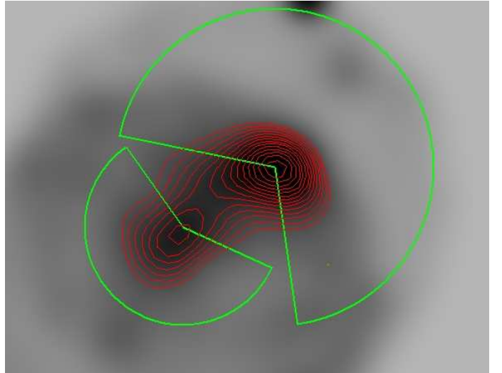
Fig. 6. The image shows the regions considered for deriving the surface brightness profiles around the NW and SE peaks. Each area was divided in different annuli and the
