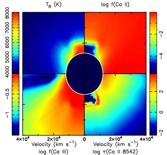
FIG. 3.— Upper left : Computed temperature structure in the atmosphere of model A20 at 30 days after the explosion. Upper right, lower left : Ionization fractions of Ca II and Ca III. Lower right : Sobolev optical depth of Ca II \lambda 8542 .
