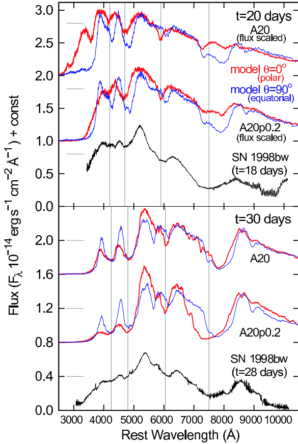
FIG. 4.— The spectra computed with model A20 and A20p0.2 compared with the spectra of SN 1998bw. The synthetic spectra are reddened with E(B-V) = 0.032 and scaled assuming \mu = 32.76 . Upper: Synthetic spectra at 20 days after the explosion (shifted upward by 2.0 and 1.0 \times 10^{-14} , respectively) and the spectrum of SN 1998bw 18 days after GRB 980425. The flux is reduced by a factor of 1.25 after the computation. The vertical lines are drawn at 4200 , 4700 , 5900 and 7500 Å. The horizontal lines show the same flux level ( 8.0 \times 10^{-15} ). Lower: Synthetic spectra at 30 days after the explosion (shifted upward by 1.6 and 0.8 \times 10^{-14} , respectively) and SN 1998bw 28 days after GRB 980425. The vertical lines are drawn at 4250 , 4800 , 6050 and 7500 Å. The horizontal lines show the same flux level ( 4.0 \times 10^{-15} ).
