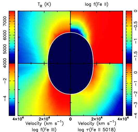
FIG. 1.— Upper left : Computed temperature structure in the atmosphere of model A20 at 20 days after the explosion. Upper right, lower left : Ionization fractions of Fe II and Fe III. Lower right : Sobolev optical depth of the Fe II \lambda 5018 . The vertical axis ( z -axis) is the jet direction.
