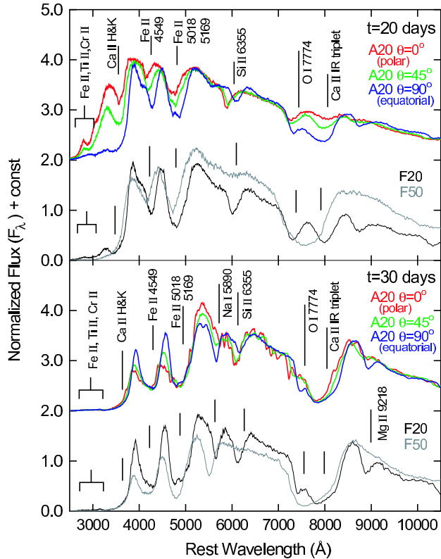
FIG. 2.— Upper : Synthetic spectra of model A20, F20 (black) and F50 (gray) at 20 days after the explosion. The red, green and blue lines show the spectra of model A20 seen from \theta = 0^\circ , 45^\circ and 90^\circ , respectively. Here \theta is measured from the z-axis (jet direction). Lower : Same as upper panel but at 30 days after the explosion.
