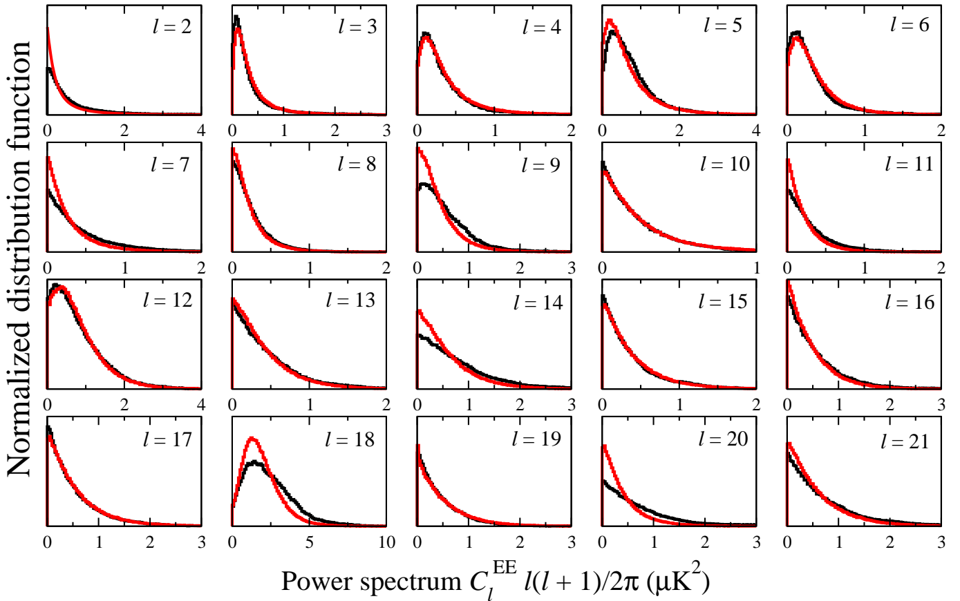
FIG. 1.— Comparison of single- l EE marginal posteriors from the WMAP code (black distributions) and the Gibbs sampler (red distributions) using the QV map. The EB and BB power spectra are held at zero.
