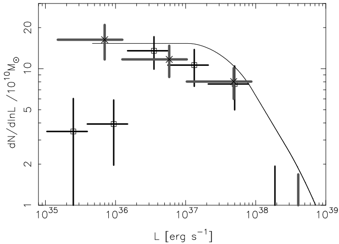
Fig. 8. The LF of sources with a radial distance of 1'-9' from the centre of M31, excluding sources in GCs and GC candidates (crosses, 130 sources), compared to the LF of sources from the inner 1' and sources in confirmed GCs (squares, 40 sources). The normalization of the latter is arbitrary. The solid line is the average LMXB LF, with the same normalization in figures 5-10.
