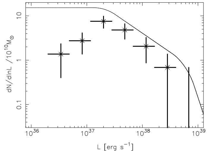
Fig. 10. The LF of the maximum luminosity of the transients observed (28 sources). Note, that below \sim 10^{37} \text{erg/s} it is subject to strong selection effects. The solid line is the average LMXB LF, with the same normalization as in figures 5-10.
