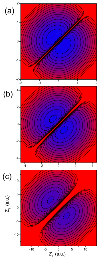
FIG. 3: Two-dimensional contour plot of the sum of the Gaussian and of the electron repulsion potentials for \omega_z = 5.0 (a), 1.0 (b), and 0.1 (c). The anharmonicity parameter for the Gaussian potential and the maximum potential height displayed are 0.05 and \omega_z \times 10 , respectively, for all cases. The diagonal line separating the contours into two regions represents the potential wall of the electron repulsion potential.
