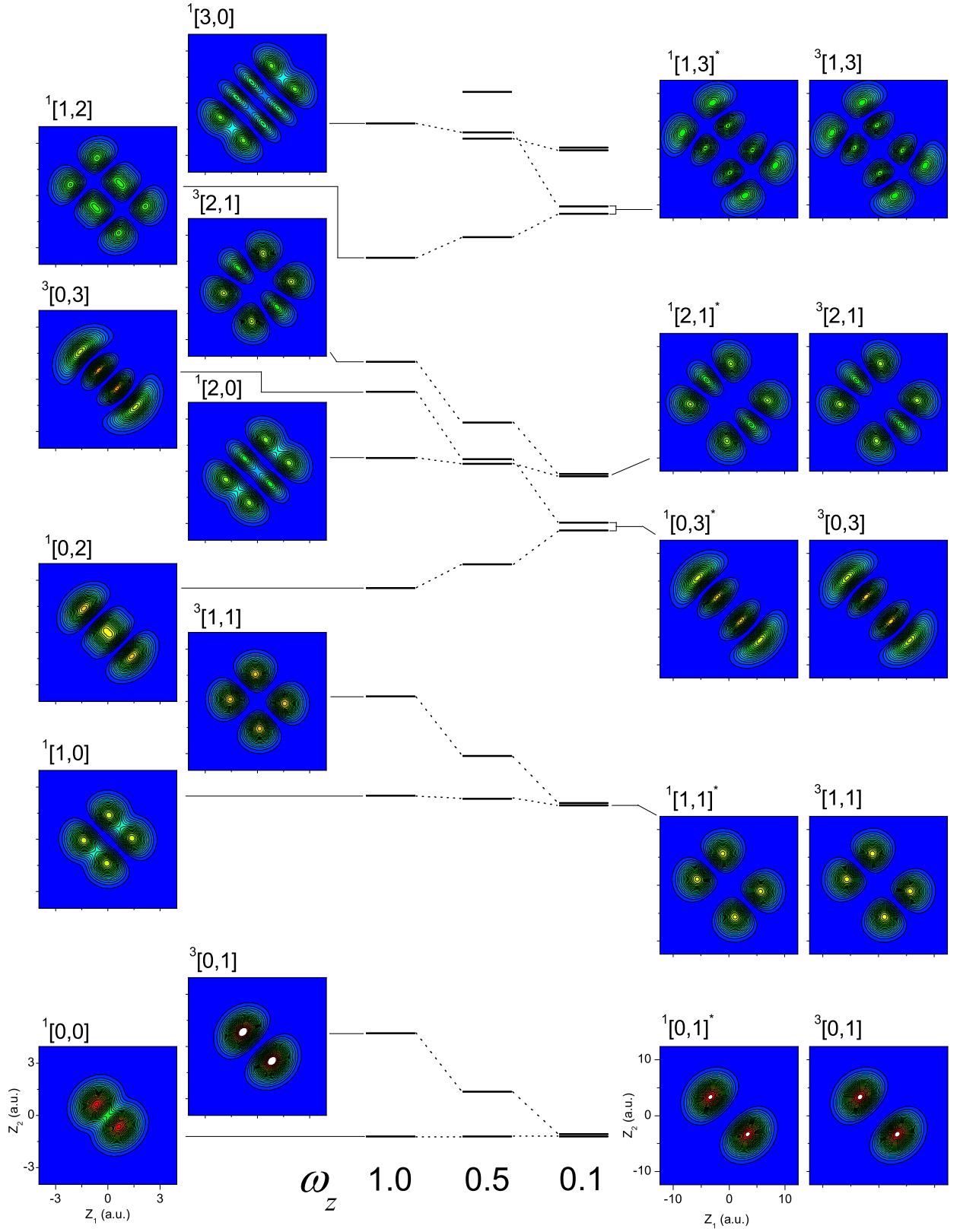
FIG. 2: Correspondence of the low-lying energy levels and wave functions of two electrons confined in a quasi-one-dimensional Gaussian potential. The anharmonicity parameter \alpha of the Gaussian potential is 0.05 for all cases. The vertical axis of each of the three energy diagrams is scaled by \omega_z so that the excitation energy of one quantum of \omega_z are on the same level. The electronic wave functions are plotted as square density in the two electron coordinates z_1 and z_2 . The assignment of wave functions has been made by counting the number of nodal lines along the symmetric and antisymmetric electron coordinates for \omega_z = 1.0 while an extended assignment marked by an asterisk has been made for the singlet wave functions with \omega_z = 0.1 (see text).
