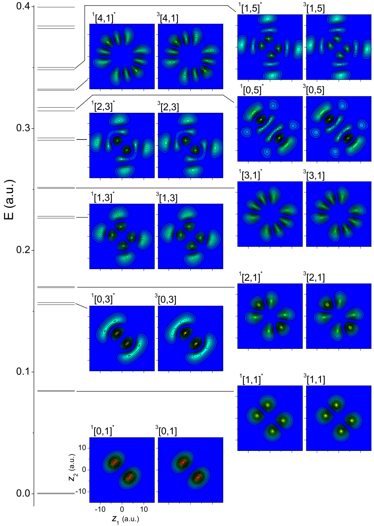
FIG. 6: Square density plot of the wavefunctions for the low-lying states of two electrons confined in a quasi-one-dimensional Gaussian potential with (D, \omega_z) = (0.8, 0.1) . The assignment of wave functions has been made by counting the number of nodal lines along the symmetric and antisymmetric electron coordinates. The assignment marked by an asterisk given to the singlet wave functions is the extended assignment (see text).
