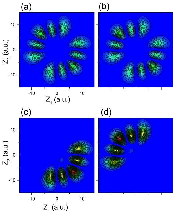
FIG. 8: Square-density plot of the wavefunctions for the doublet pair ^1[4,1]^* (a) and ^3[4,1] (b), and their sum (c) and difference (d).
