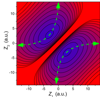
FIG. 9: Two-dimensional contour plot of the sum of the Gaussian and of the electron-repulsion potentials for (D, \omega) = (0.8, 0.1) . The maximum potential height displayed and the domain of the coordinates z_1 and z_2 are the same as in Fig. 3(c). The dotted allows represent the valleys of the potential.
