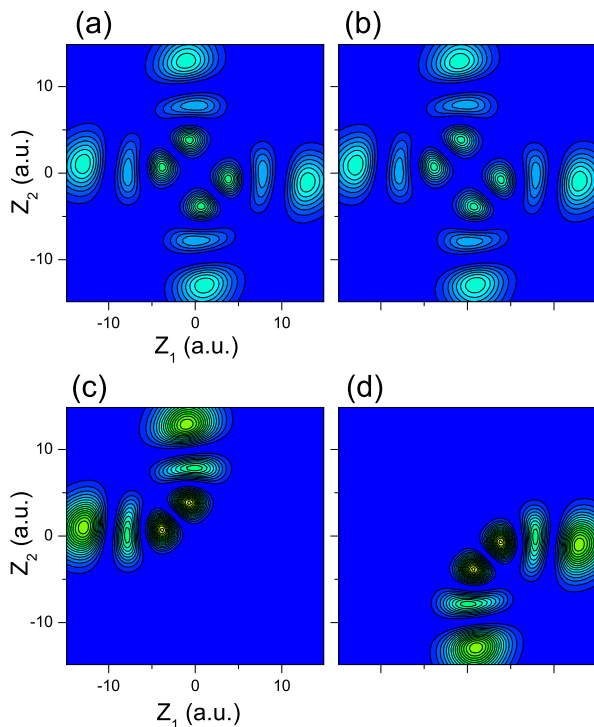
FIG. 7: Square-density plot of the wavefunctions for the doublet pair ^1[1,5]^* (a) and ^3[1,5] (b), and their sum (c) and difference (d).
