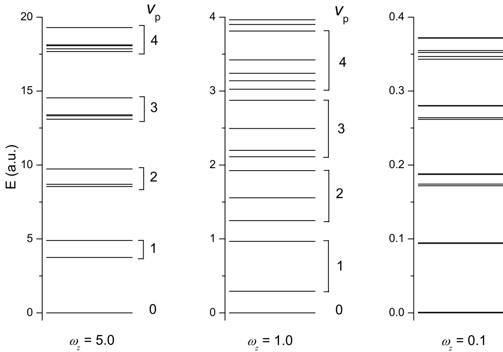
FIG. 1: Energy spectrum of two electrons confined by a quasi-one-dimensional Gaussian potential with different strength of confinement \omega_z represented as relative energies from the ground state. The anharmonicity parameter \alpha of the Gaussian potential is 0.05 for all cases. The vertical axis of each of the three energy diagrams is scaled by \omega_z so that the energy of the ground state and the excitation energy of 4 quanta of \omega_z are at the same level of the vertical axis, respectively.
