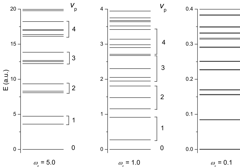
FIG. 5: Excitation energy spectrum of two electrons confined in a quasi-one-dimensional Gaussian potential with different strength of confinement \omega_z . The anharmonicity of the Gaussian potential \alpha is 0.125 for all cases. The vertical axis of each of the three energy diagrams is scaled by \omega_z so that the energy of the ground state and the excitation energy of 4 quanta of \omega_z are at the same level of the vertical axis, respectively.
