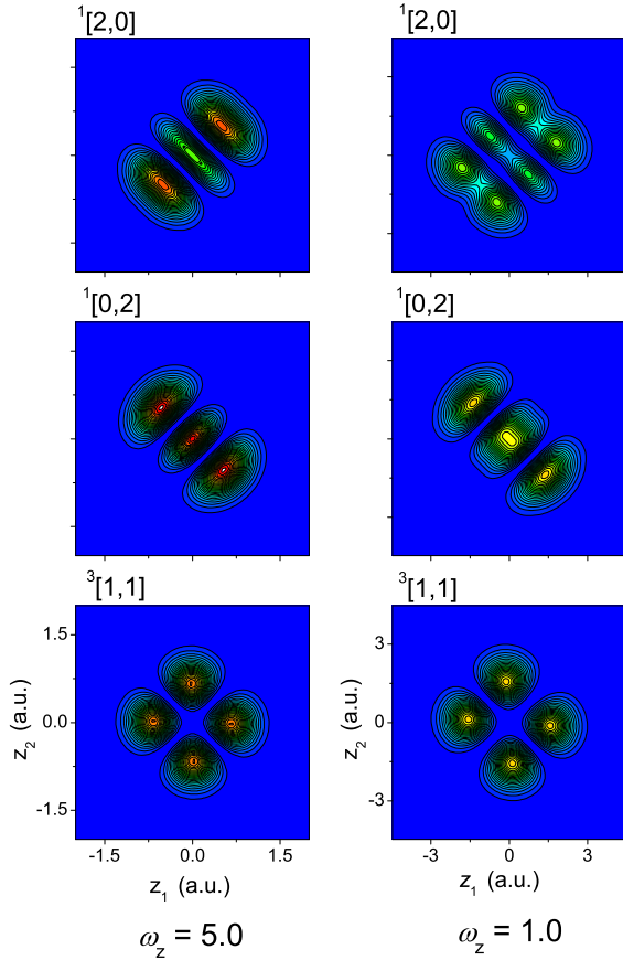
FIG. 4: Square density plot of the wave functions for the three states in the polyad manifold of v_p = 2 of two electrons confined in a quasi-one-dimensional Gaussian potential with \omega_z = 5.0 and 1.0 . The anharmonicity parameter \alpha of the Gaussian potential is 0.05 .
