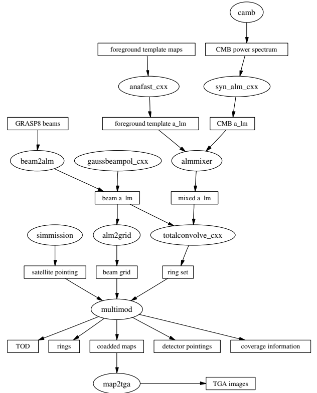
Fig. 1. Schematic data flow in a typical Planck simulation pipeline. Rectangular components denote parameters or data products (see Sect. 4), whereas elliptic shapes represent modules (see Sect. 6).
