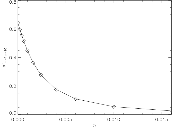
Fig. 13. Growth rate of the m = 1 , n = 20 mode in the velocity field as function of the magnetic diffusivity \eta . Unstratified case.
