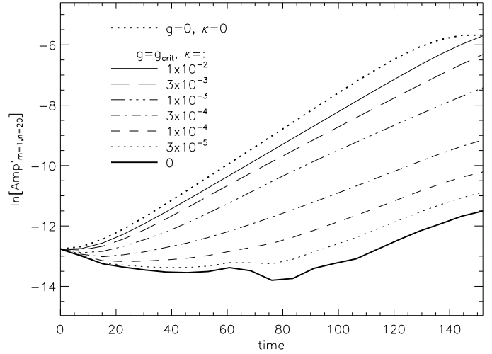
Fig. 15. Velocity field amplitudes of the m = 1 , n = 20 mode as a function of time, at different values of thermal diffusion \kappa , when g = 10/\pi . For large values of \kappa , the stabilising effect of gravity is absent and growth occurs at the same rate as in the adiabatic unstratified case (uppermost line).
