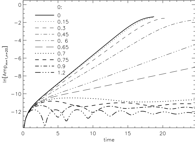
Fig. 12. Amplitudes of the m = 1 , n = 20 mode at different values of \Omega , taken from the displacement field. Adiabatic unstratified case. For values of \Omega of 0.7 and higher, an oscillatory behaviour is seen, indicating stability.
