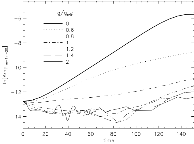
Fig. 14. Effect of the stabilising stratification, under adiabatic conditions ( \kappa = \eta = 0 ). Velocity field amplitudes of the m = 1 , n = 20 mode as a function of time for seven values of the acceleration of gravity g . The first half of the run with g = 2g_{\text{crit}} is plotted at higher time resolution.
