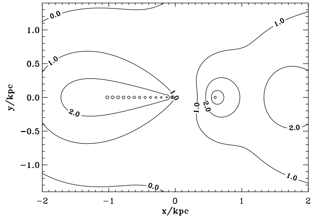
Fig. 6. Contour plot of the brightness temperature of the scattered radiation about twenty thousand years after the onset of the jet activity, i.e. the ejection of the first pair of blobs. About every 1000 years a further pair of blobs is being produced. The corresponding apparent distance between individual blobs is about 1 kpc for the approaching blobs on the right side of the nucleus and about 80 pc for the receding blobs on the left side of the nucleus.
