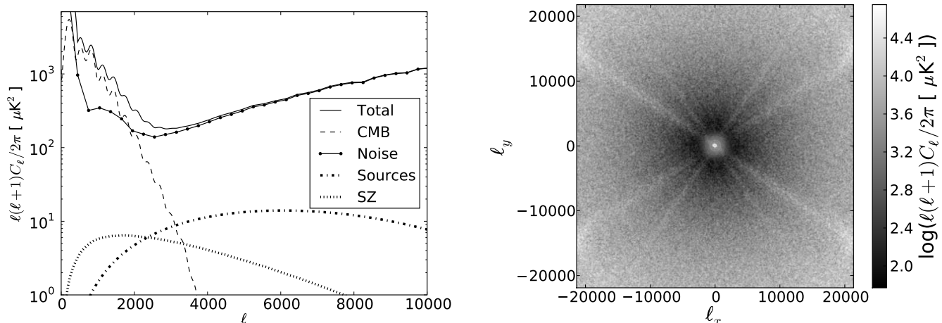
FIG. 2.— Model ACT auto-power spectra used for the matched filter. Left . One-dimensional spectra decomposed by component. The CMB spectrum is taken from WMAP5 (Nolta et al. 2009). The undetected sources and the Sunyaev-Zel’dovich effect from galaxy clusters are 1D templates fit to the high- \ell 148 GHz spectrum in Fowler et al. (2010). The 1D noise spectrum is obtained by radially-binning the average of 2D spectra from ACT 148 GHz jackknife maps. The spectra are dominated at low- \ell by the CMB and atmospheric noise and at high- \ell by white detector and photon shot noise. Convolution of all celestial components by the ACT beam results in attenuation of the corresponding spectra at high- \ell . Right . The model two-dimensional auto power spectrum. The spectrum includes noise, CMB, undetected sources and the Sunyaev-Zel’dovich effect from galaxy clusters. The latter three components were obtained from the 1D models. The ACT noise is isotropic except for extra noise in scan parallel (from residual 1/f) and scan perpendicular (from detector row correlations) directions. For each rising and setting scan direction, two orthogonal bands of excess power are centered on the origin rotated 60^\circ with respect to one another. To minimize contamination, it is important to deweight data in these diagonal modes through the two-dimensional matched filter.
