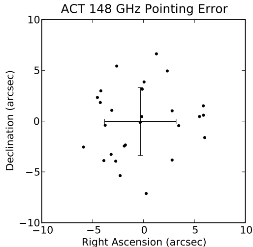
FIG. 4.— Astrometric Accuracy. The small filled circles are the positional offsets of ACT sources with \text{SNR} > 20 from counterparts in AT20G. The error bars show the rms in right ascension ( 3.5'' ) and declination ( 3.3'' ) and are centered on the mean of the distribution: -0.3'' \pm 0.7'' in right ascension and 0.0'' \pm 0.6'' in declination.
