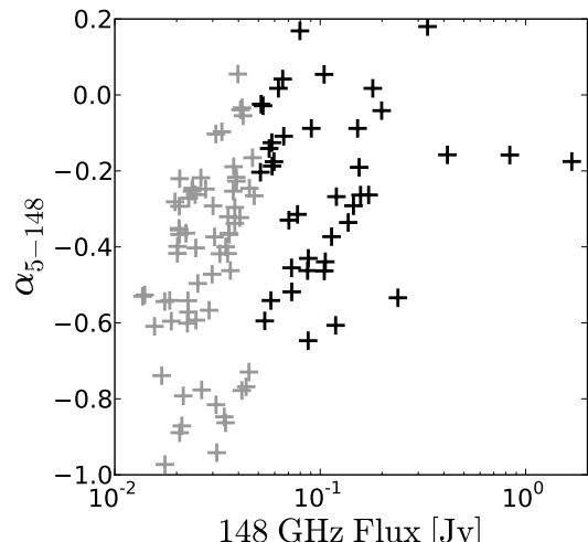
FIG. 9.— Radio color-magnitude diagram. As in Figure 8, the data are divided between high flux densities (black crosses) and low flux densities (gray crosses) at 50 mJy. The unbiased 50 mJy sample has a 5–148 GHz spectral index of \alpha_{5-148} = -0.20 \pm 0.21 (\pm 0.03) . The low flux density data suffer a selection bias that excludes sources with flat or rising spectra.
