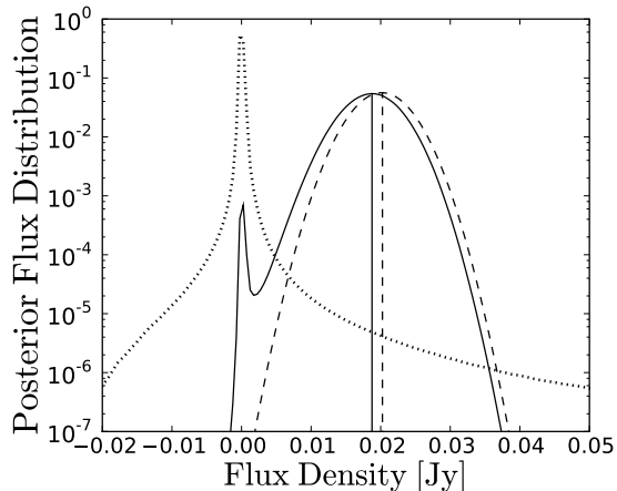
FIG. 6.— Flux density deboosting. The Gaussian flux density distribution P(S_m | S_0) (dashed) derived directly from the maps is multiplied by the prior distribution P(S_0) (dotted) of the intrinsic source flux to obtain the deboosted posterior flux distribution (solid). Since the mean of the maps is set to zero through filtering, P(S_0) can assume negative values. The peak in the distribution shifts to lower density flux (a <10\% effect for 20 mJy sources). For the SNR=5.6 source shown here, there is little volume in the posterior P(S_m | S_0) at negative flux.
