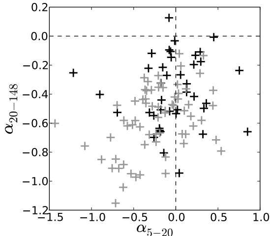
FIG. 8.— Radio source spectral indices. In this radio color-color diagram, 5–20 GHz and 20–148 GHz spectral indices are shown for ACT-AT20G cross-identified sources. The population is dominated by sources which are peaked (lower right quadrant) or falling (lower left quadrant). Black (Gray) crosses correspond to sources with 148 GHz flux density greater (less) than 50 mJy. The low flux sample is incomplete and suffers from selection bias that favors sources with more negative spectral indices.
