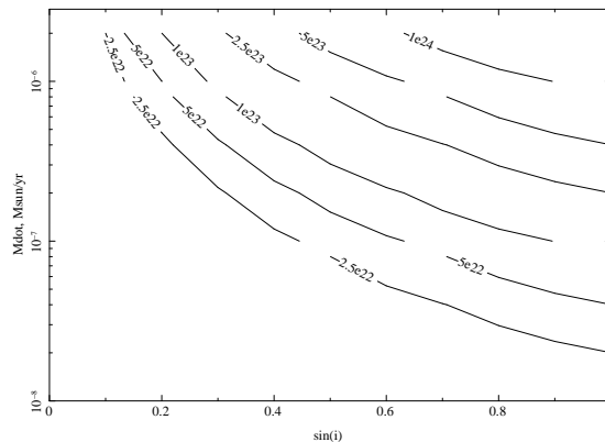
Fig. 5. Equivalent column for photoabsorption as a function of binary inclination and mass loss rate by the optical companion.
