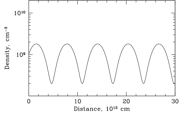
Fig. 9. Density profile of the medium at the initial time: n_0 = 10^9 + 8 \times 10^8 \sin r_{13} , where r_{13} is the radius in 10^{13} cm.
