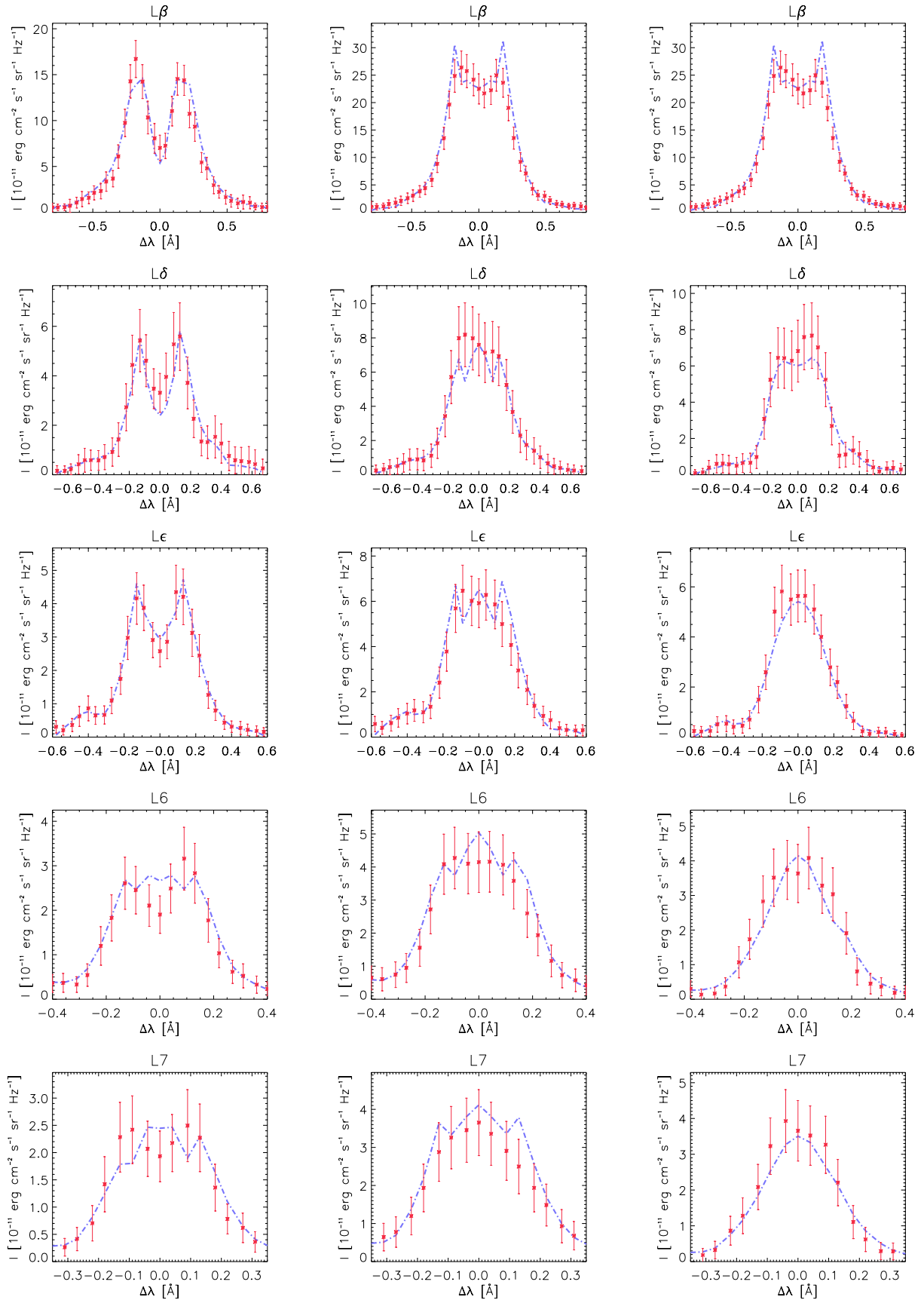
Fig. 9. Comparison of observed profiles from the sections Ha\text{-fil} , ext2 and ext6 (columns from left to right) with fitted synthetic profiles computed using the 1D-slab model. Observed intensities are plotted with points with errorbars and synthetic profiles with dot-dashed lines. Intensities are expressed in units 10^{-11} \text{ erg cm}^{-2} \text{ s}^{-1} \text{ sr}^{-1} \text{ Hz}^{-1} .
